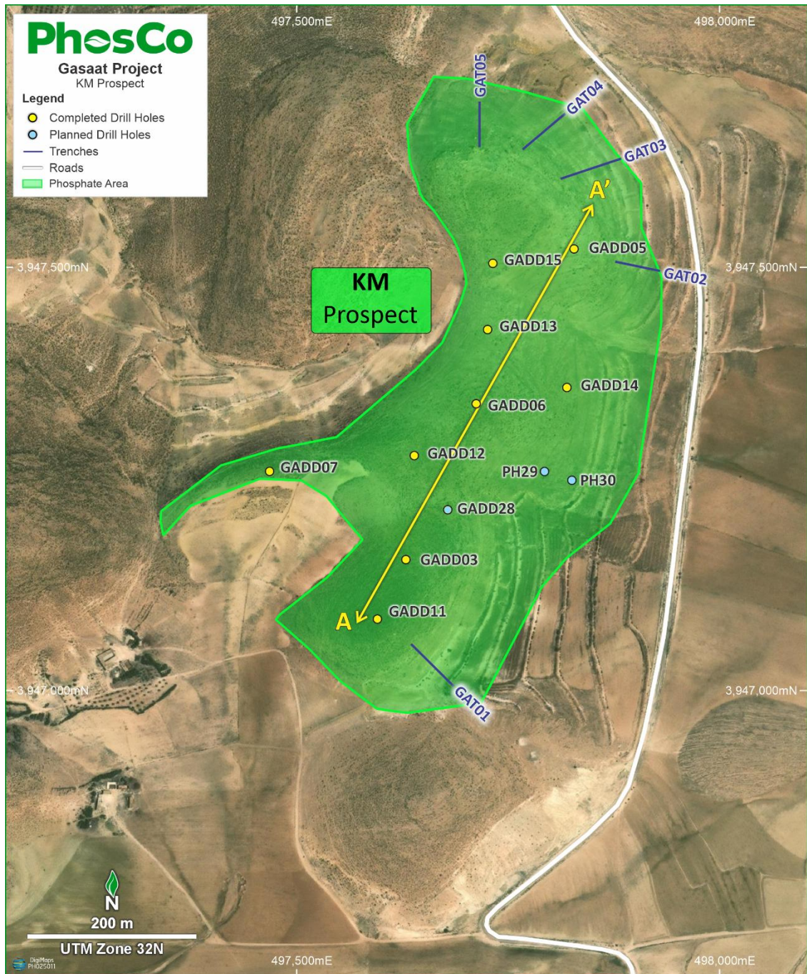
Figure 6 – KM Prospect showing location of trenches
