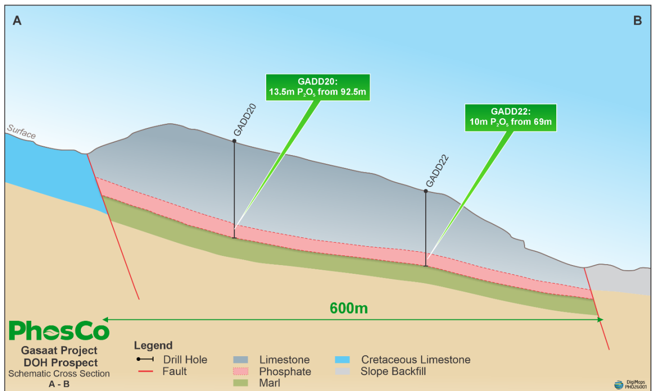
Figures 3 & 4 – DOH Cross Sections C-D and A-B showing generalised geology as determined from drilling, trenching and outcrop mapping
