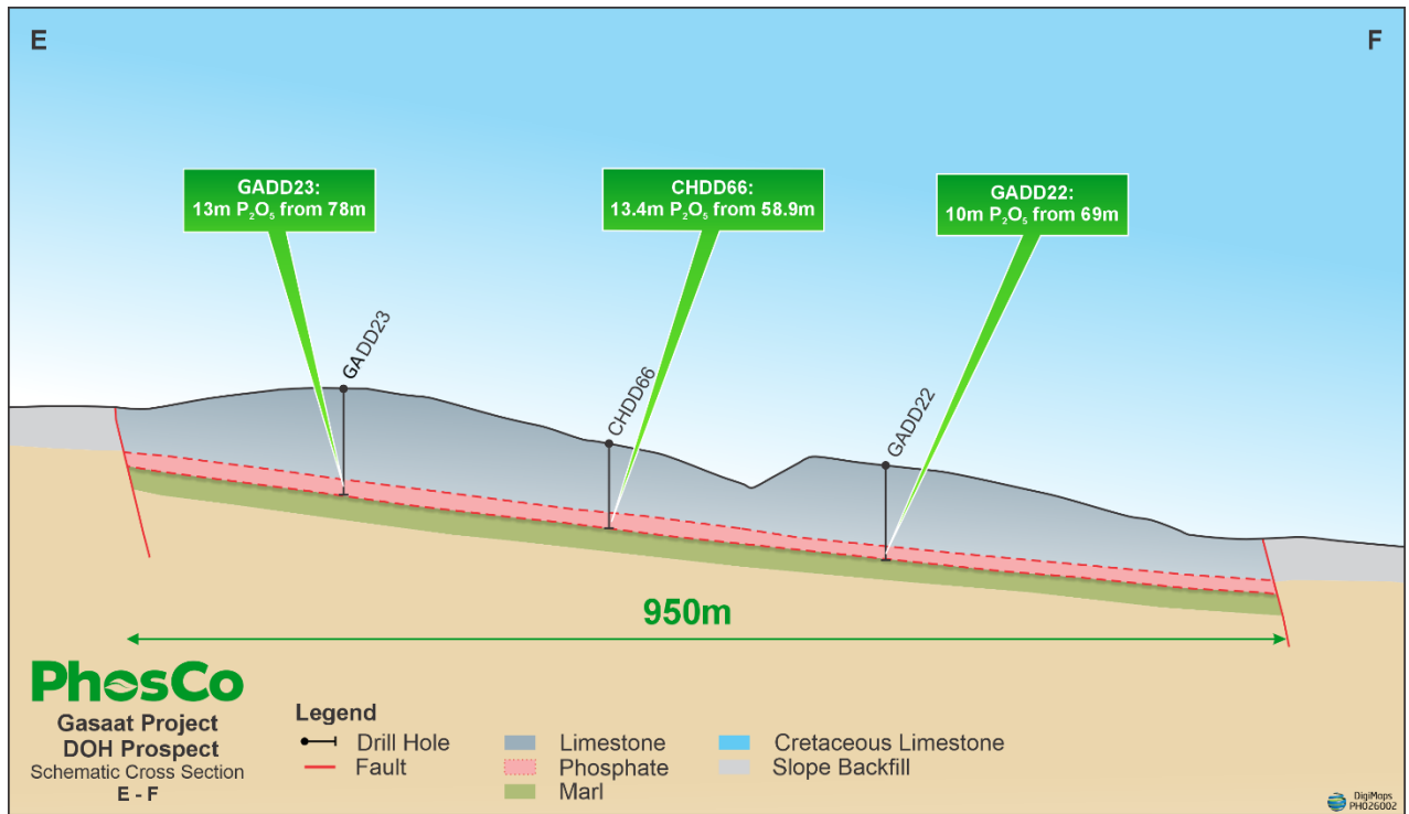
Figure 5 – DOH Long Section E-F showing generalised geology as determined from drilling, trenching and outcrop mapping
