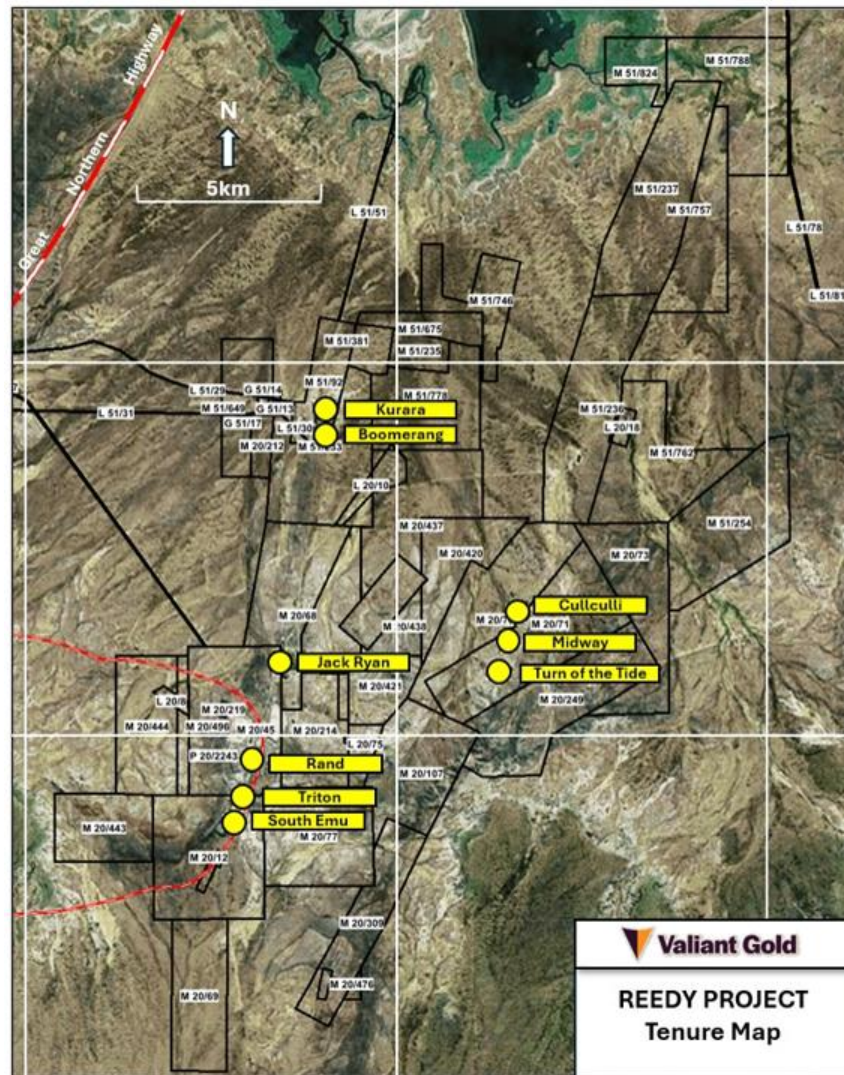
Figure 3.5 Reedy Project Tenure Map
