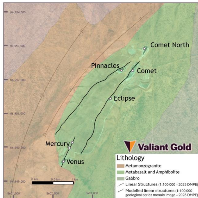
Figure 6.1 Location of Deposits within Comet Mining Area, Showing Major Lithological Units (Entech/Westgold 2025)
