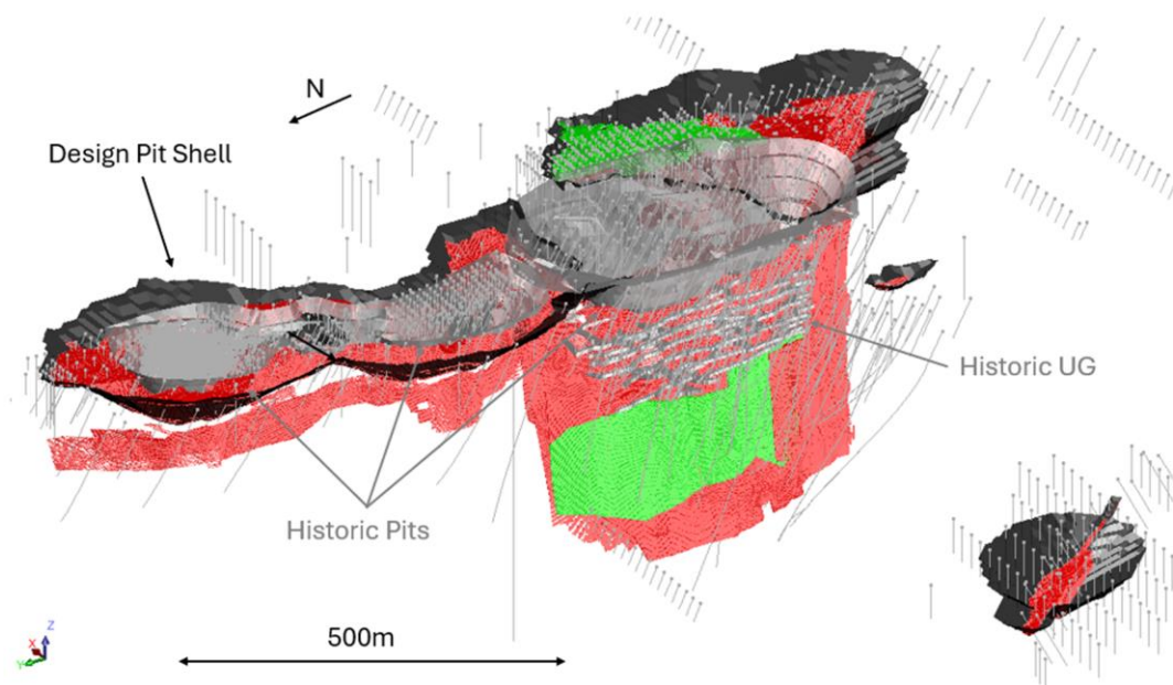
Figure 3 Reedy North (Boomerang – Kurara) classified and depleted MRE inventory – open pit in situ Resource inside A$5,000/oz pit shell. Indicated = green, Inferred = red.
