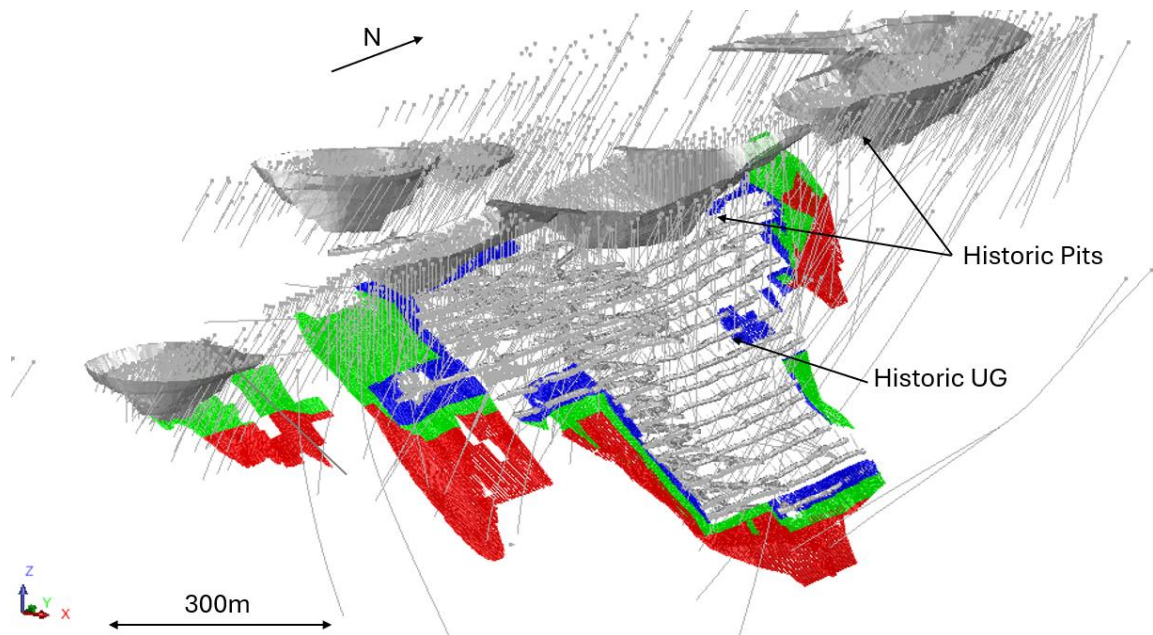
Figure 2 Comet classified and depleted MRE inventory – underground in situ Resource. Measured = blue, Indicated = green, Inferred = red.
