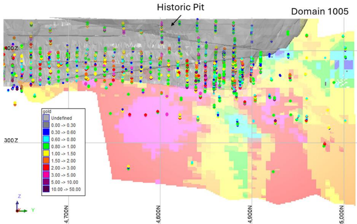
Figure 9.2 Long Section View, Looking West, at Comet North Block Model and Entech Composites (Entech 2025)
