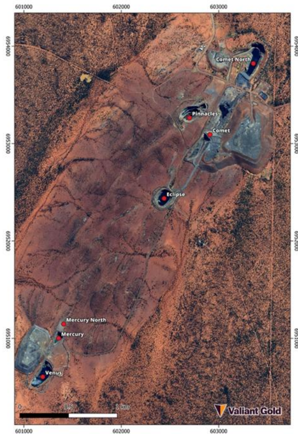
Figure 4.1 Satellite view of Comet Mining District (Entech 2025)
