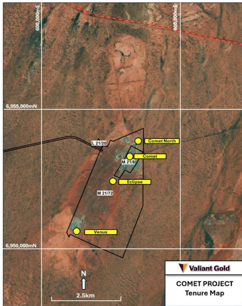
Figure 3.4 Comet Project Tenure Map
