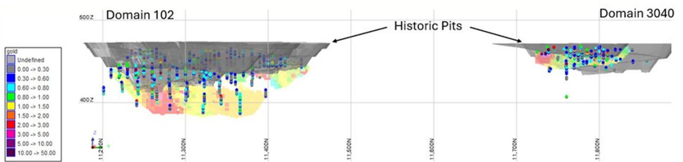
Figure 9.11 Long Section View, Looking West, of Culculli Block Model and Entech Composites (Entech 2025)
