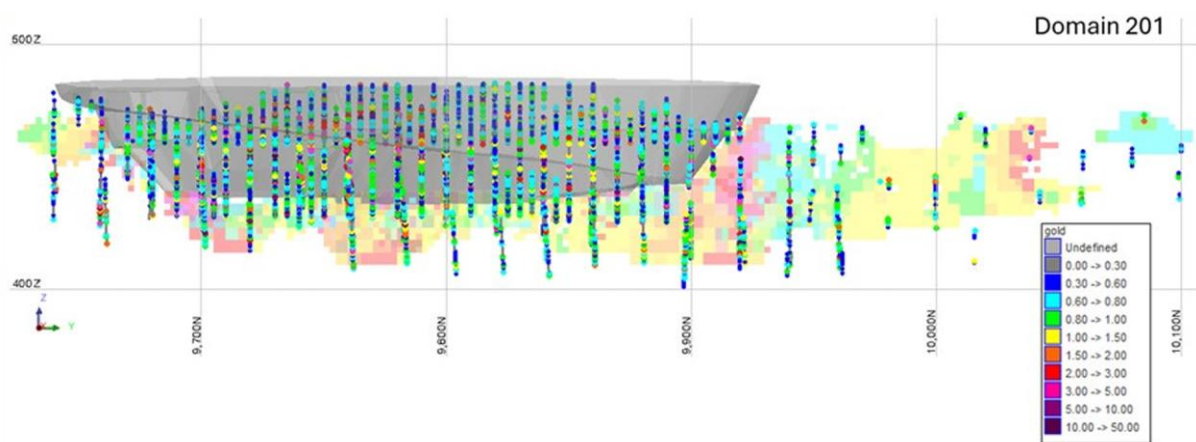
Figure 9.12 Long Section View, Looking West, of Turn of The Tide Block Model and Entech Composites (Entech 2025)
