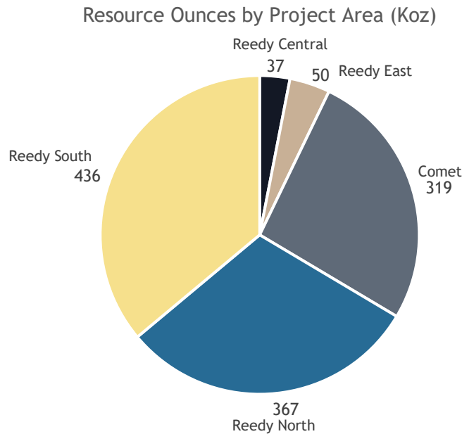
Figure 1.1 Resource Ounces by Project Area (Measured, Indicated and Inferred)
