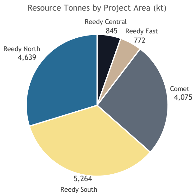
Figure 11.1 Resource Tonnes by Project Area (M+I+I)
