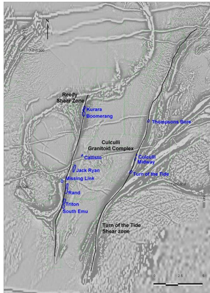
Figure 6.3 1st Vertical Derivative Magnetics at Reedy Highlighting Project Structural Corridors (Thebaud, 2008, Entech/Westgold 2005)
