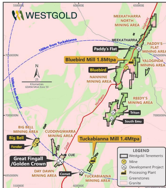
Figure 3.1 Westgold's Murchison Project Area (Westgold 2025)
