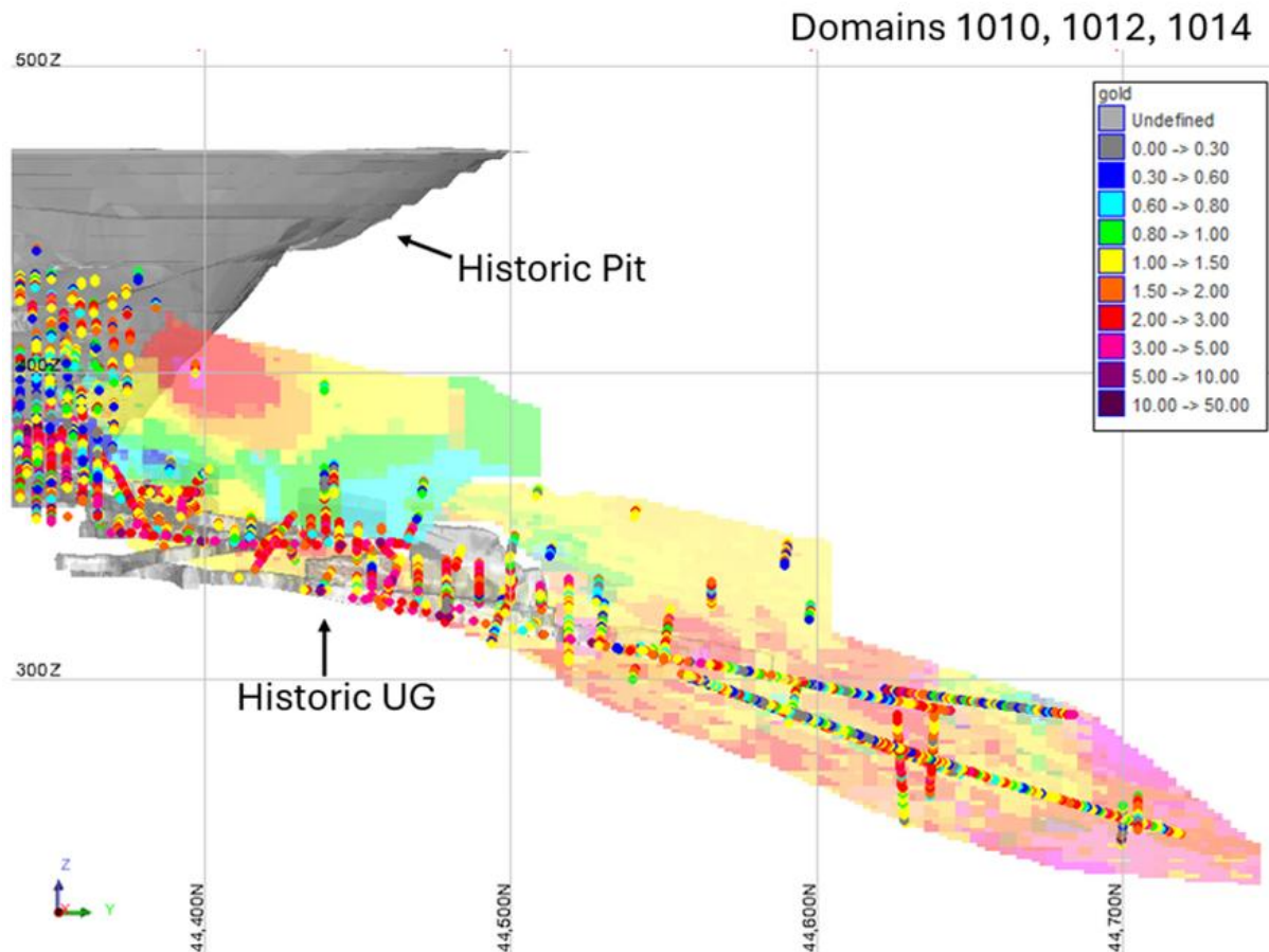
Figure 9.8 Long Section View, Looking West, of Jack Ryan Block Model and Entech Composites (Entech 2025)
