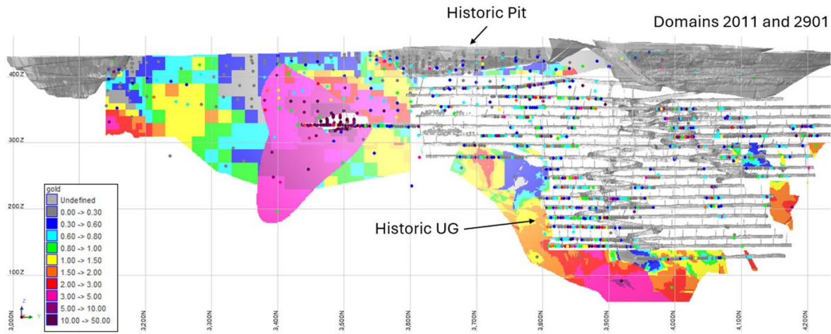
Figure 9.1 Long Section View, Looking West, of Comet Block Model and Entech Composites (Entech 2025)
