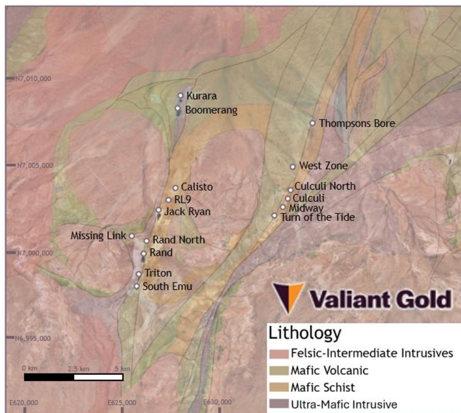
Figure 6.2 Location of Deposits within Reedy Mining Area, Showing Major Lithological Units (DMPE 2025)
