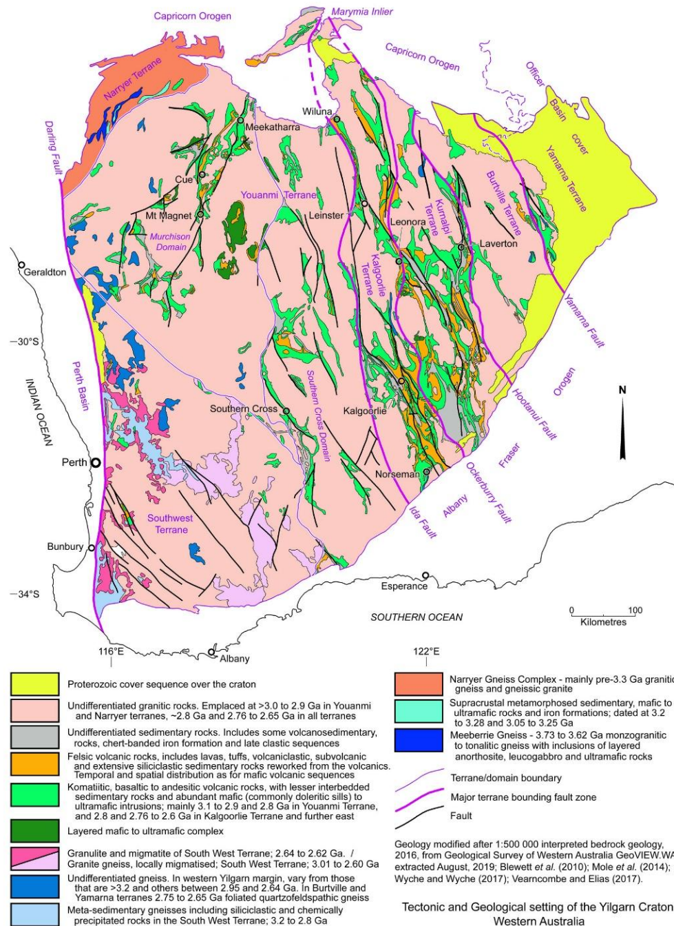
Figure 5.1 Tectonic and Geological Setting of Yilgarn Craton, WA (Porter GeoConsultancy 2019) 1
