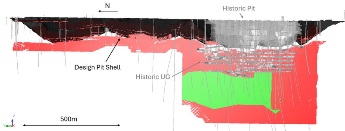
Figure 4 Reedy North (Boomerang – Kurara) classified and depleted MRE inventory – underground in situ Resource. Indicated = green, Inferred = red.
