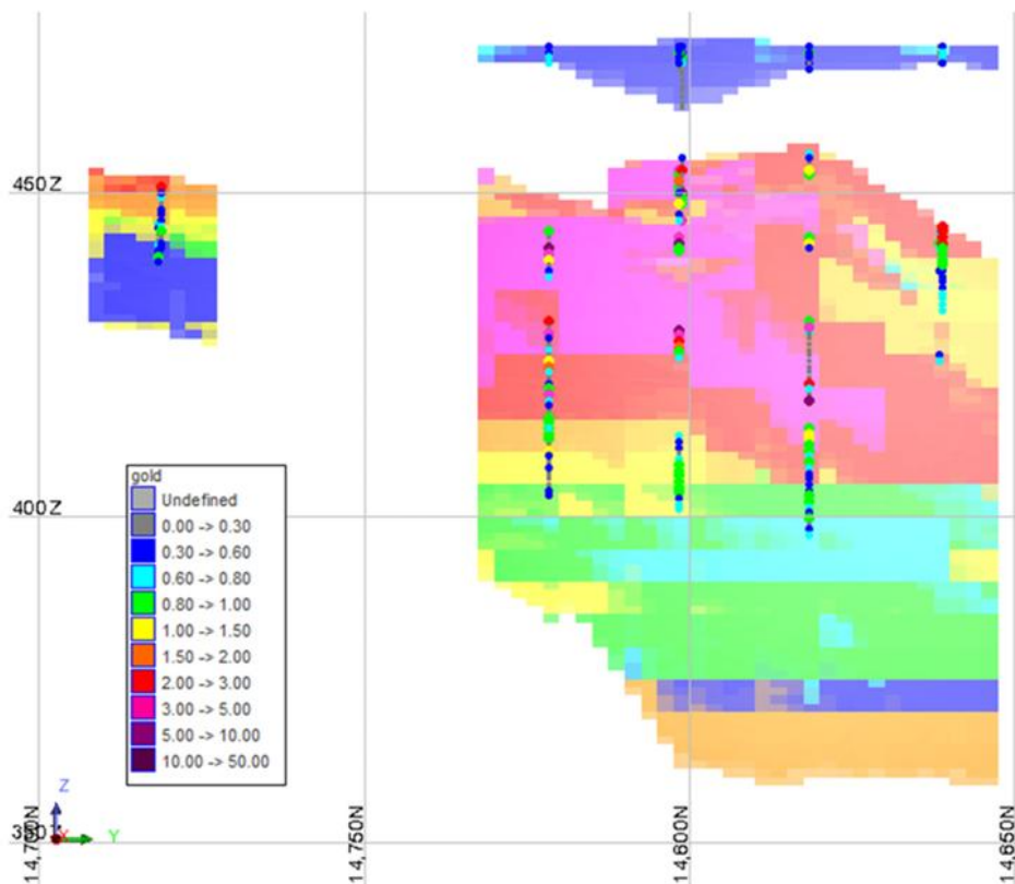
Figure 9.9 Long Section View, Looking West, of RL9 Block Model and Entech Composites (Entech 2025)
