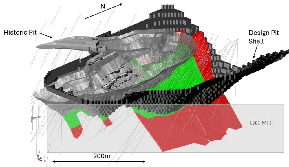
Figure 1 Comet North classified and depleted MRE inventory – open pit in situ Resource inside A$5,000/oz pit shell. Indicated = green, Inferred = red.
