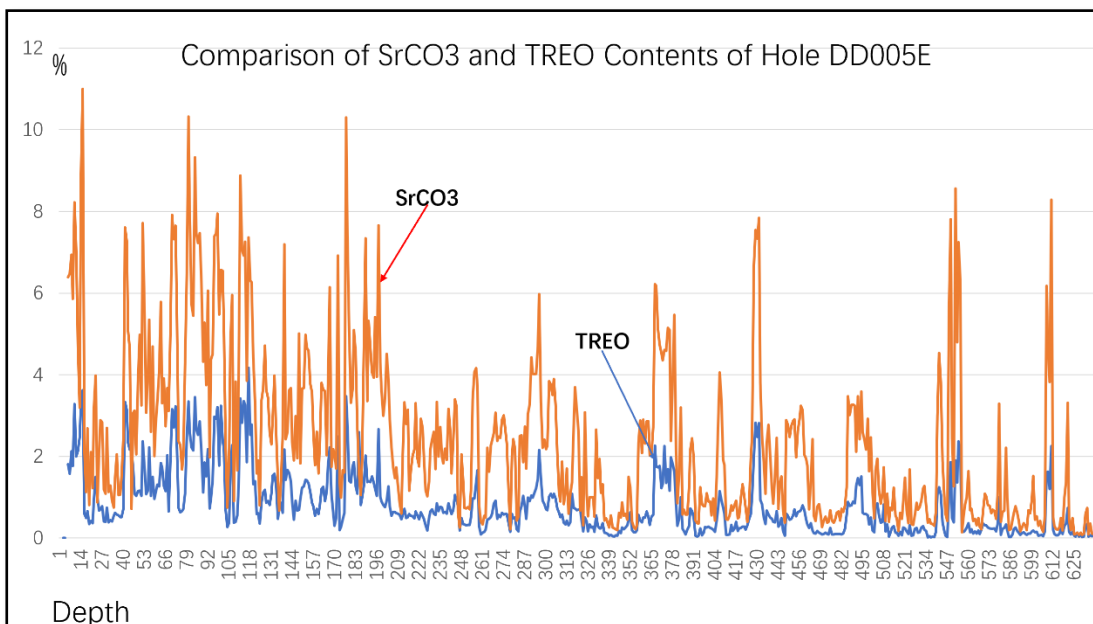
Figure 3: Grade correlation of SrCO 3 and TREO throughout the drillcore is strong.
