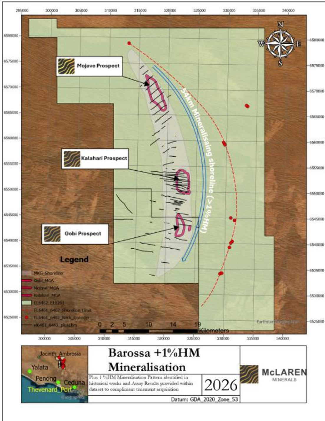
Figure 2 – Barossa Project Mineralisation envelope and interpreted shorelines.
