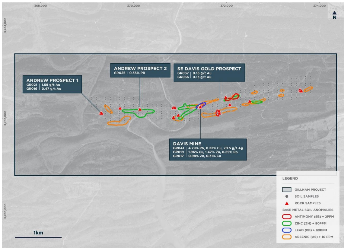
Figure 5 – West Gilham project area highlighting anomalous zinc, lead, gold and antimony.
