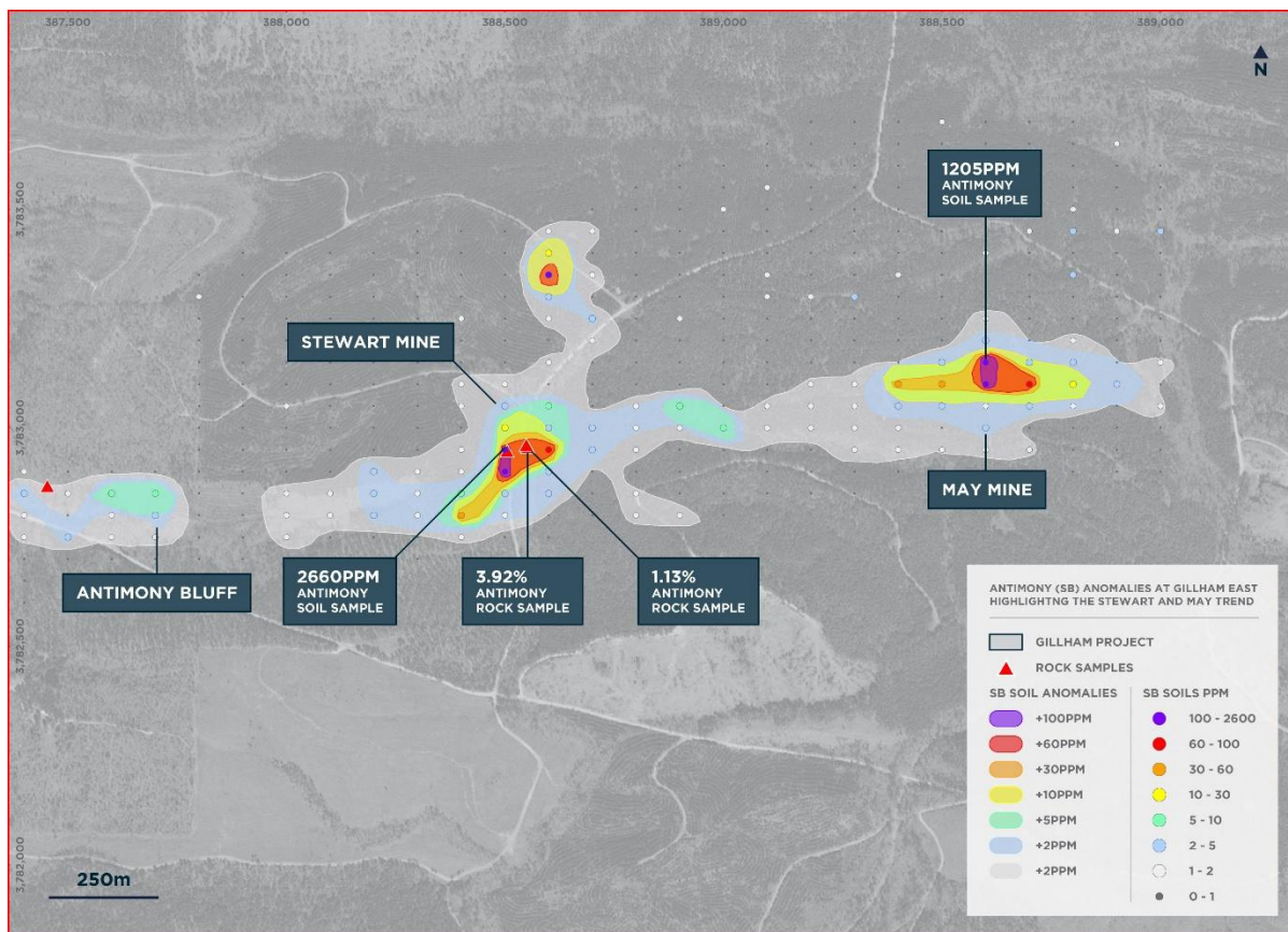
Figure 1. Antimony Soil anomalies highlight the historic May and Stewart undrilled prospects.
