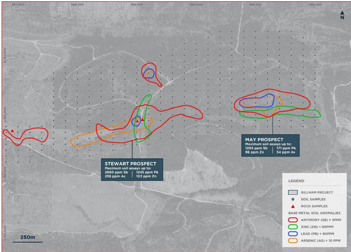
Figure 4 – East Gilham project area highlighting anomalous antimony, zinc, lead, and arsenic.
