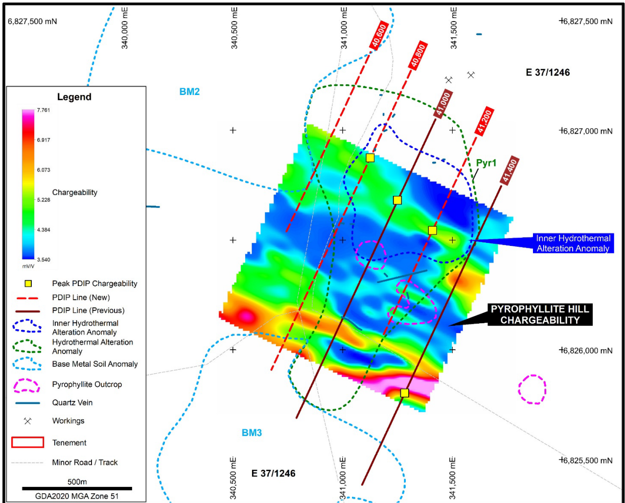
Figure 2: Pyrophyllite Hill PDIP lines with peak chargeability, main pyrophyllite outcrop and Pyr1 UFF soil anomaly on GAIP survey chargeability image
