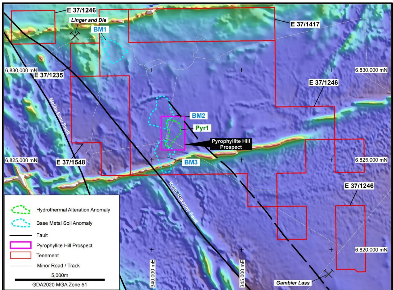
Figure 1: Pinnacle Well Project – Pyrophyllite Hill prospect location and UFF soil anomalies on aeromagnetic image
