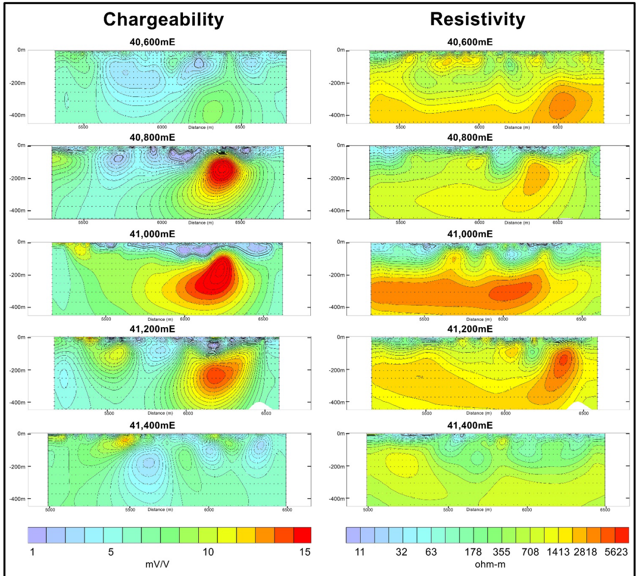
Figure 3: Pyrophyllite Hill PDIP survey chargeability and resistivity inversion models. Lines 40800E, 41000E and 41200E display strong coincident chargeable and resistive features (red) at depth, along with shallow chargeable lows (blue)
