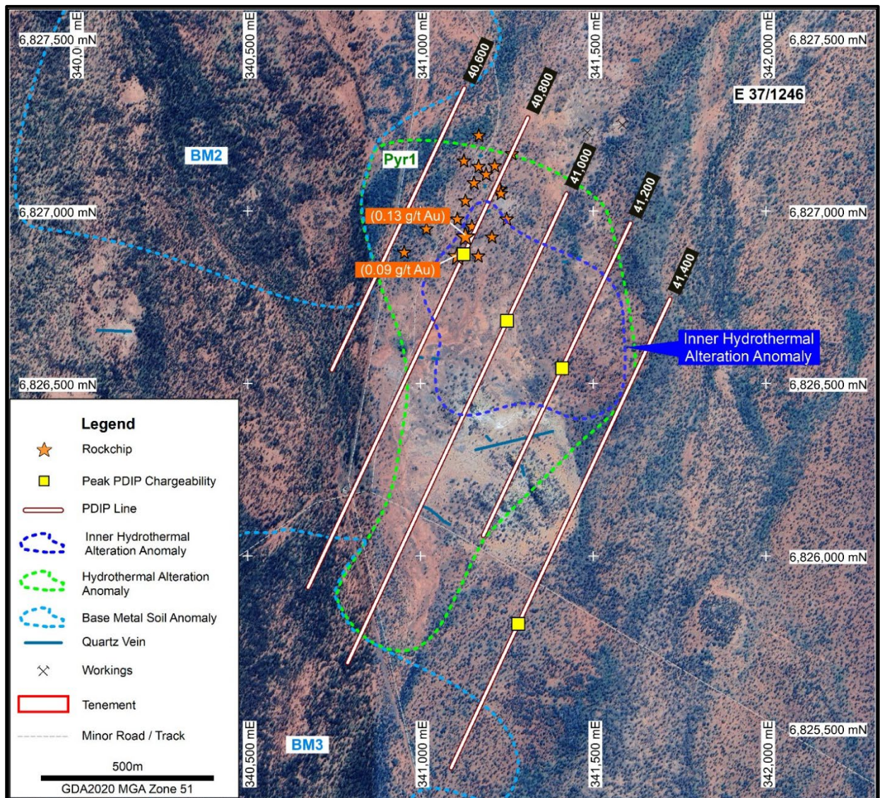
Figure 4: Pyrophyllite Hill Summary – PDIP lines with peak chargeability responses, UFF soil anomalies, historic rockchip samples and quartz veining on Google Earth image
