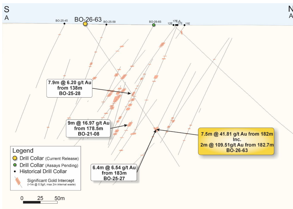
Figure 3 Cross section A-A' showing significant gold intersections ( \geq 1\text{m} @ \geq 0.5\text{g/t Au} , max 2m internal waste)
