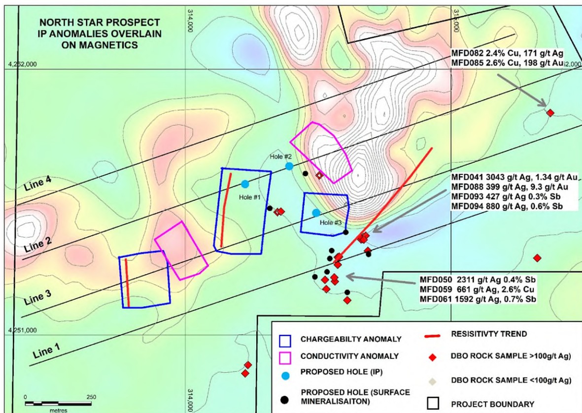
Figure 2 - Location of IP traverse lines, relative chargeability and conductivity IP anomalies overlain on magnetic 1VD image and contours. Warm colours are interpreted as intrusives
