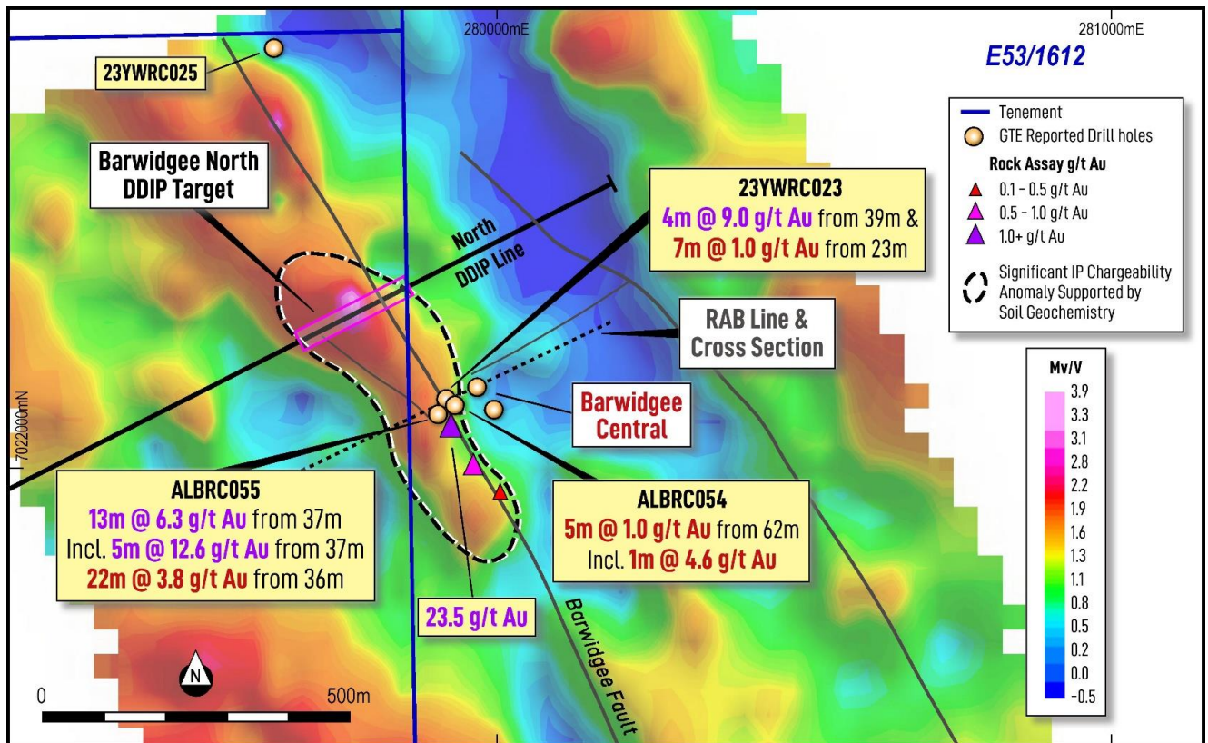
Figure 3: Map of the GAIP Chargeability showing the regional scale potential along the 2km Barwidgee Trend 7
