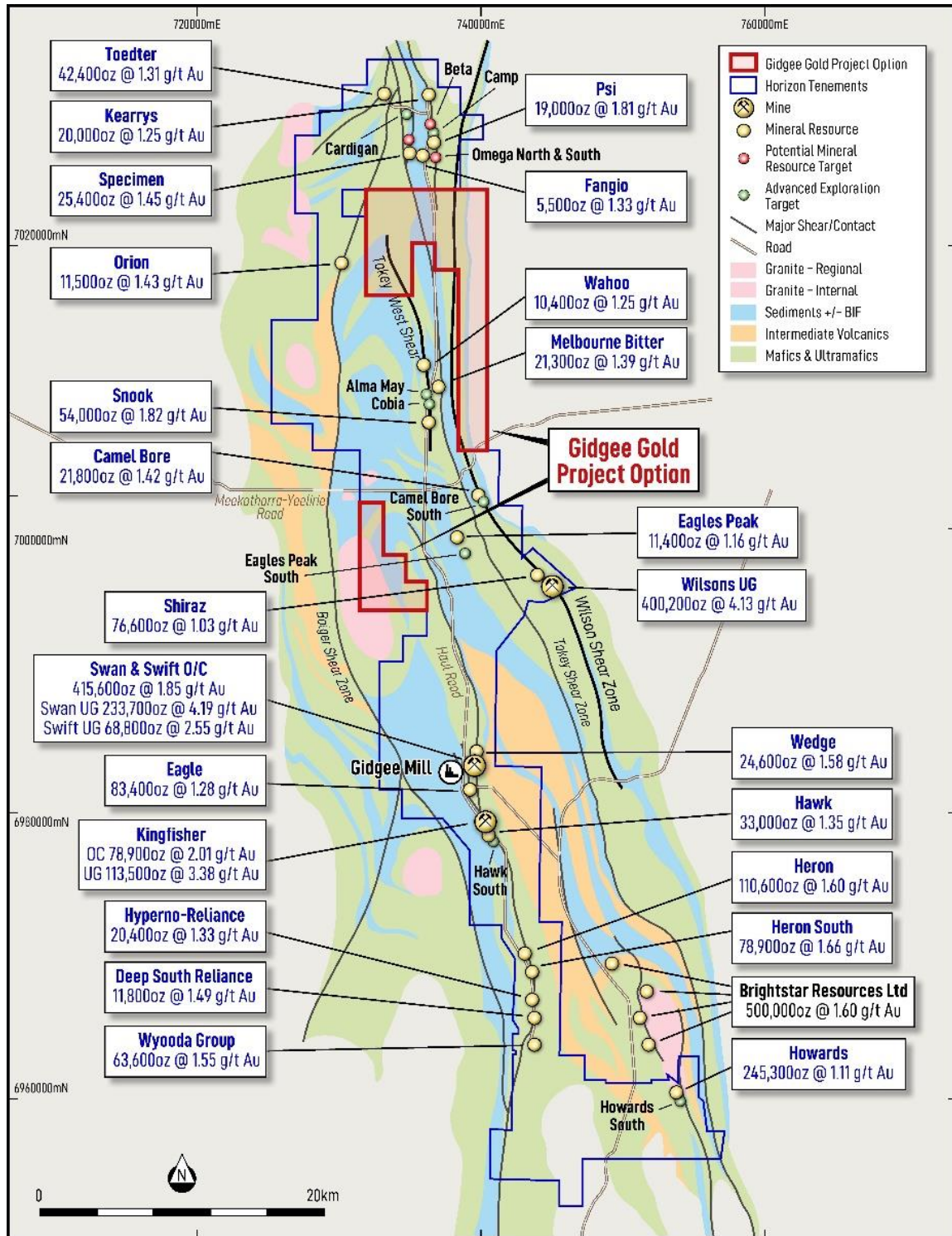
Figure 4: Gum Creek Gold Project location and major deposits within the Gum Creek Greenstone Belt. Note: Figure adapted from various Horizon Gold Limited Presentations 8,9,10,11
