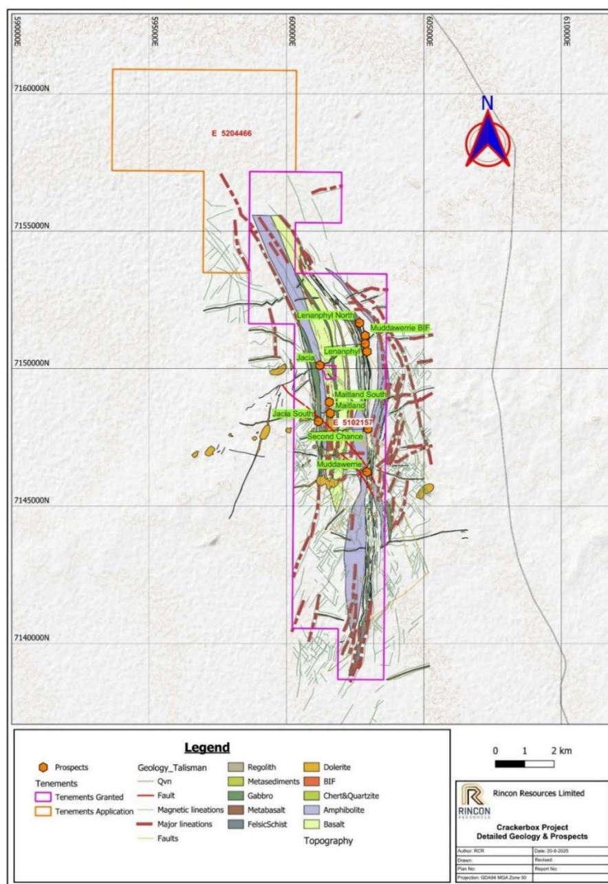
Figure 3 – Crackerbox Geological Setting
