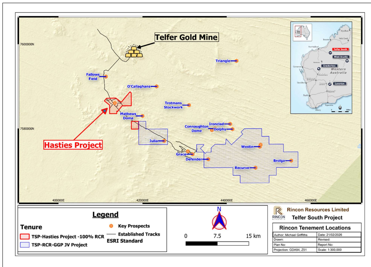
Figure 2 – Telfer South Project Location
