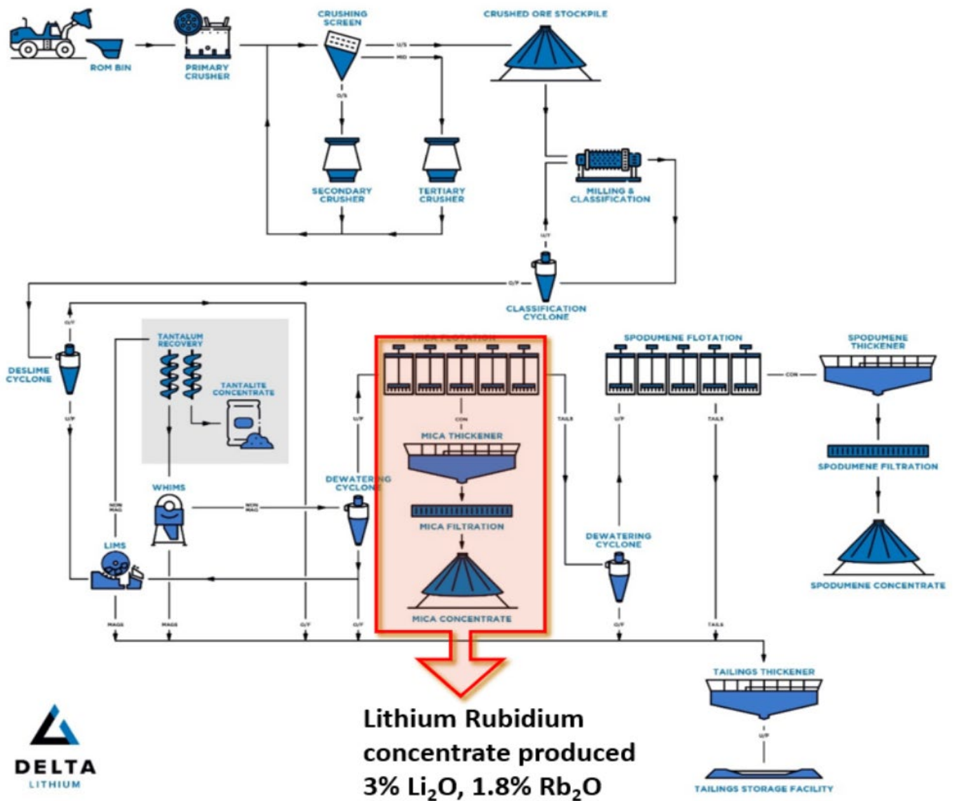
Figure 4: Block Flow diagram showing Mt Ida Lithium process flowsheet with average Li & Rb concentrate grades based on testwork to date
