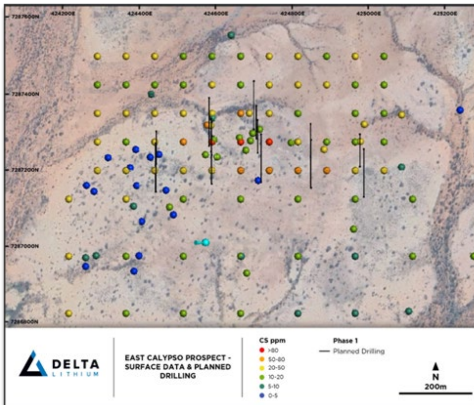
Figure 11: Plan view of East Calypso with surface data showing caesium anomalism
