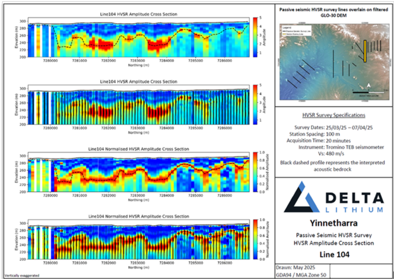
Figure 13: Passive seismic survey results mapping paleochannel
