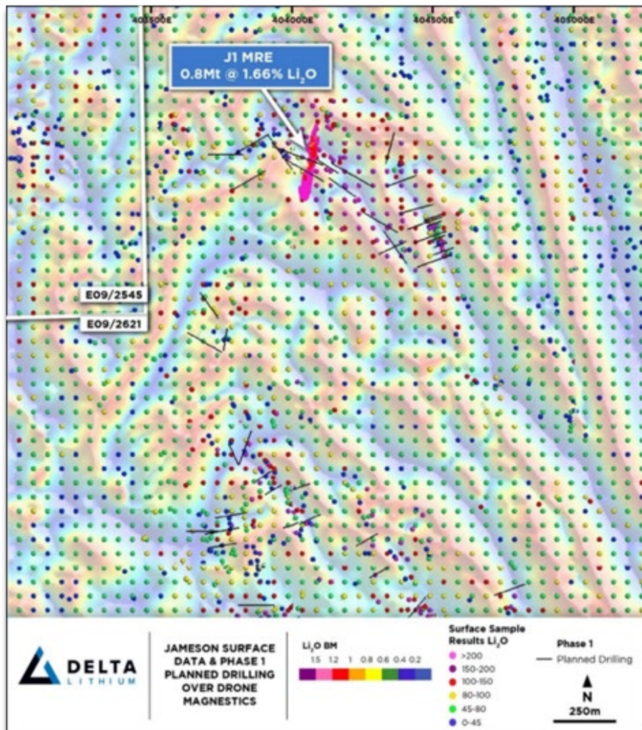
Figure 7: Plan view of Jameson with planned drilling
