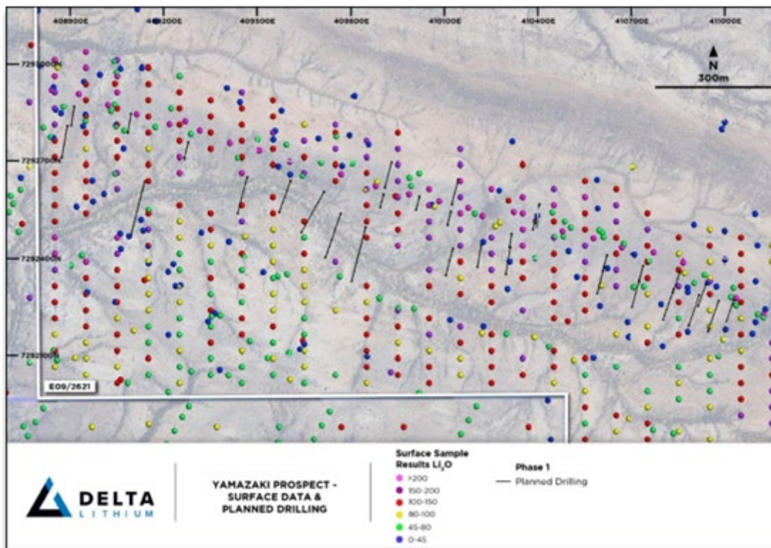
Figure 9: Plan view of Yamazaki prospect showing surface anomalies
