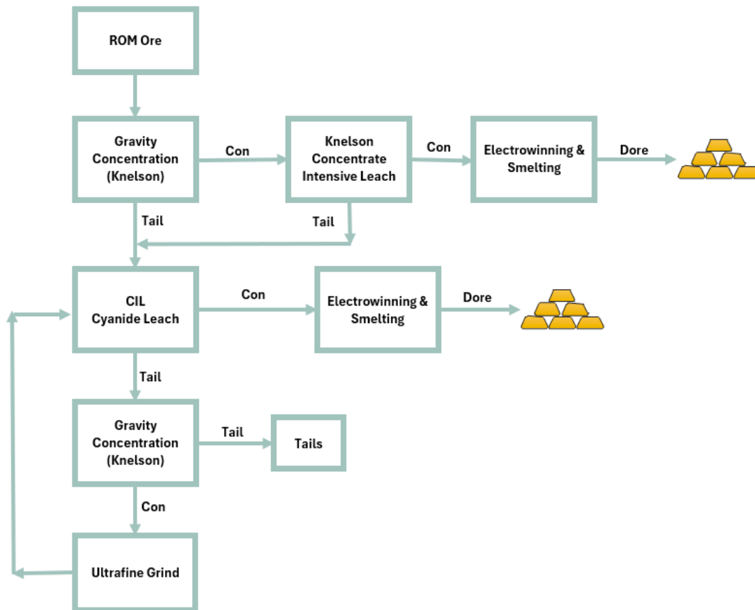
Figure 2: Test Work Process Flowchart
