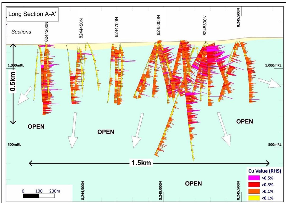
Figure 4: Cangallo Long Section A-A' showing the open-ended extent of copper mineralisation defined to date by the RC drilling program.
