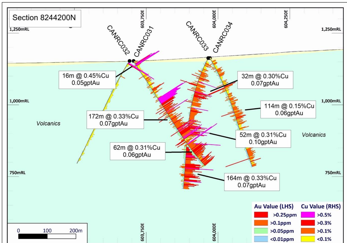
Figure 3: Cangallo RC drill section 8244200N showing copper intersections averaging +0.30% Cu – (NB: intersection for CANRC033 is based on 0.1%Cu cut off shown in Table 2)
