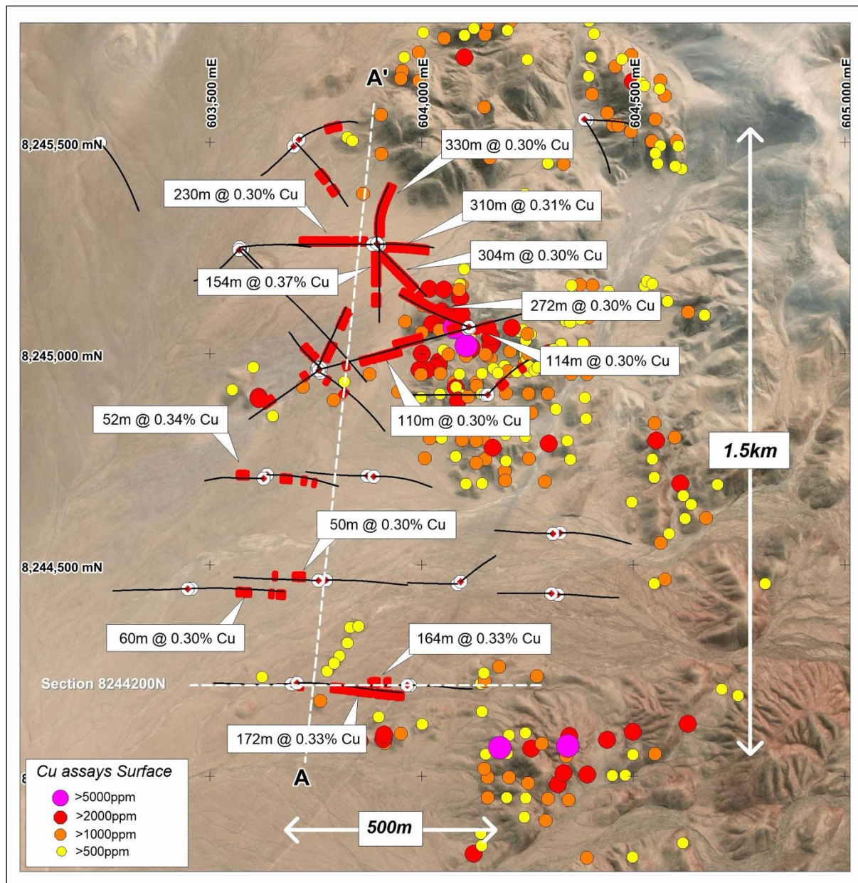
Figure 2: Cangallo Prospect showing location of Stage 3 RC drill-holes and significant intersections averaging greater than 0.3% Cu.
