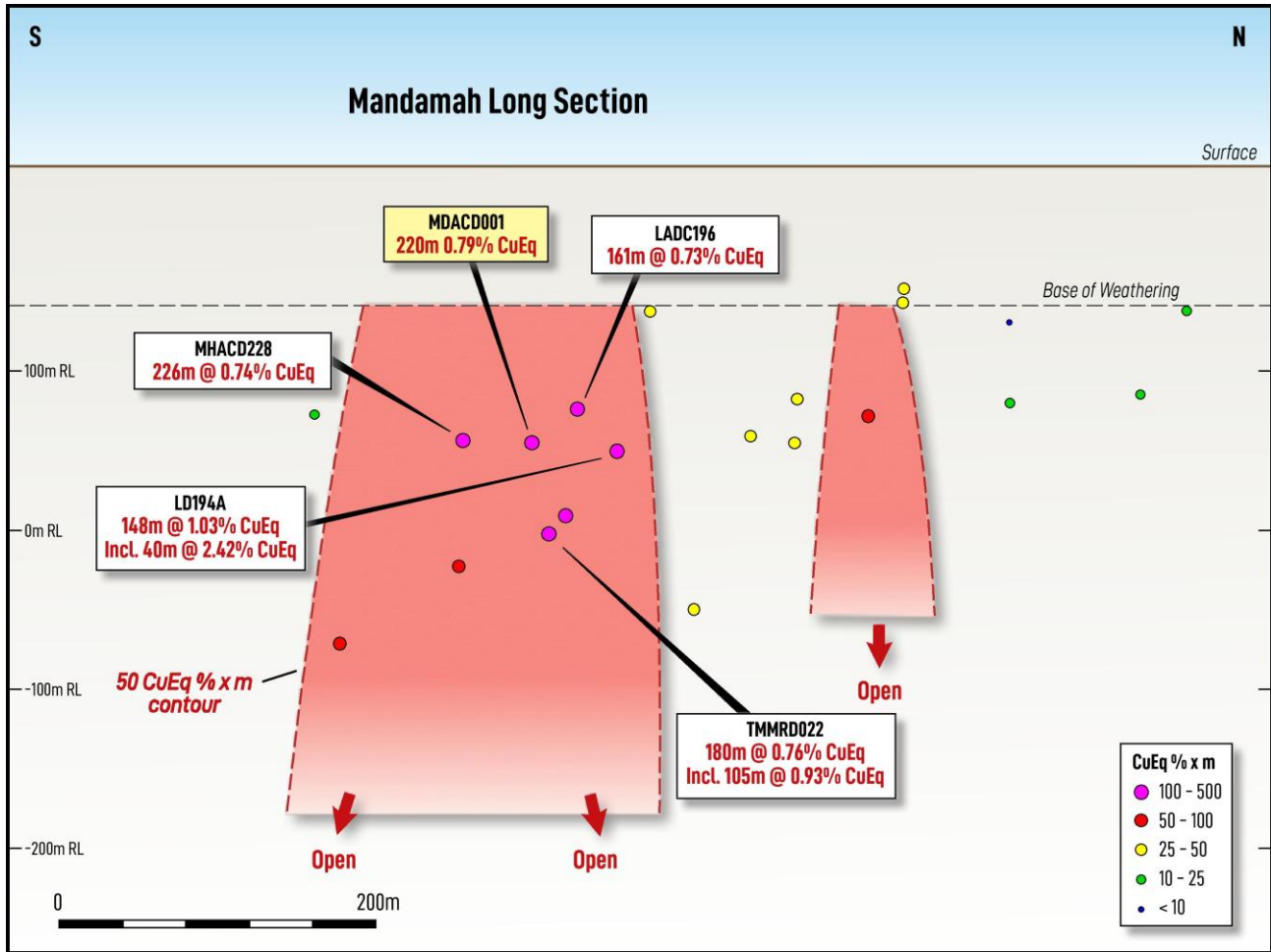
Figure 4: Mandamah long section illustrating the results from hole MDACD001.
