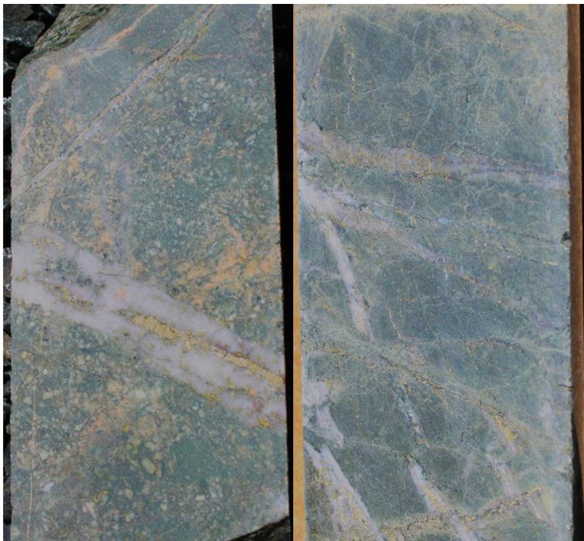
Figure 2: Core photos from MDACD001. Left 187.5m. Potassium feldspar, magnetite and biotite altered diorite porphyry hosting quartz veined, bornite, chalcopyrite and pyrite mineralised stockwork 0.44g/t Au & 0.42% Cu Right 293.4m. Magnetite, biotite altered volcaniclastic hosting quartz-magnetite veined, chalcopyrite & pyrite mineralised stockwork 0.4g/t Au & 0.71% Cu.
