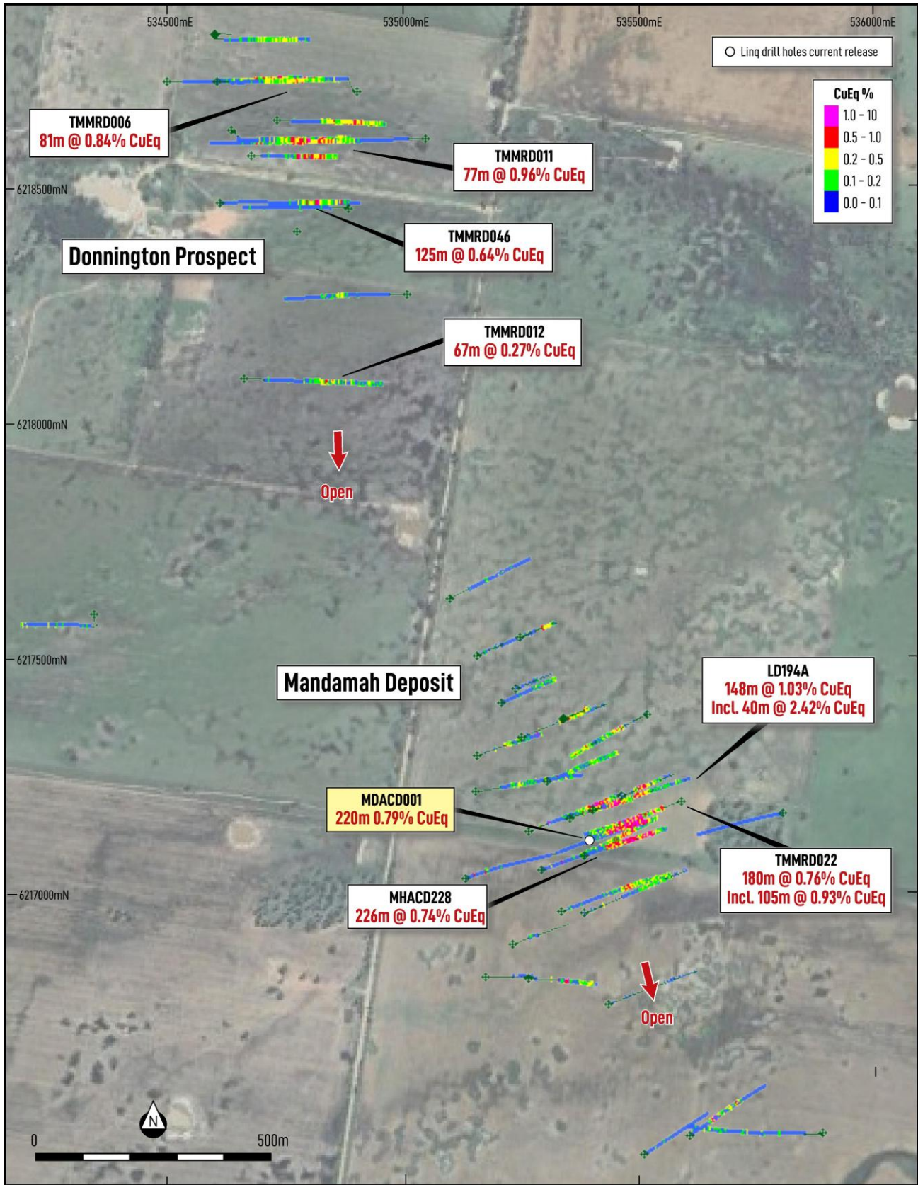
Figure 3: Mandamah/Donnington plan image illustrating the location of drilling results for MDACD001.
