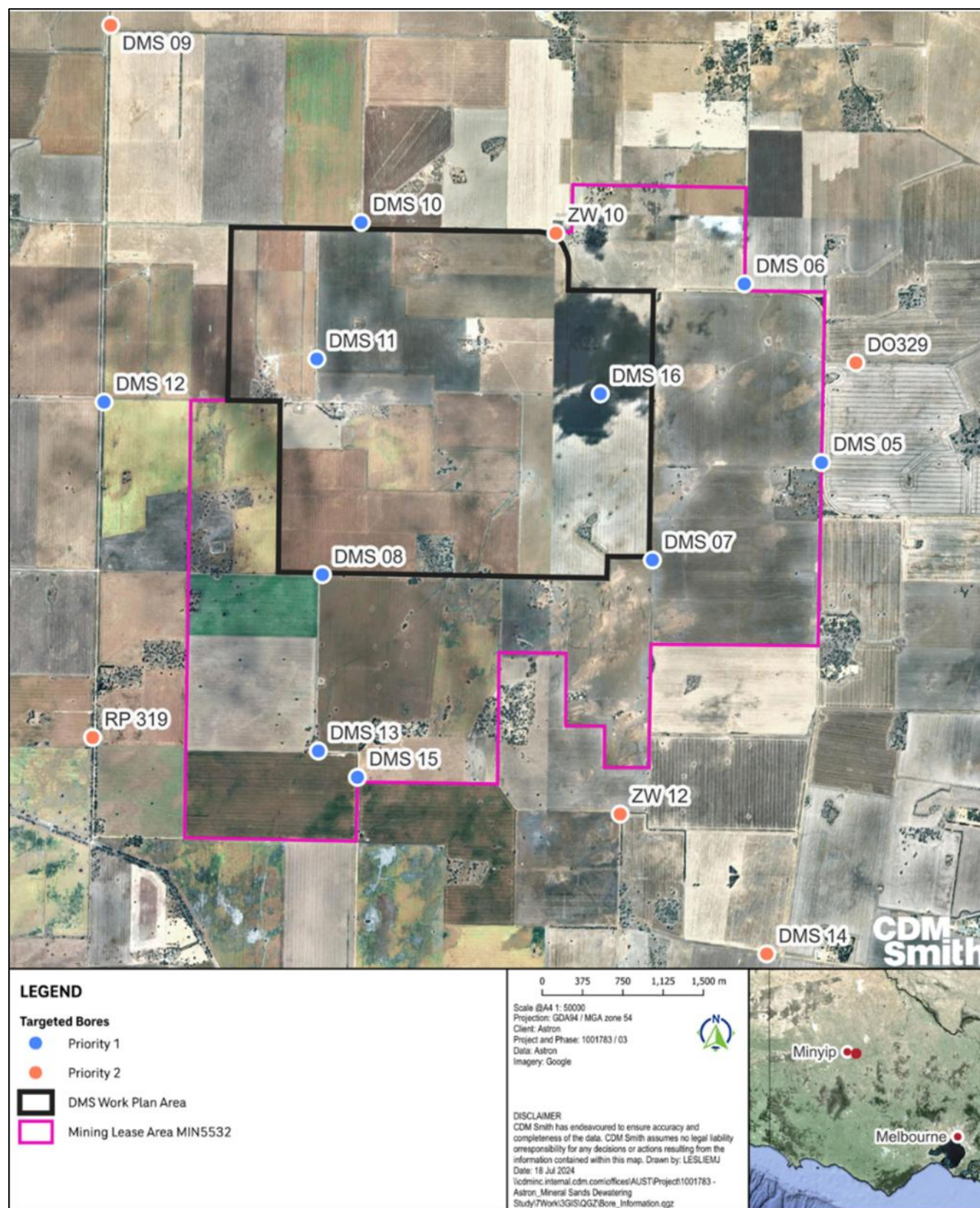
Figure 16.2 Location of wells for 2024 slug testing
