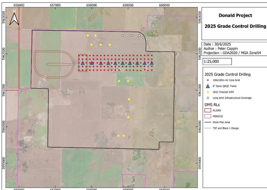
Figure 10.2 Drilling in MIN5532 (purple outline) during 2025 – not used for Mineral Resource estimation
