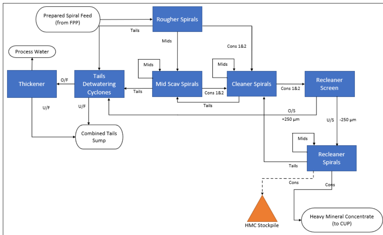
Figure 17.4 WCP spiral circuit flowsheet
