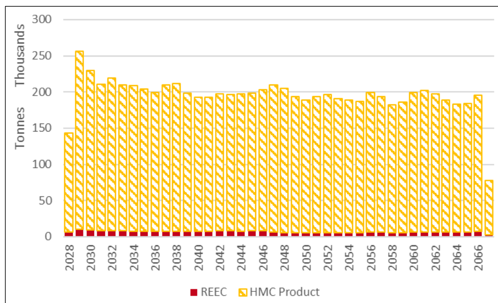
Figure 16.9 Annualized MIN5532 concentrate product schedule
