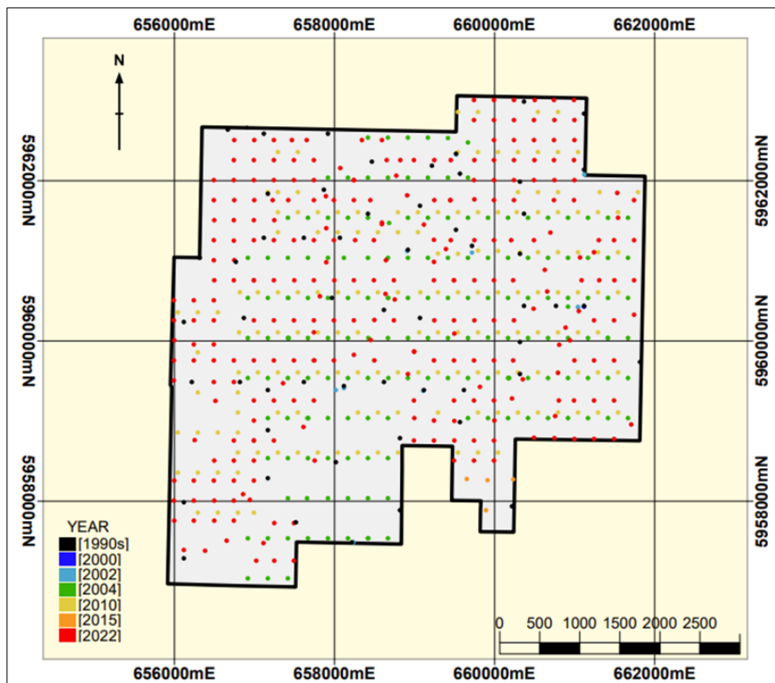
Figure 10.1 Drilling in MIN5532 (black outline) coloured by year and used for Mineral Resource estimation
