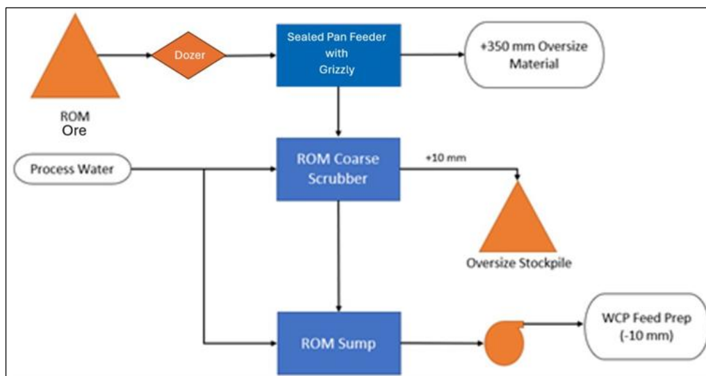
Figure 17.1 MUP flowsheet
