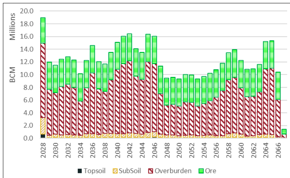
Figure 16.7 Annualized MIN5532 mining schedule – ex-pit movement
