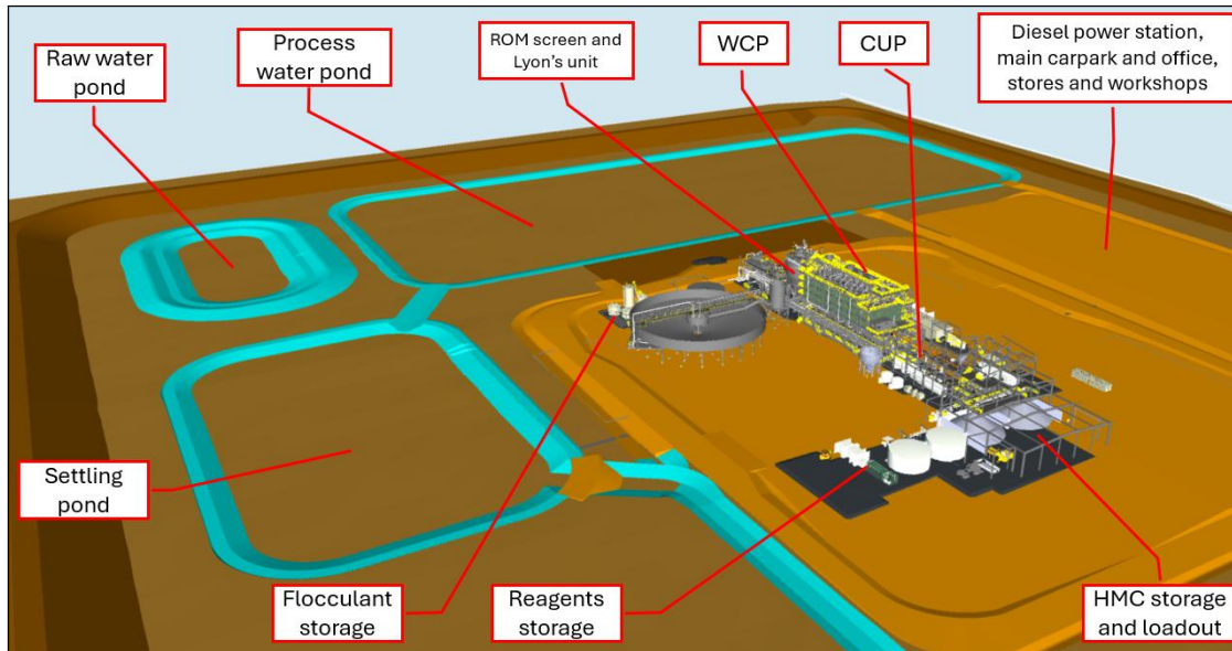
Figure 17.2 Process plant layout
