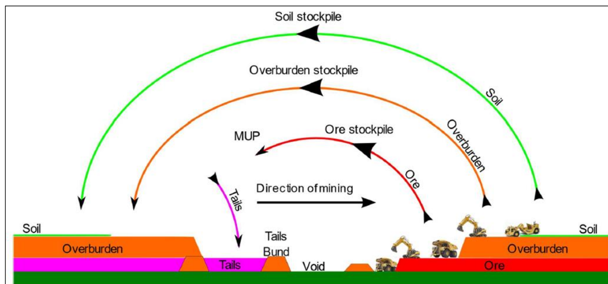
Figure 16.1 Schematic cross-section of mining approach (conceptual)
