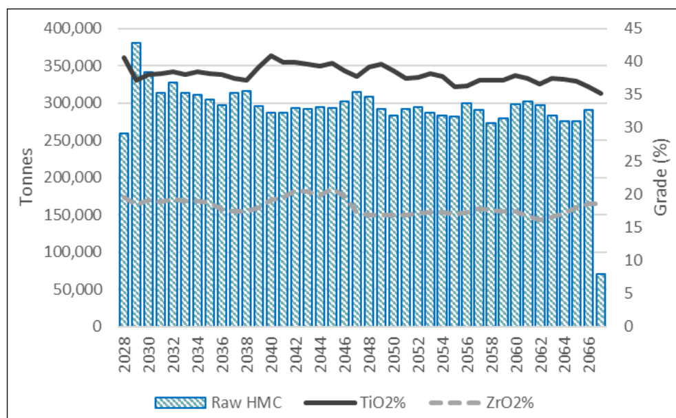
Figure 16.8 Annualized MIN5532 processing schedule – raw HM
