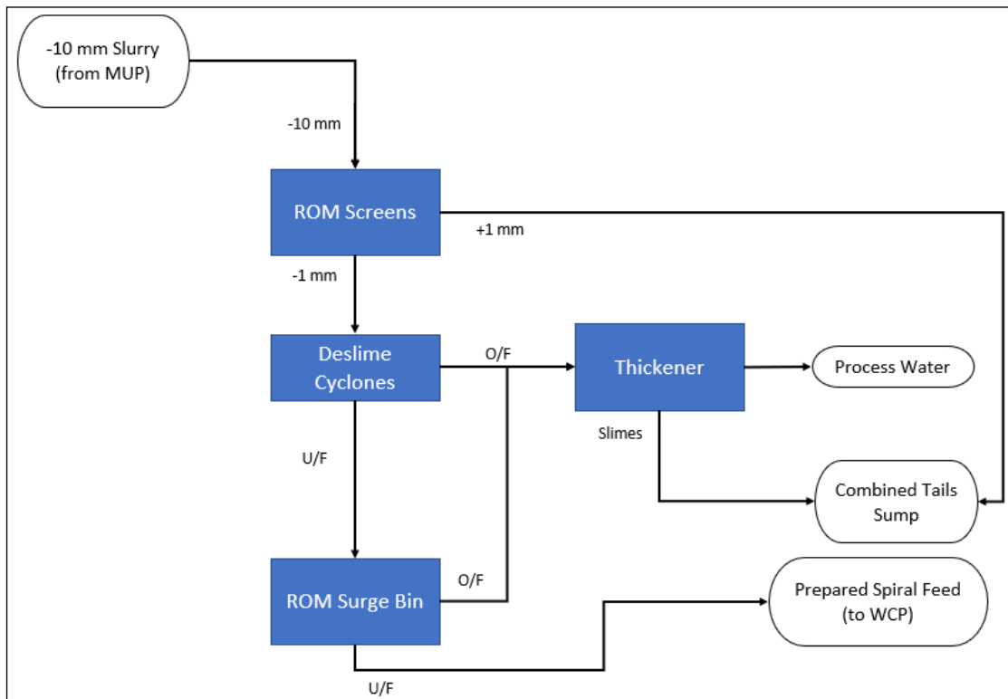
Figure 17.3 WCP feed preparation circuit flowsheet
