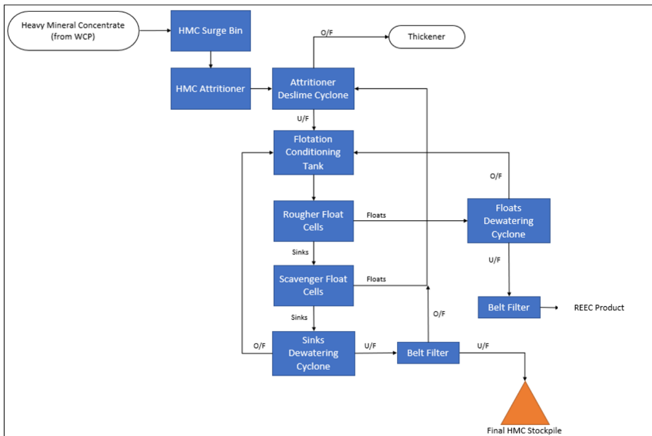
Figure 17.5 CUP circuit flowsheet
