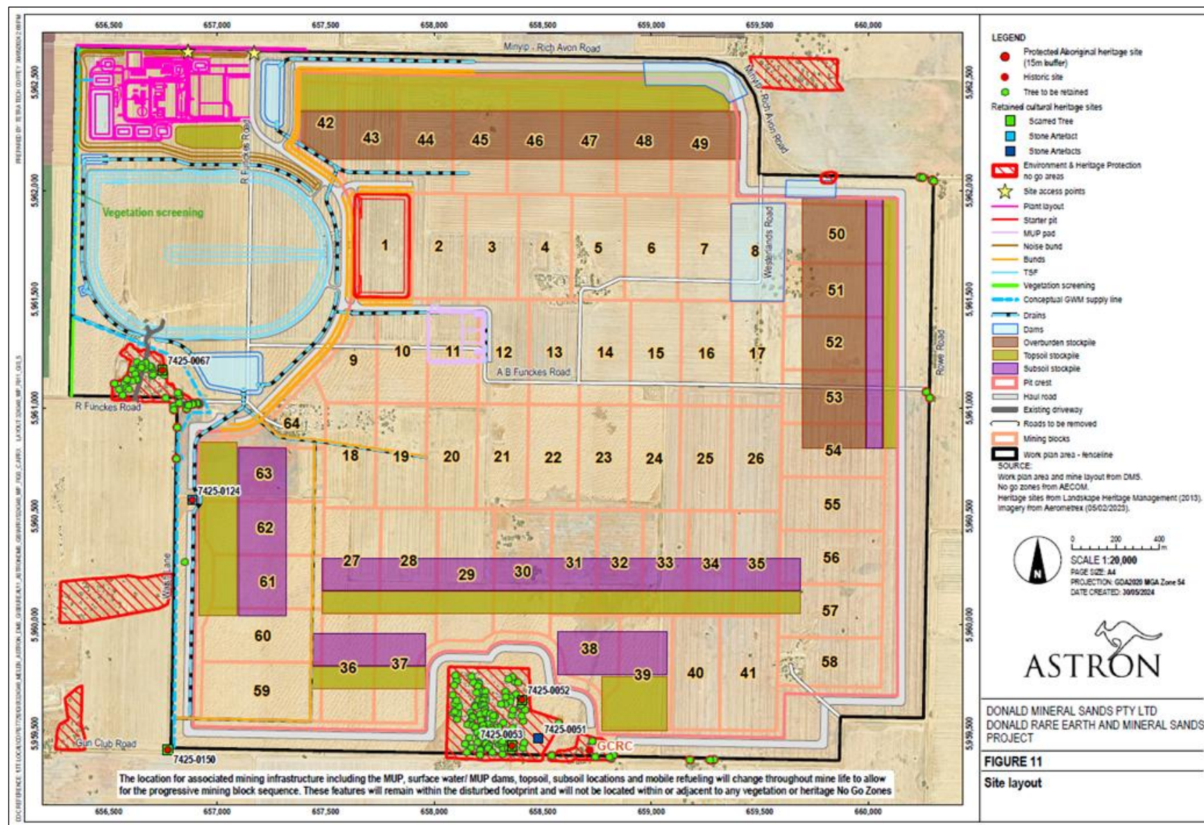
Figure 18.1 Site layout in Work Plan area
