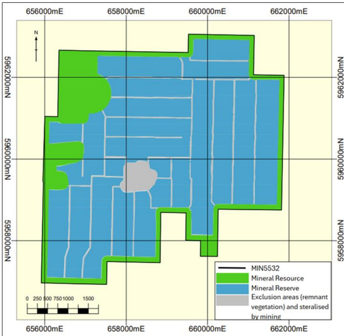
Figure 14.6 Plan of 2025 Mineral Reserve area and remaining 2025 Mineral Resource within MIN5532
