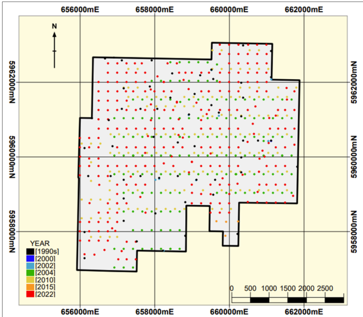
Figure 2: Drilling in MIN5532 (black outline) coloured by year, used for Mineral Resource estimation
