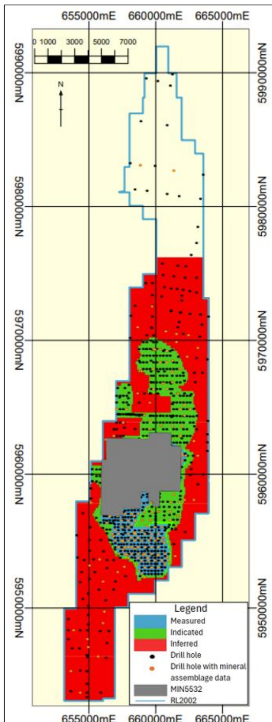
Figure 24.5 RL2002 resource classification
