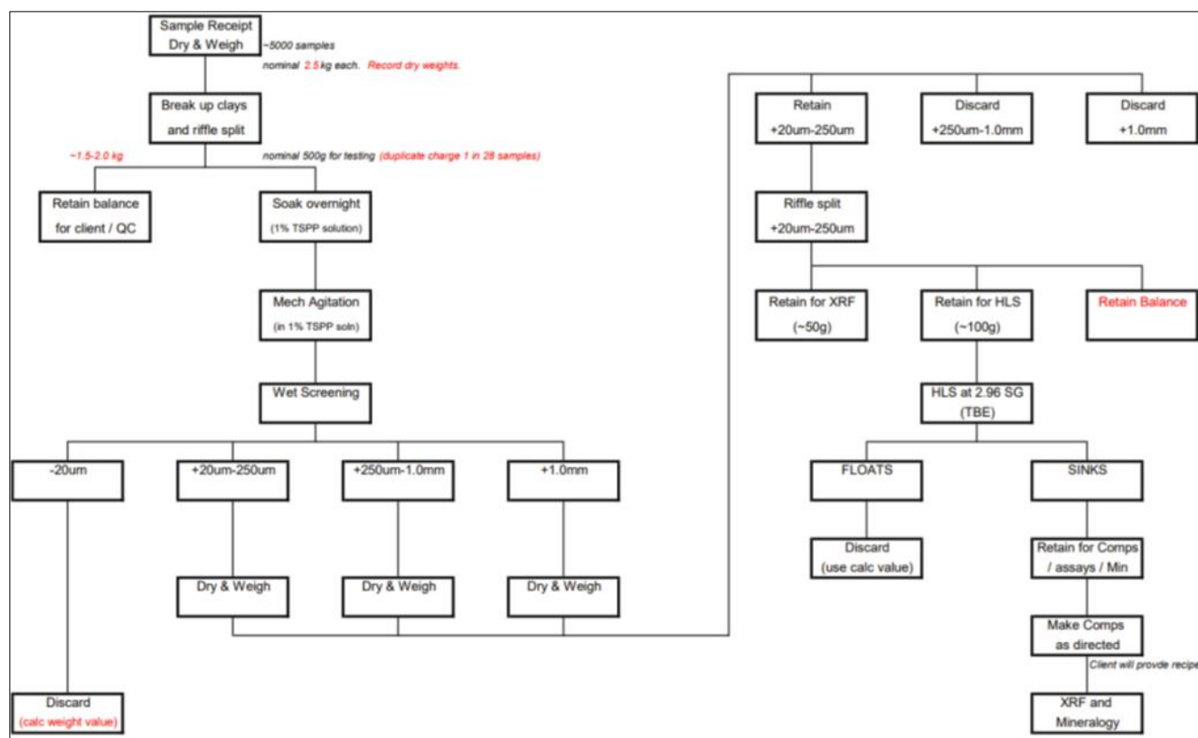
Figure 11.1 2022 analytical testwork flowsheet
