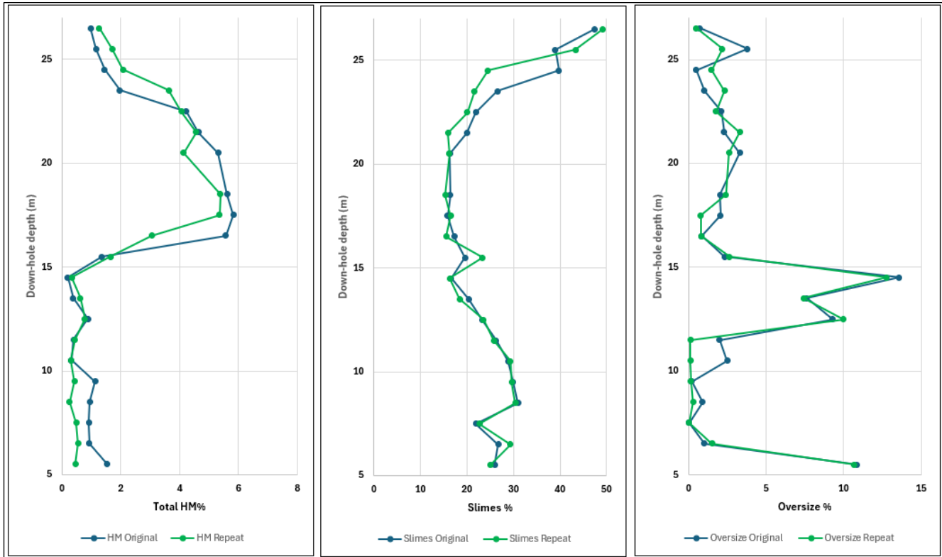
Figure 12.1 DMS170 – downhole plots for verification results for total HM (left), slimes (centre) and oversize (right) results
