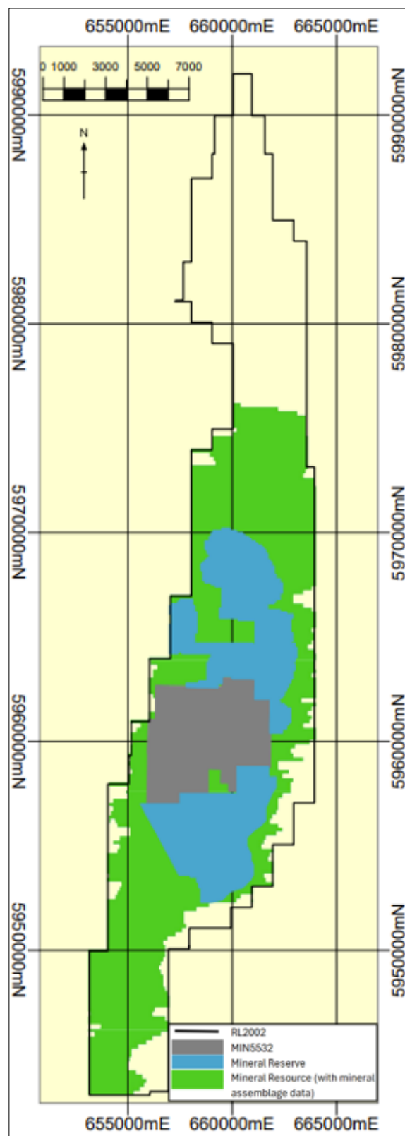
Figure 24.6 Plan of reserve area and remaining historical resource (with mineral assemblage data) within RL2002
