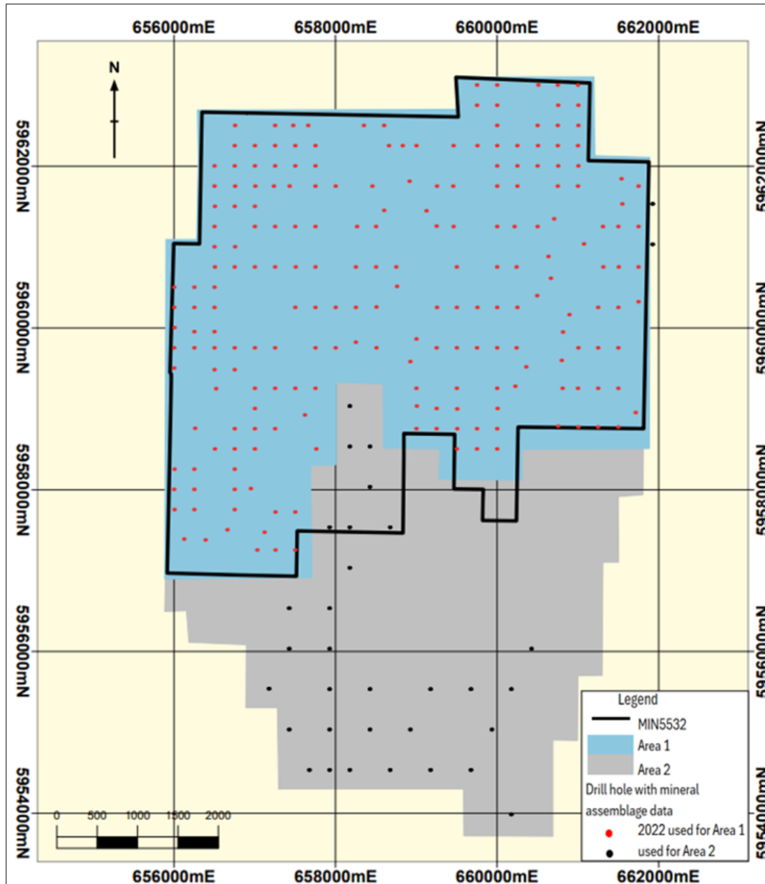
Figure 14.3 Plan of drillholes with mineral assemblage data used for Area 1 and Area 2
