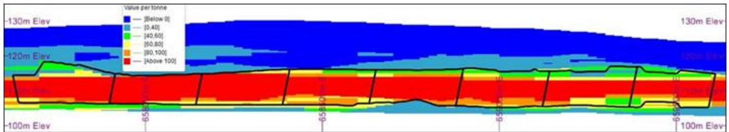
Figure 15.2 Long section through first eight ore blocks (5961700 mN)
