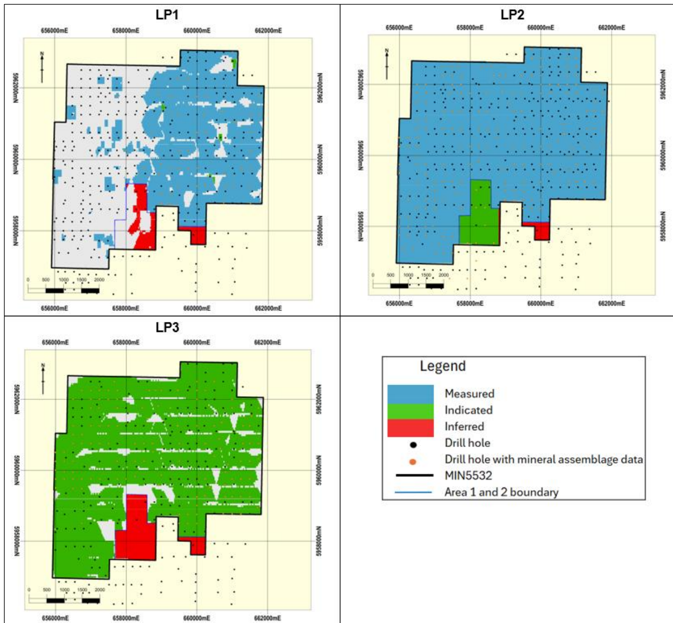
Figure 14.5 MIN5532 Mineral Resource classification
