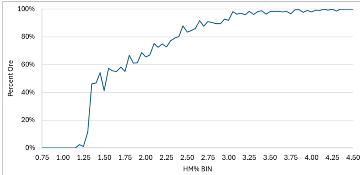
Figure 15.1 Cut-off grade curve – percent ore and equivalent total HM%
