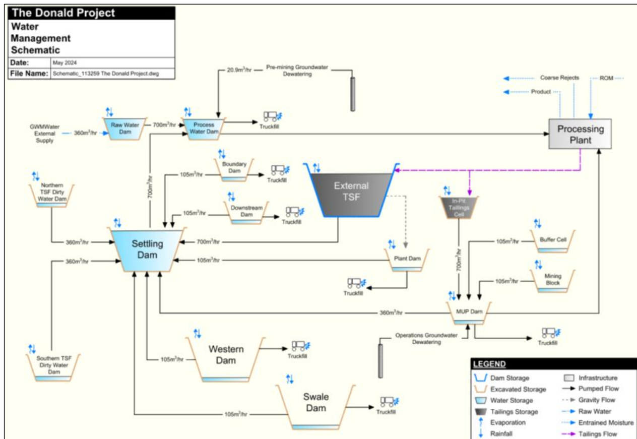
Figure 20.2 Water management system schematic
