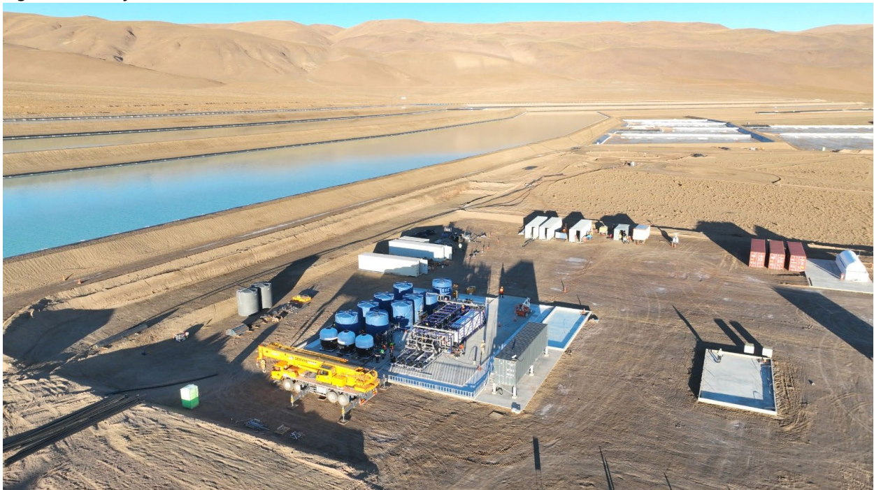
Figure 1. Nanofiltration Plant at HMW
