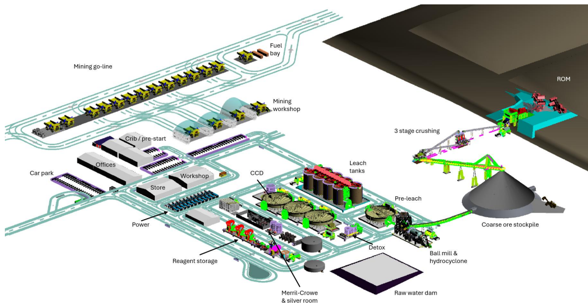
Figure 1.7 Conventional process: crush–grind–leach–Merrill–Crowe silver recovery
