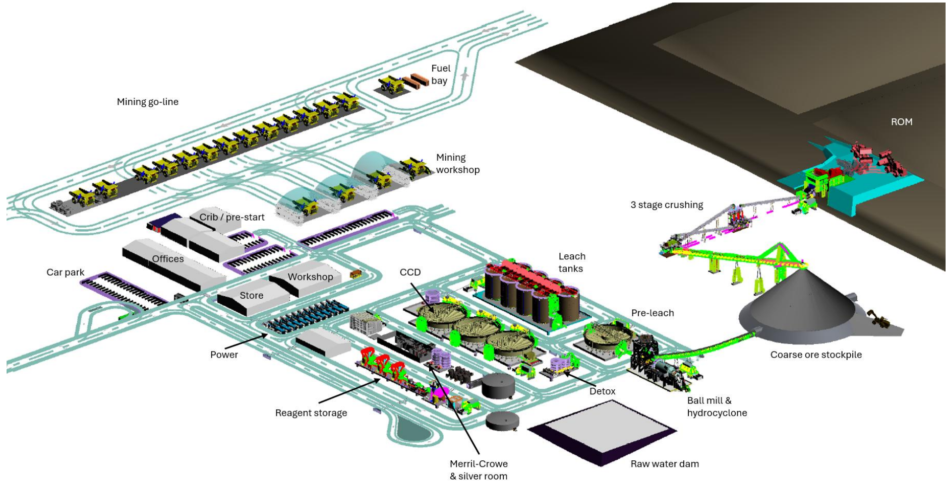
Figure 6.2 General site layout
