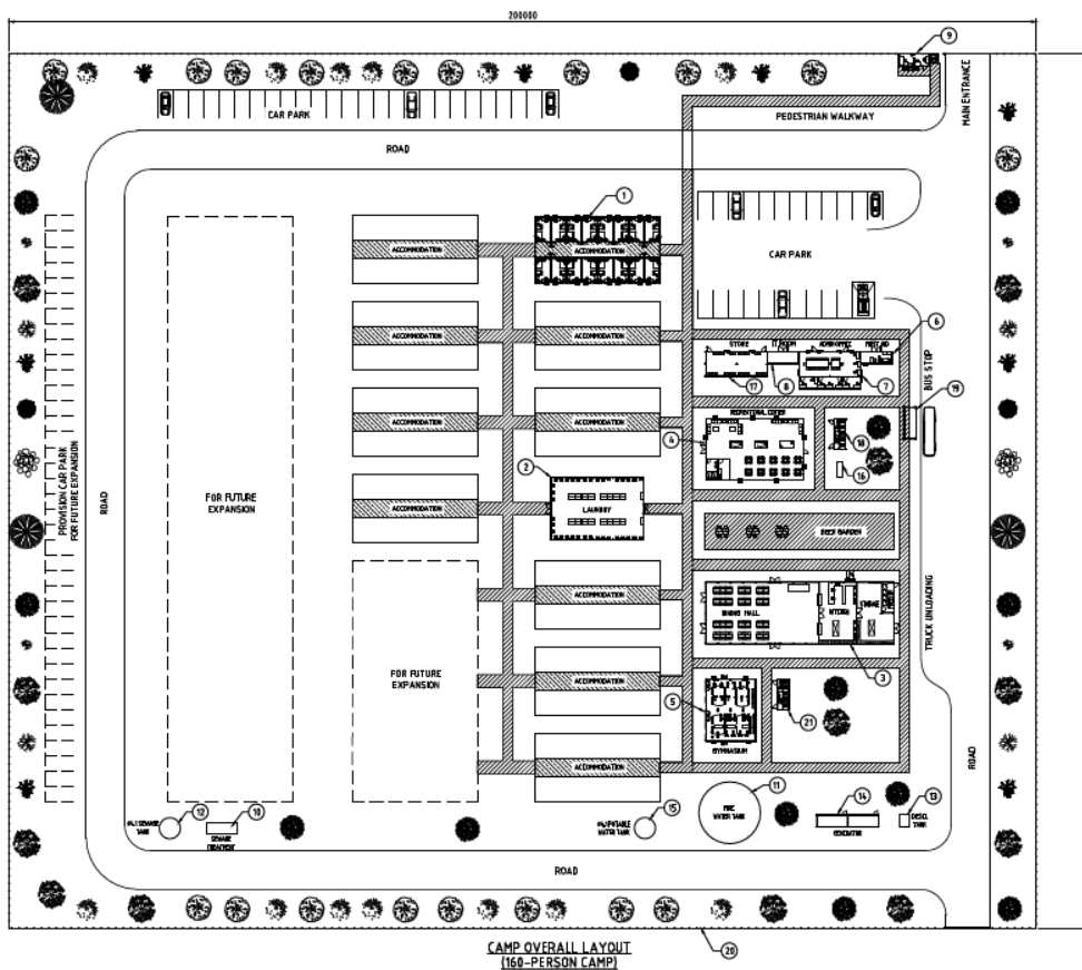
Figure 7.2 Camp layout
