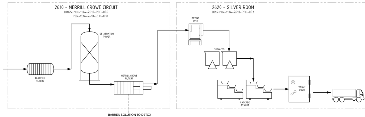
Figure 6.8 Merrill Crow & Silver Room
