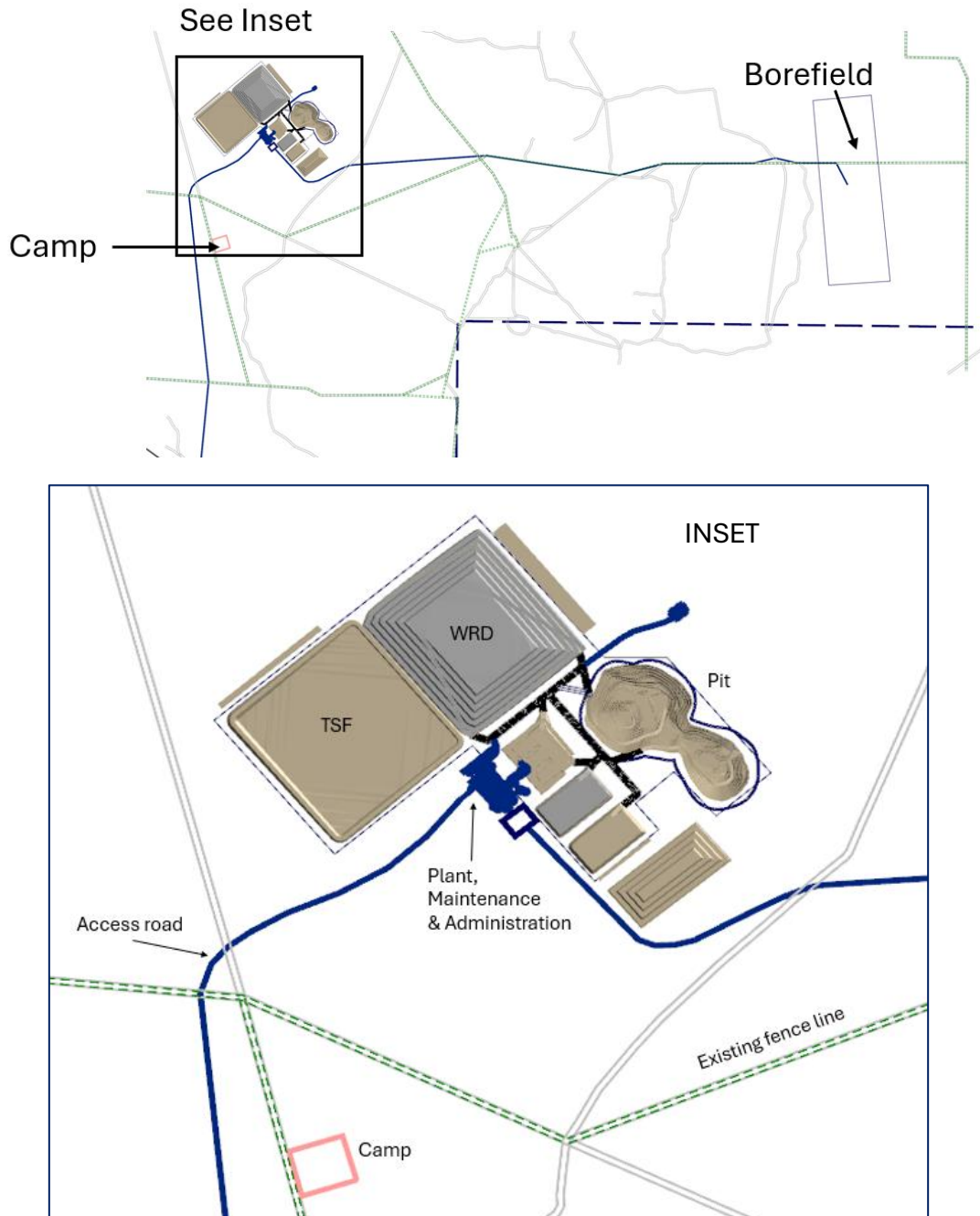
Figure 7.1 Site layout
