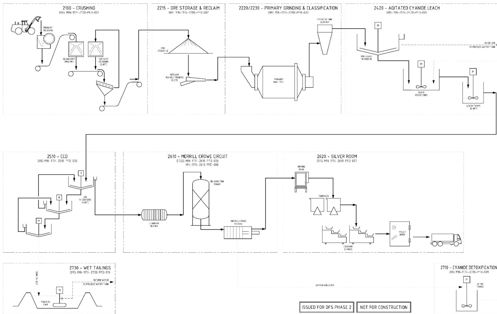
Figure 6.1 Simplified process flowsheet
