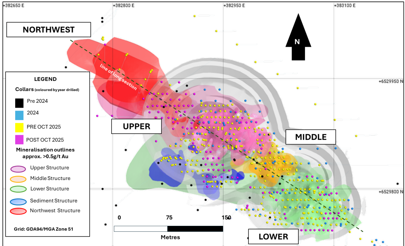
Figure 4: Plan view at the Lady Herial deposit scale, illustrating all drilling (by period drilled) along with location of long section shown in Figure 5.
