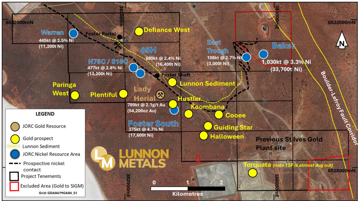
Figure 3: Foster-Baker Project Area showing select high-ranking gold prospects, gold & nickel Mineral Resource 7 positions.
