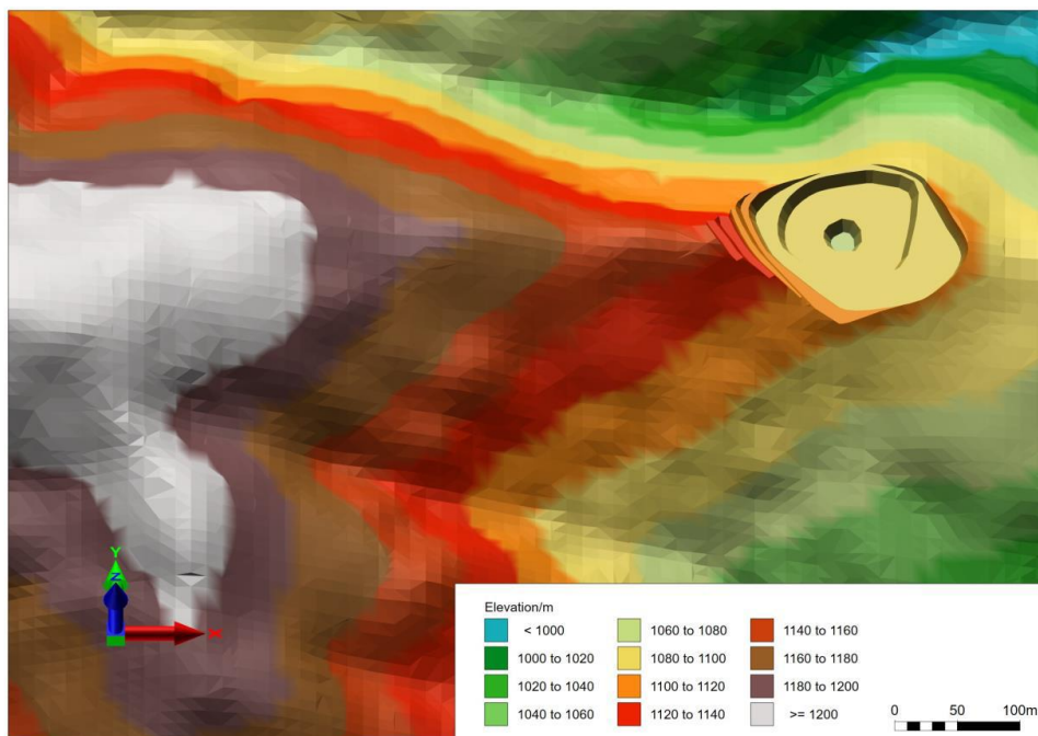
Figure 15: Development of Pit Stage Designs Pushback 1
