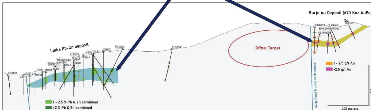
Figure 10: Cross section through the Barje and Liska deposits, with tagged core photographs showing similarities in mineralization styles between the two deposits.
