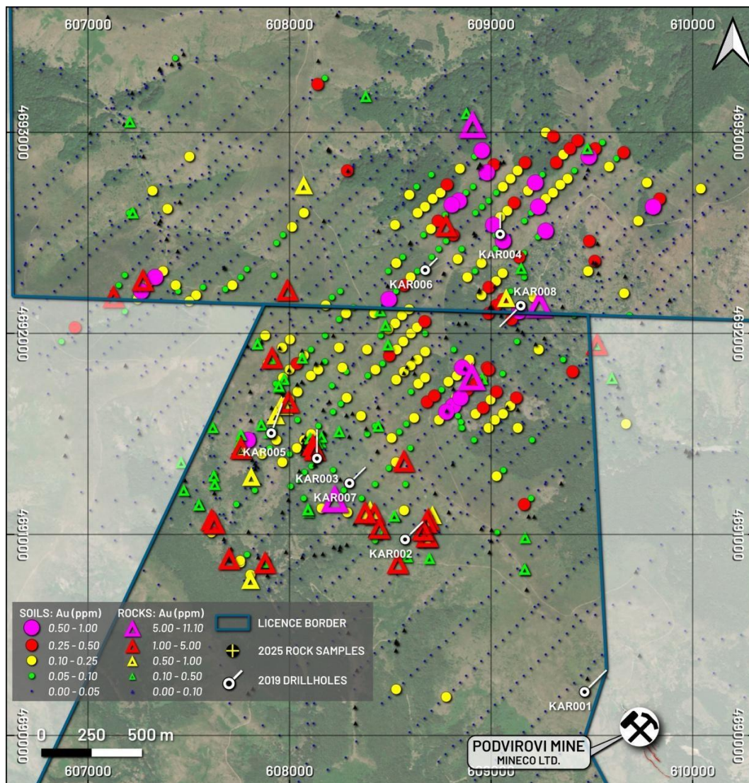
Figure 5: Distribution of gold grades in soil and rock samples at Karamanica. (EPSG: 32634).
