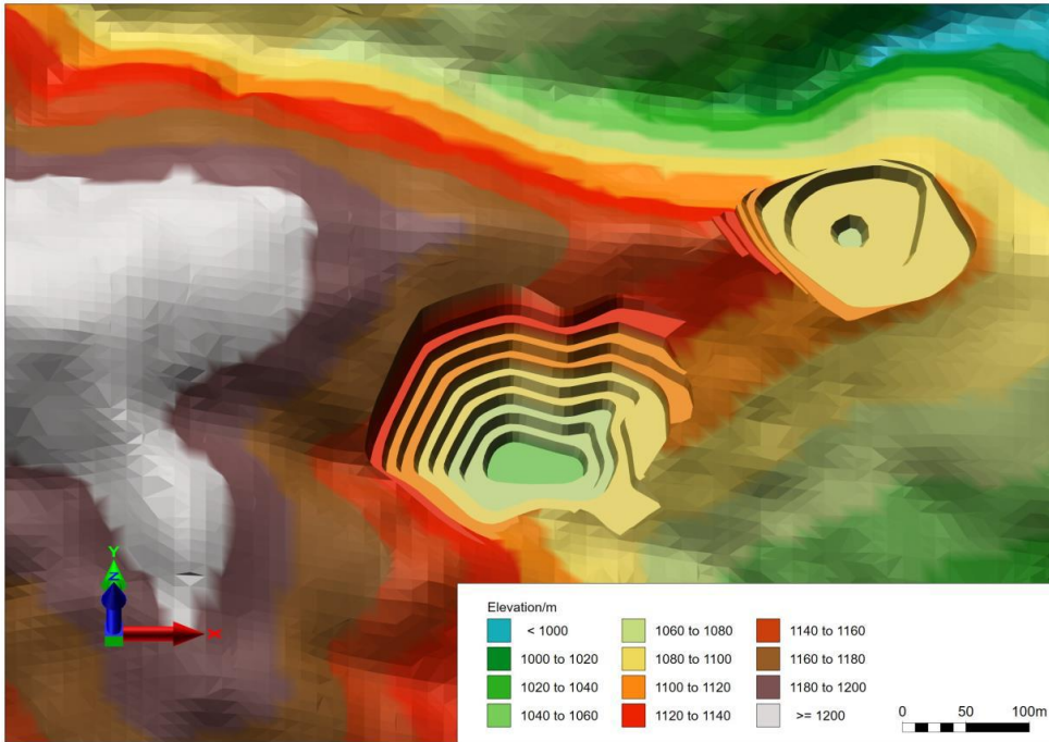
Figure 16: Development of Pit Stage Designs Pushback 2
