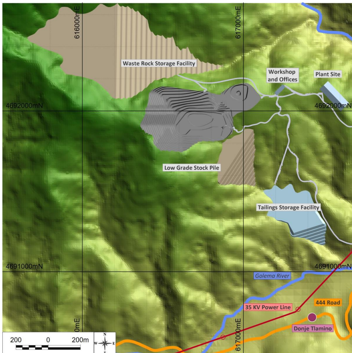
Figure 19: Plan View of Pit Limit and location of the WRSF and LG Stockpile
