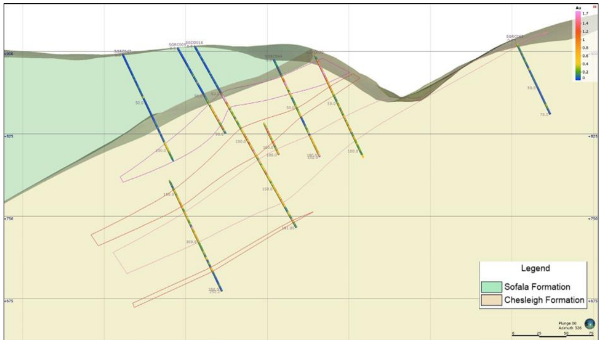
Figure 6: Spring Gully Project Typical Cross Section Looking North Sunny Corner Project
