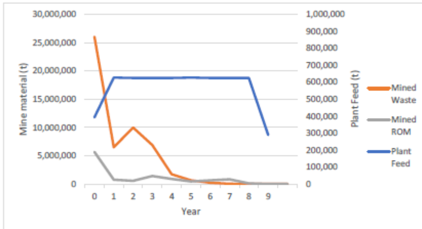
Figure 13: ROM production tonnes by period
