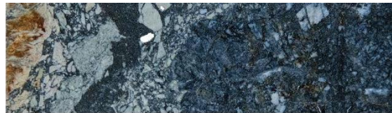
Photograph of core from Barje Hole BAR013, 84 - 85 meters and assaying 13.15 g/t Au, 78 g/t Ag, 1.4% Pb and 2.7 % Zn
