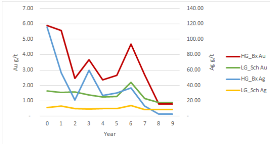
Figure 14: Processed grade by period.
