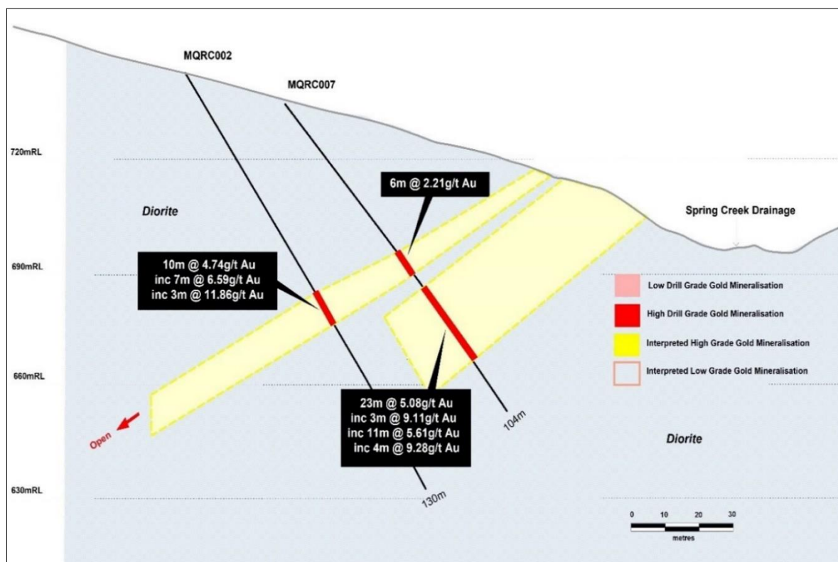
Figure 5: Queenslander Project Typical Cross Section Looking North Spring Gully Gold Project
