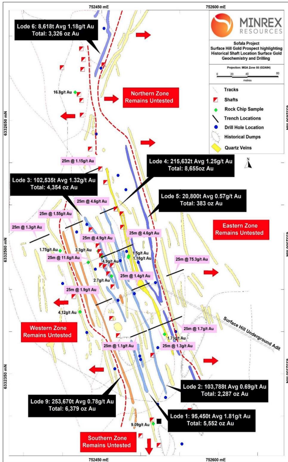
Figure 4: Surface Hill Drill Hole Location Map highlighting Projected Mineral Resource along with proximal surface and Hard Rock Mined Areas
