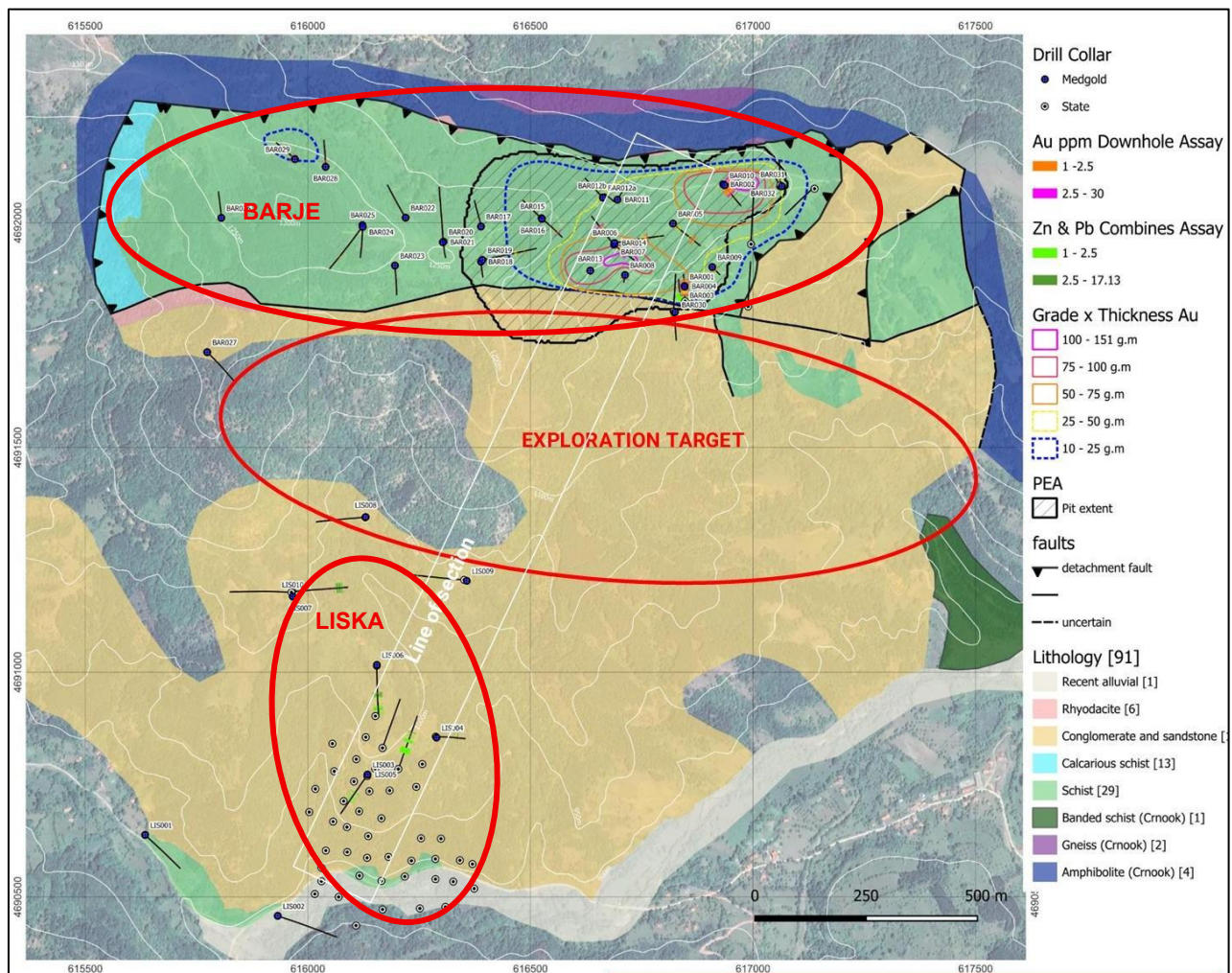
Figure 9: Plan view geology map showing the location of the Liska Target and drill holes complete to date at the Barje Deposit and Liska Target.
