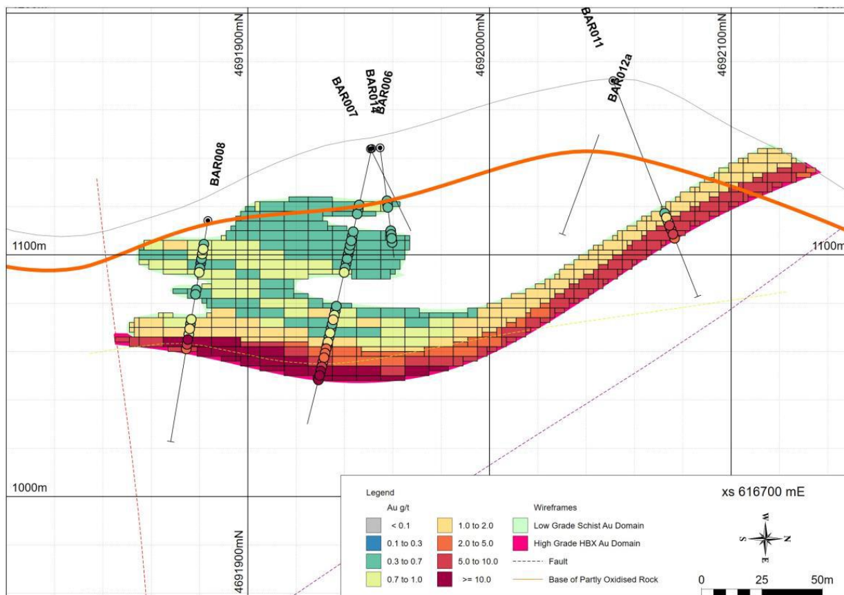
Figure 12: Example cross section 616700 mE. Composite data and block model both colour coded to Au grade.
