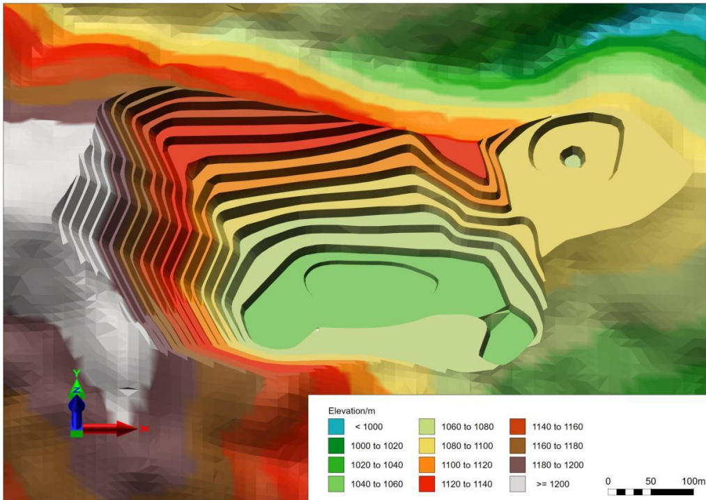
Figure 18: Development of Pit Stage Designs Pushback 4
