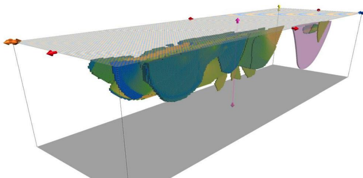
Figure 3: Sofala Gold Resources Oblique 3D View of Block Model
