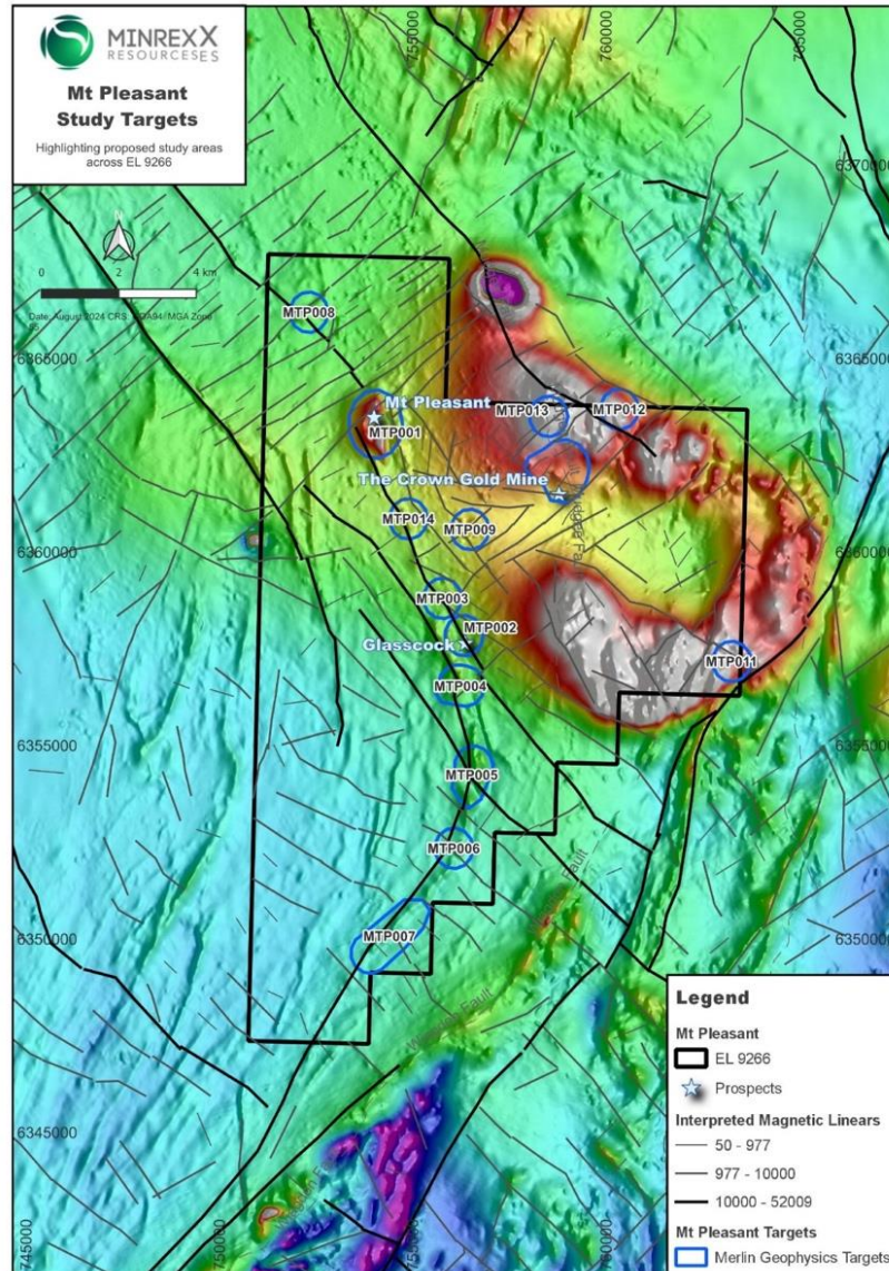
Figure 8: Targets From Study On Magnetic Image Over EL 9266
