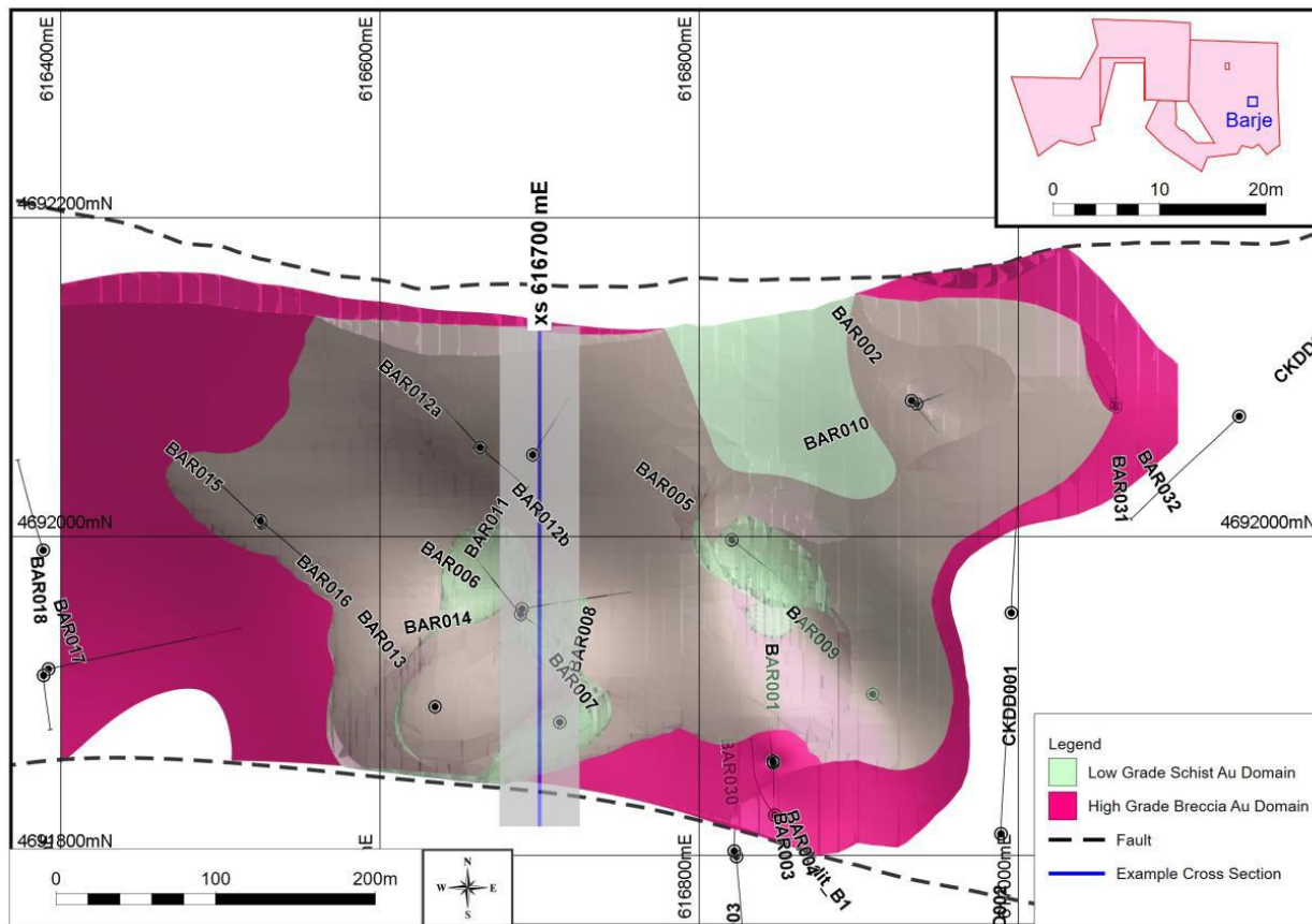
Figure 11: Plan view of mineralized wireframes used in resource estimation. Cross section line shown for 616700 mE.
