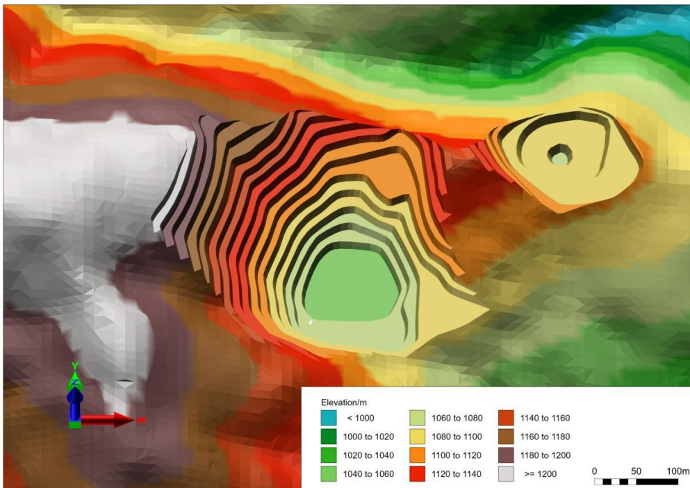
Figure 17: Development of Pit Stage Designs Pushback 3
