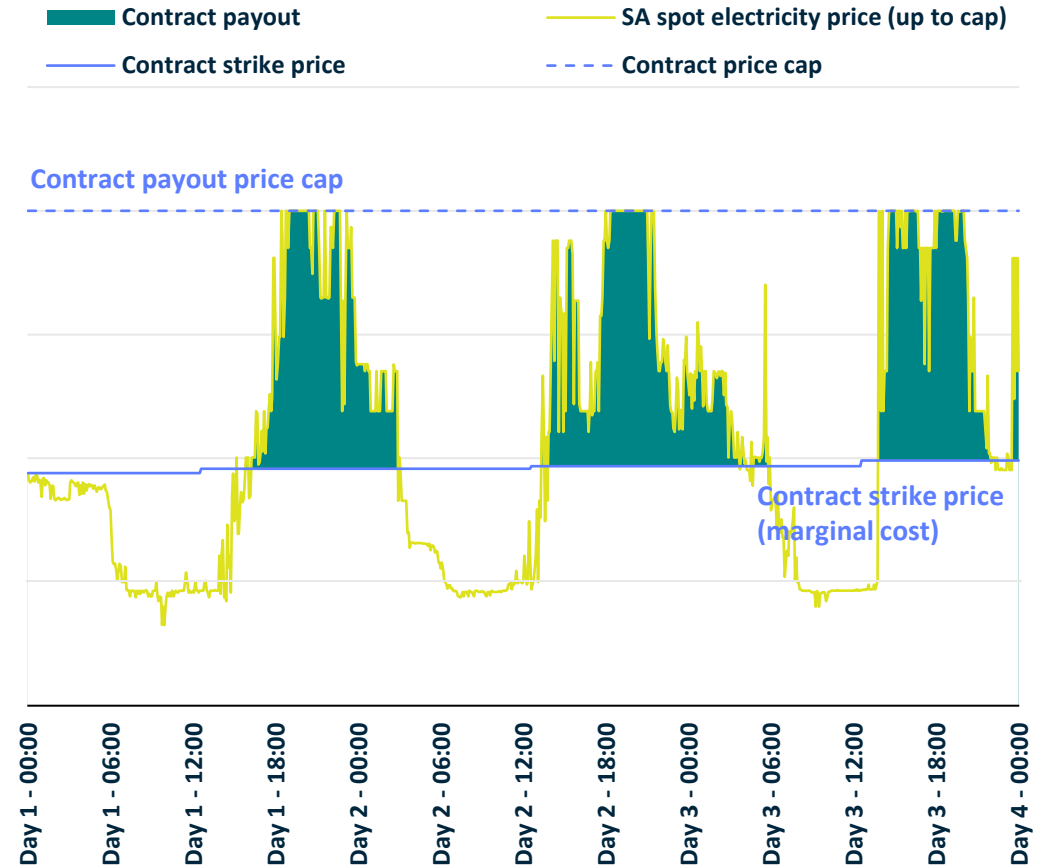
Spark spread contractual arrangement (illustrative)
