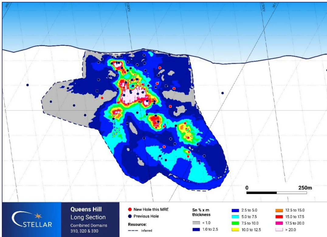
Figure 5: Queen Hill Domain Zones 310, 320 and 330 as % Sn x m thickness.
