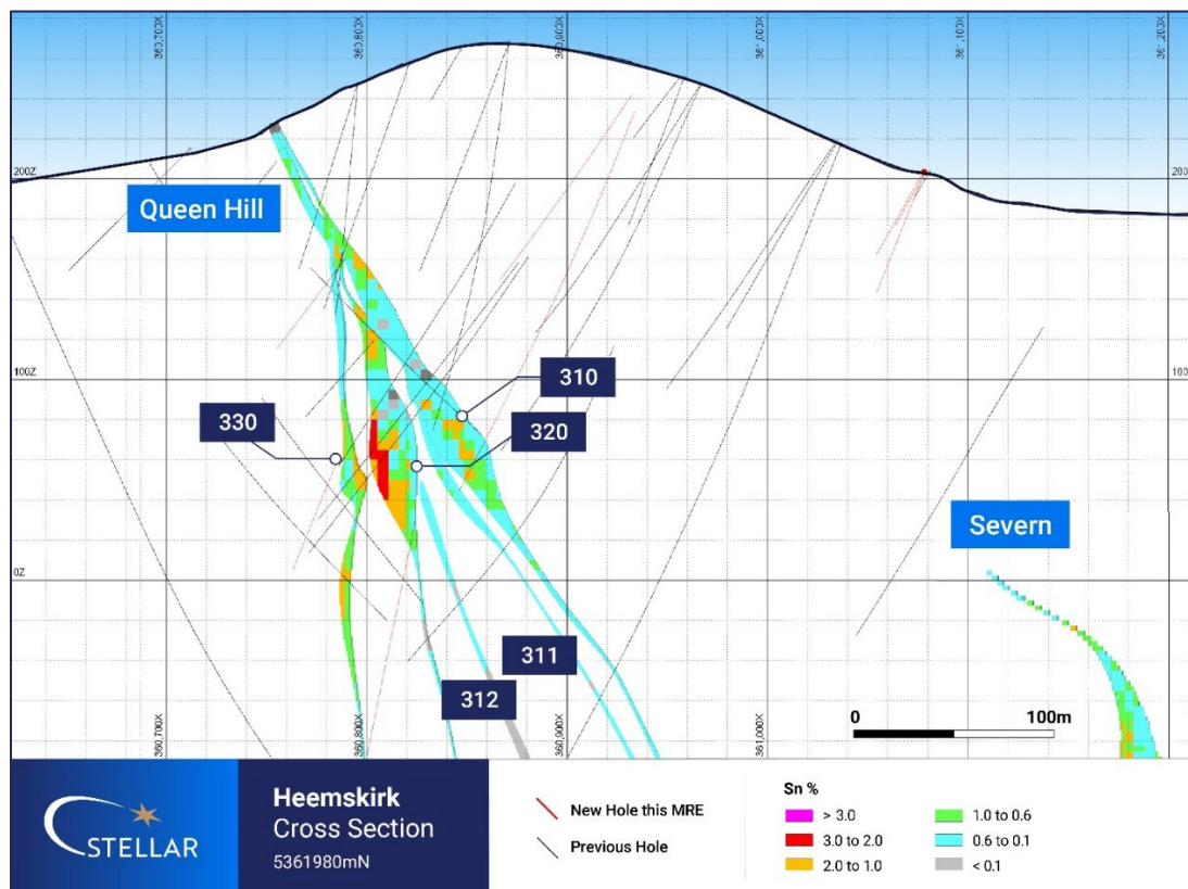
Figure 4: Section 5361980mN showing domains 310, 320 and 330 and % Sn content.
