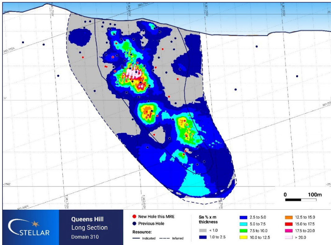
Figure 6: Queen Hill Main Upper Domain Zone 310 as % Sn x m thickness.
