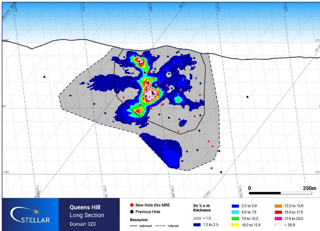
Figure 7: Queen Hill Middle Domain Zone 320 as % Sn x m thickness.
