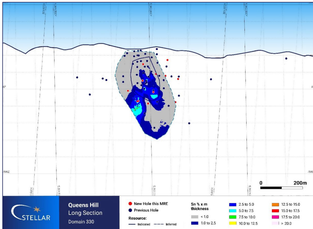
Figure 8: Queen Hill Lower Domain Zone 330 as % Sn x m thickness.
