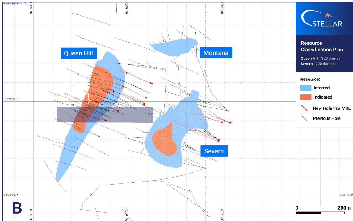
Figure 3: Resource classification for domain 320 at Queen Hill from 2026 MRE update, and resource domain 220 at Severn from 2023 MRE classification with location of cross section 5361980mN (grey rectangle)
