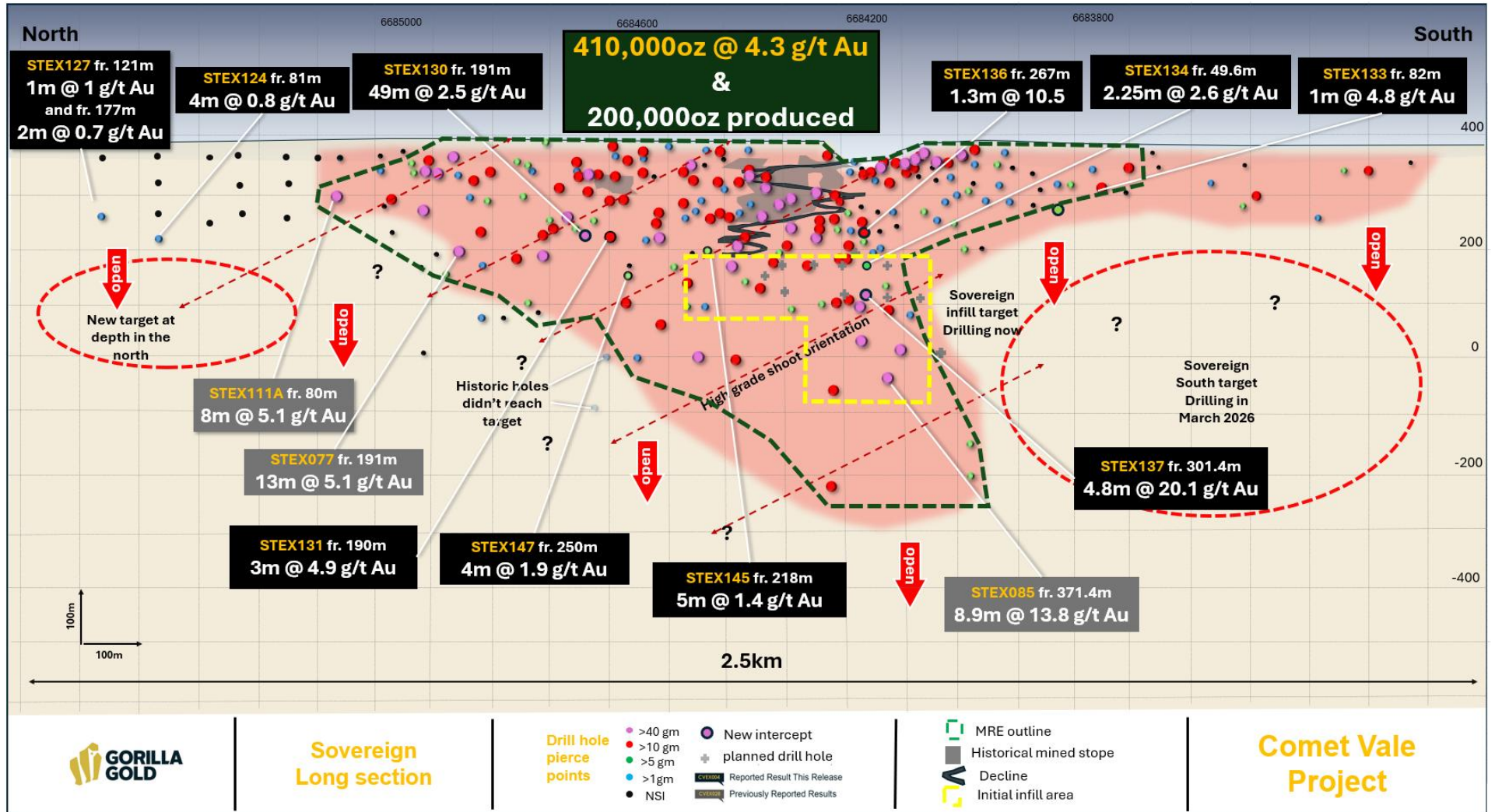
Figure 1. Sovereign Long Section
