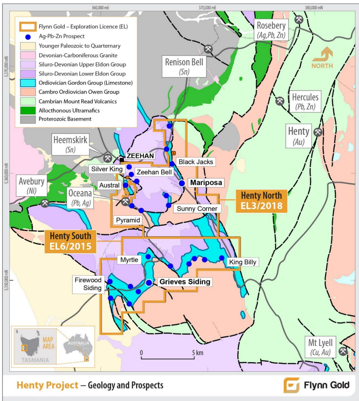
Figure 1 – Henty Project - Geology and Prospect Locations.
