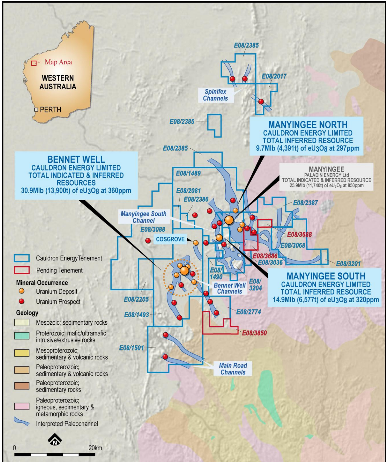
Figure 3. Regional Geological Map.
