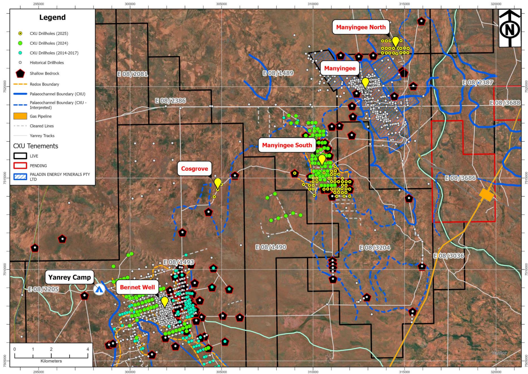
Figure 2. Map of the Yanrey region showing recent and historical drilling within interpreted Early Cretaceous palaeodrainage network.
