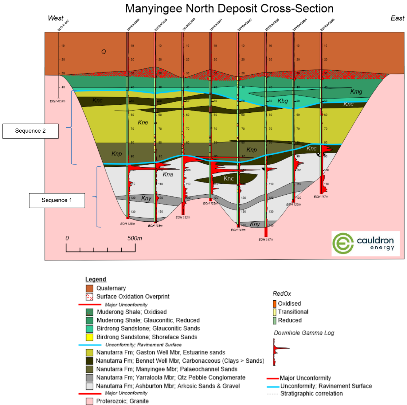
Figure 14. Manyingee North Cross-Section
