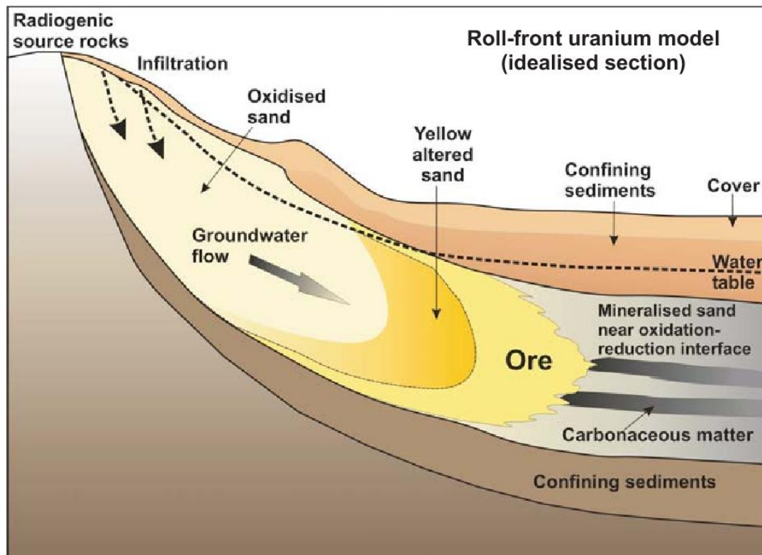
Figure 5. Uranium roll-front conceptual model.
