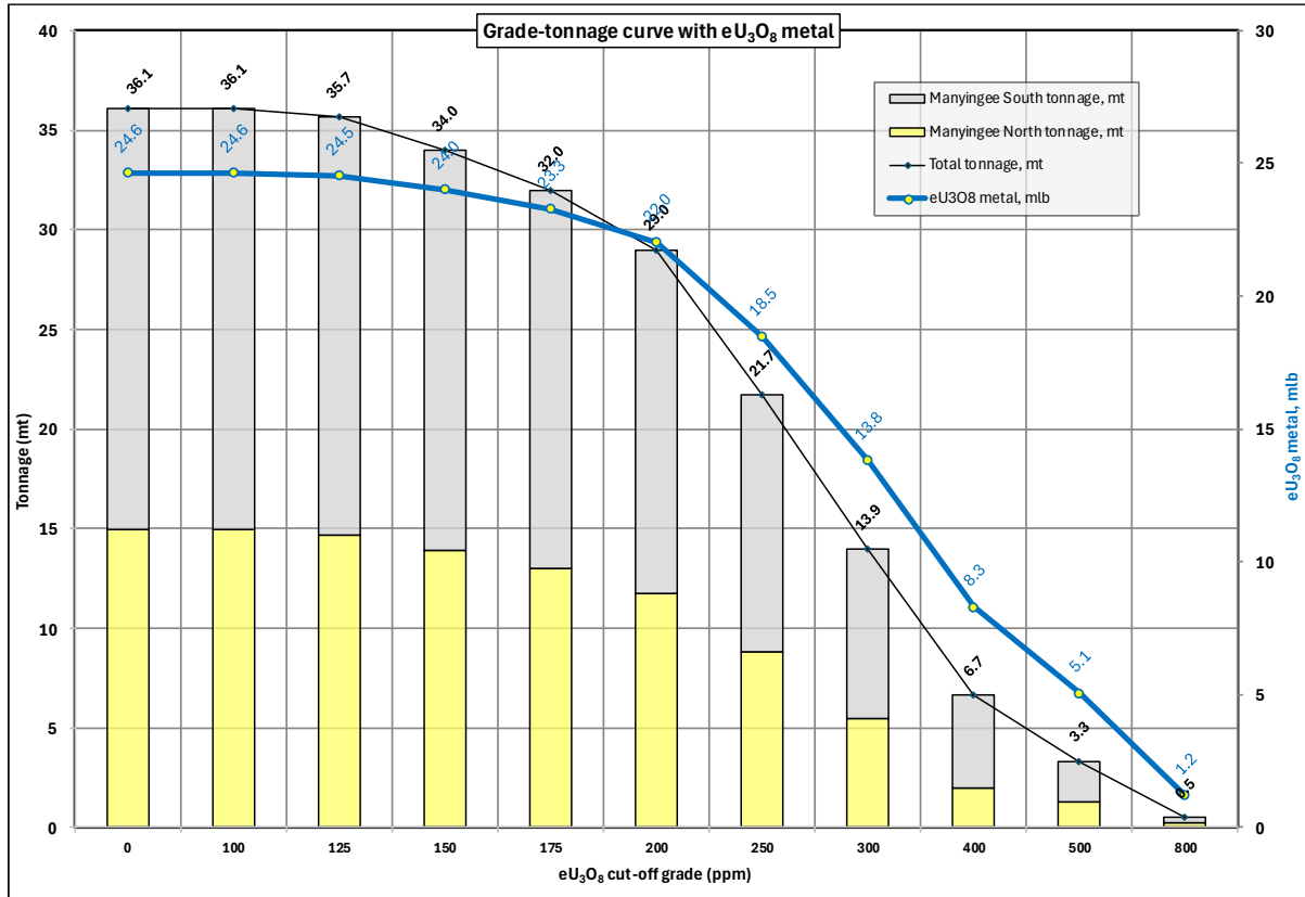
Figure B.2 Grade-tonnage curve with eU 3 O 8 metal
