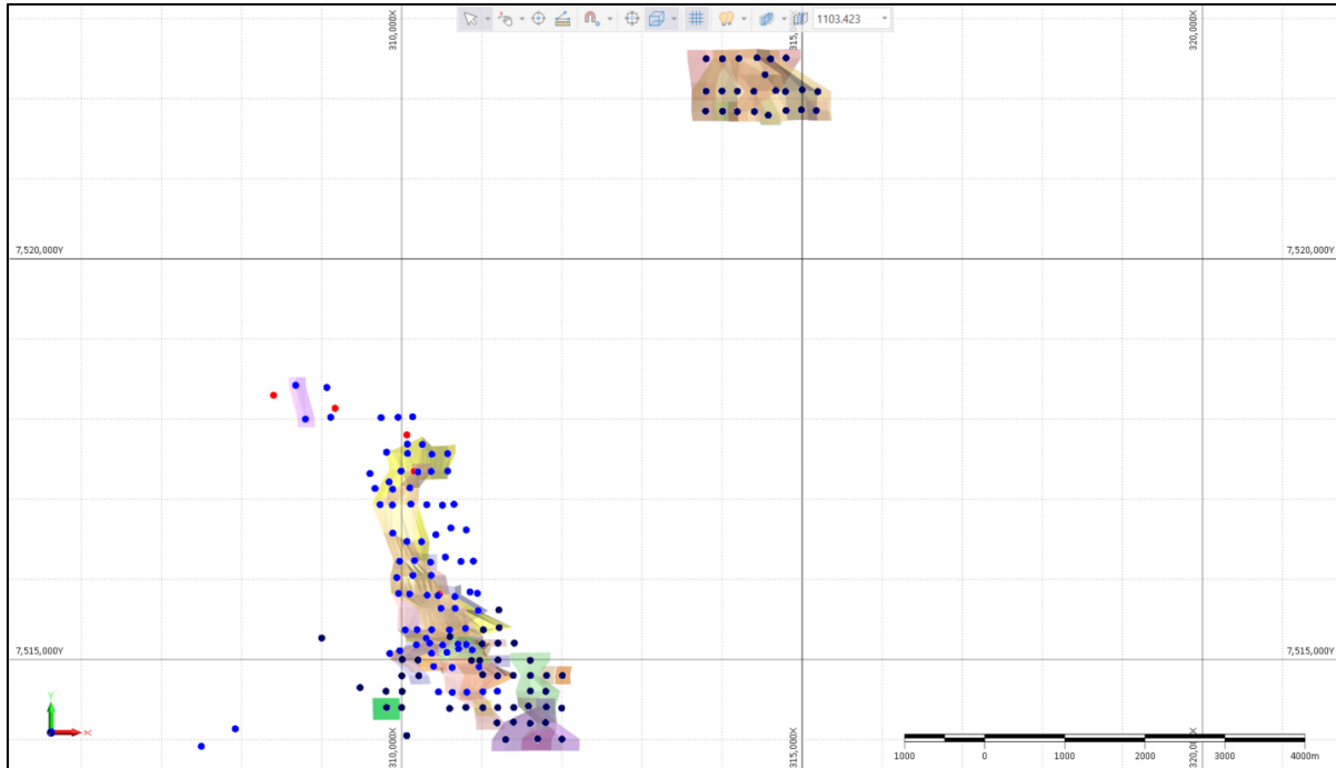
Figure 15. Exploration drilling density at Manyingee South and North deposits (plan view).
