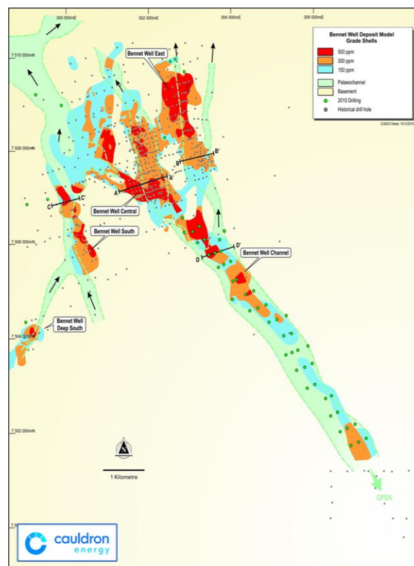
Figure C.1. Bennet Well Uranium Deposit and spatial distribution of U_3O_8 domains.
