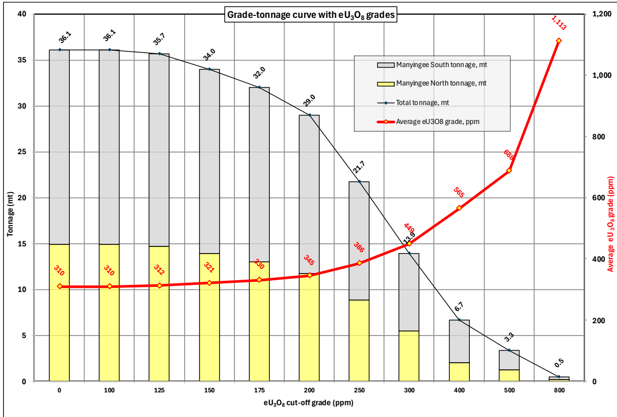
Figure B.1 Grade-tonnage curve with eU 3 O 8 grades
