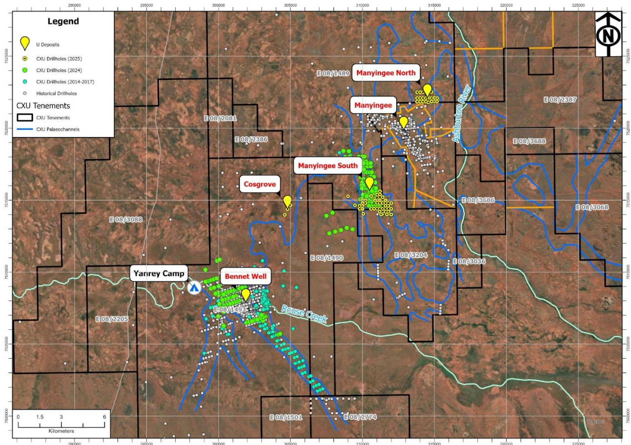
Figure 4. Uranium deposit location and Cauldron drilling activities within the Yanrey Project.
