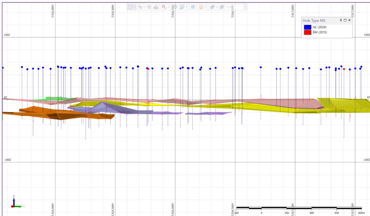
Figure 16. Orientation of drillholes (long section view, Manyingee South).
