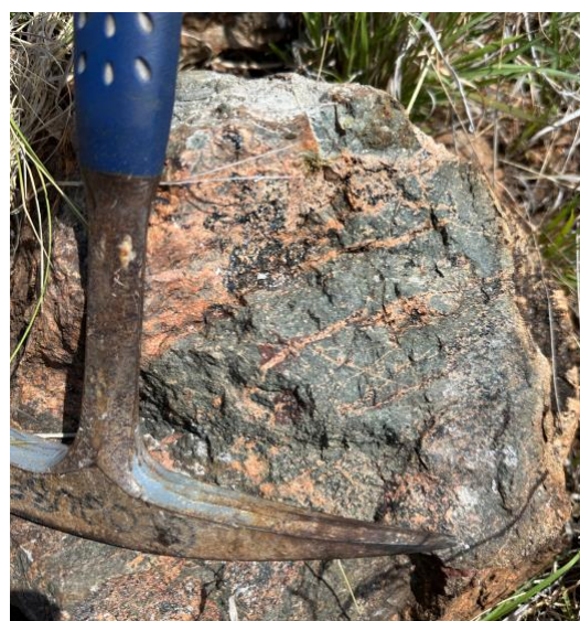
Propylitic alteration (at 217916mE, 7372419mN)
