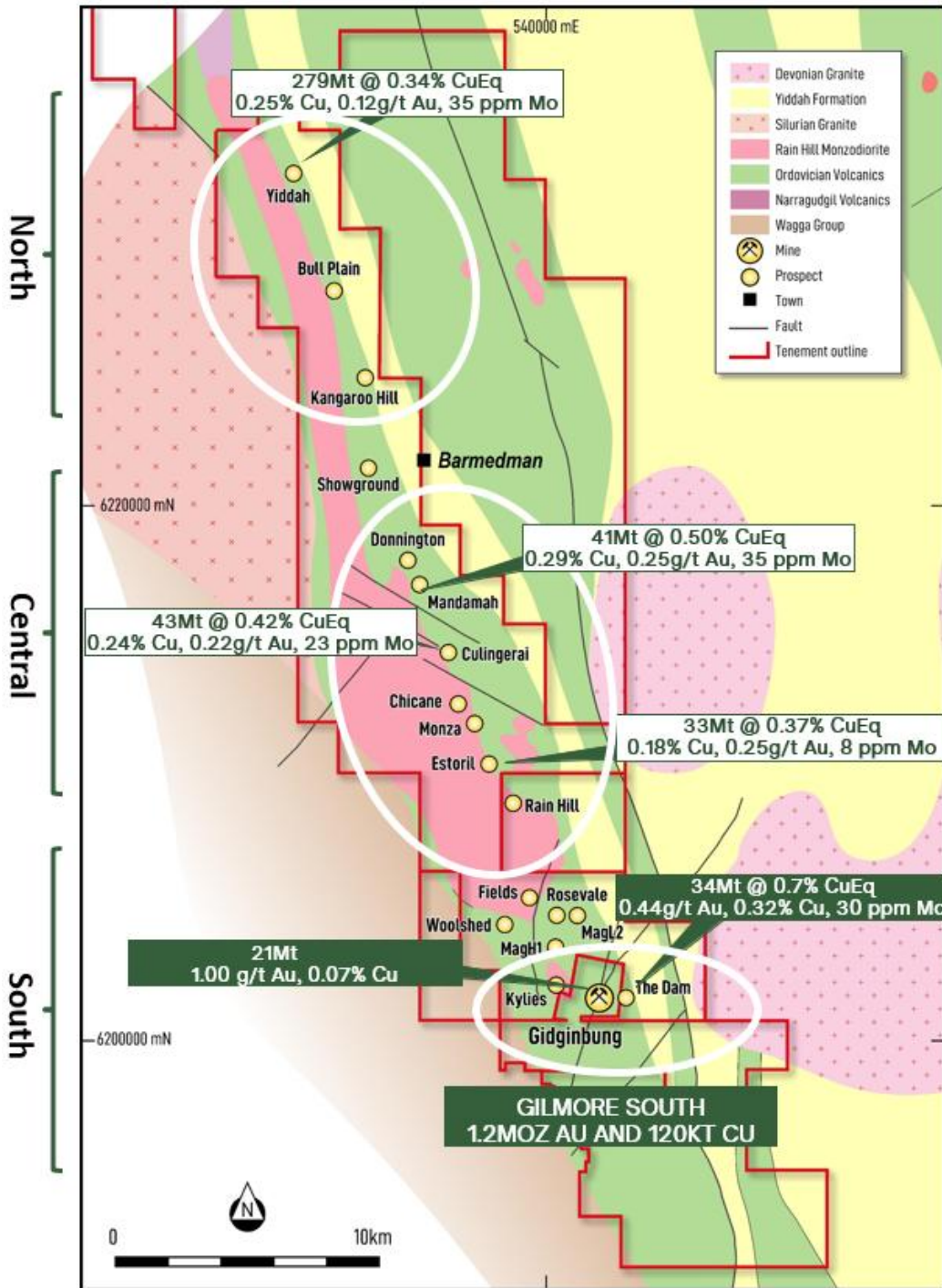
Figure 3: Plan View of the Gilmore Project highlighting the Southern, Central and Northern Zones.
