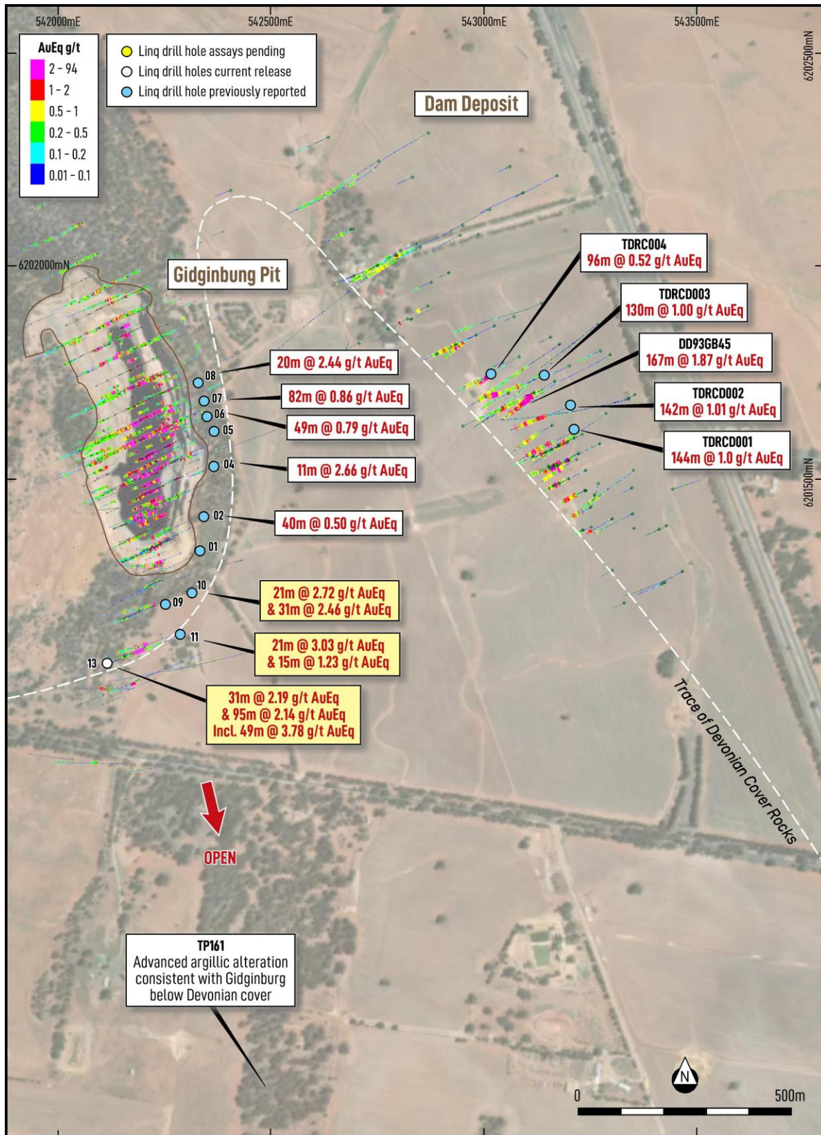
Figure 1: Southern Zone (Gidginbung/ Dam) plan image illustrating the location of Phase 1 drilling results.
