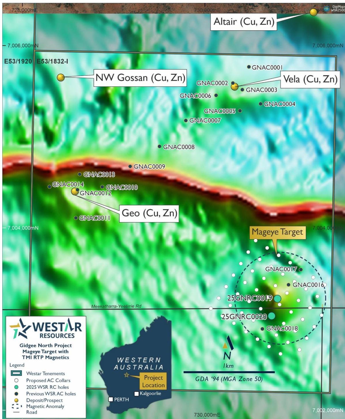
Figure 2. Airborne magnetic image (TMI, RTP) showing the magnetic high at the Mageeye prospect, previous WSR air core and reverse circulation holes, and planned air core holes.
