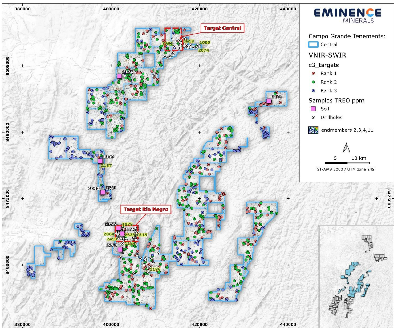
Figure 2: Central Block showing Sentinel - 2 VNIR - SWIR target ranking, interpreted endmember distribution and historical drill hole, soil and rock sample locations
