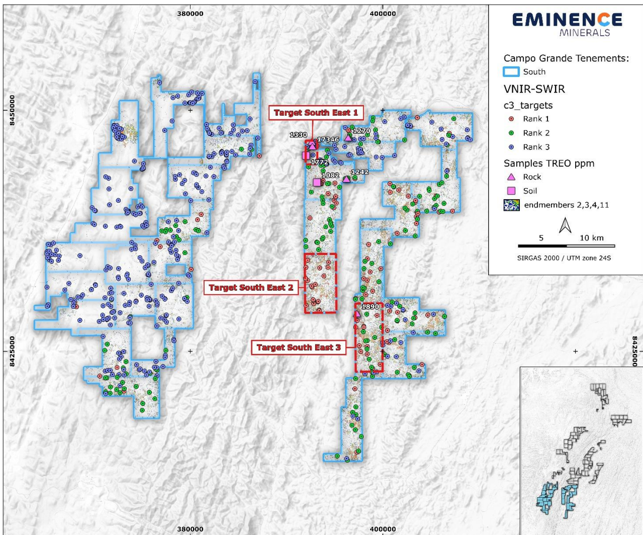
Figure 3: Southern Block showing Sentinel - 2 VNIR - SWIR target ranking, interpreted endmember distribution and soil and rock sample locations
