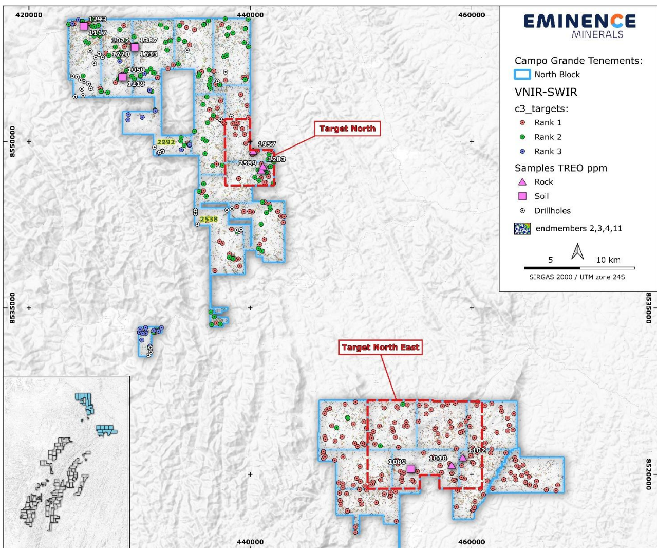
Figure 1: Northern Block showing Sentinel - 2 VNIR - SWIR target ranking, interpreted endmember distribution and historical drill hole, soil and rock sample locations
