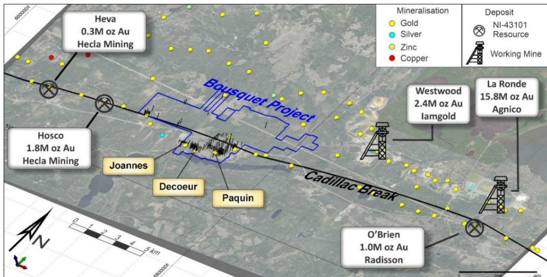
Figure 8: Setting of the Bousquet Project relative to working mines and mineral resources along the Cadillac Break
