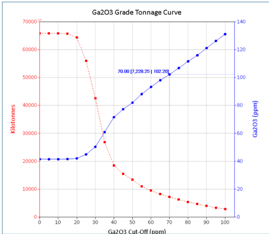
Figure 3 - Grade Tonnage Curve
