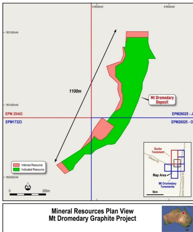
Figure 19: Mt Dromedary Deposit - Indicated and Inferred Mineral Resources Plan View
