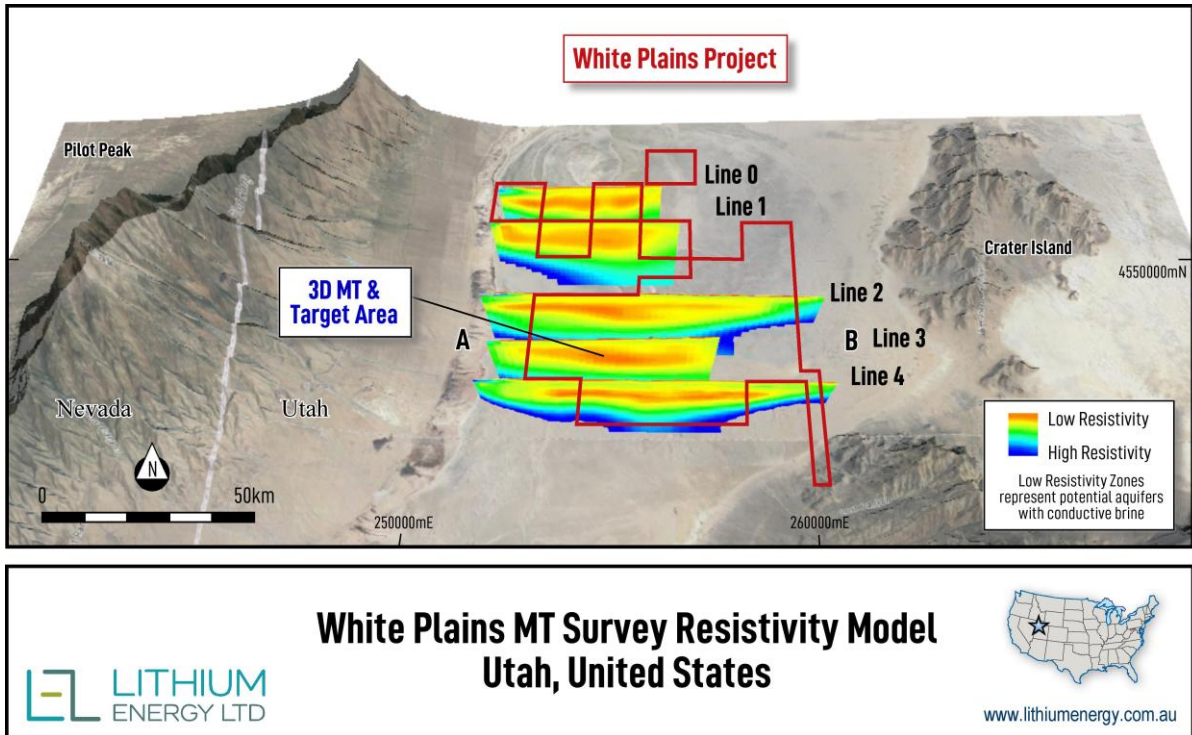
Figure 15: 3D resistivity cross sections from 5 MT survey lines within the White Plains claims area (shown in red)
