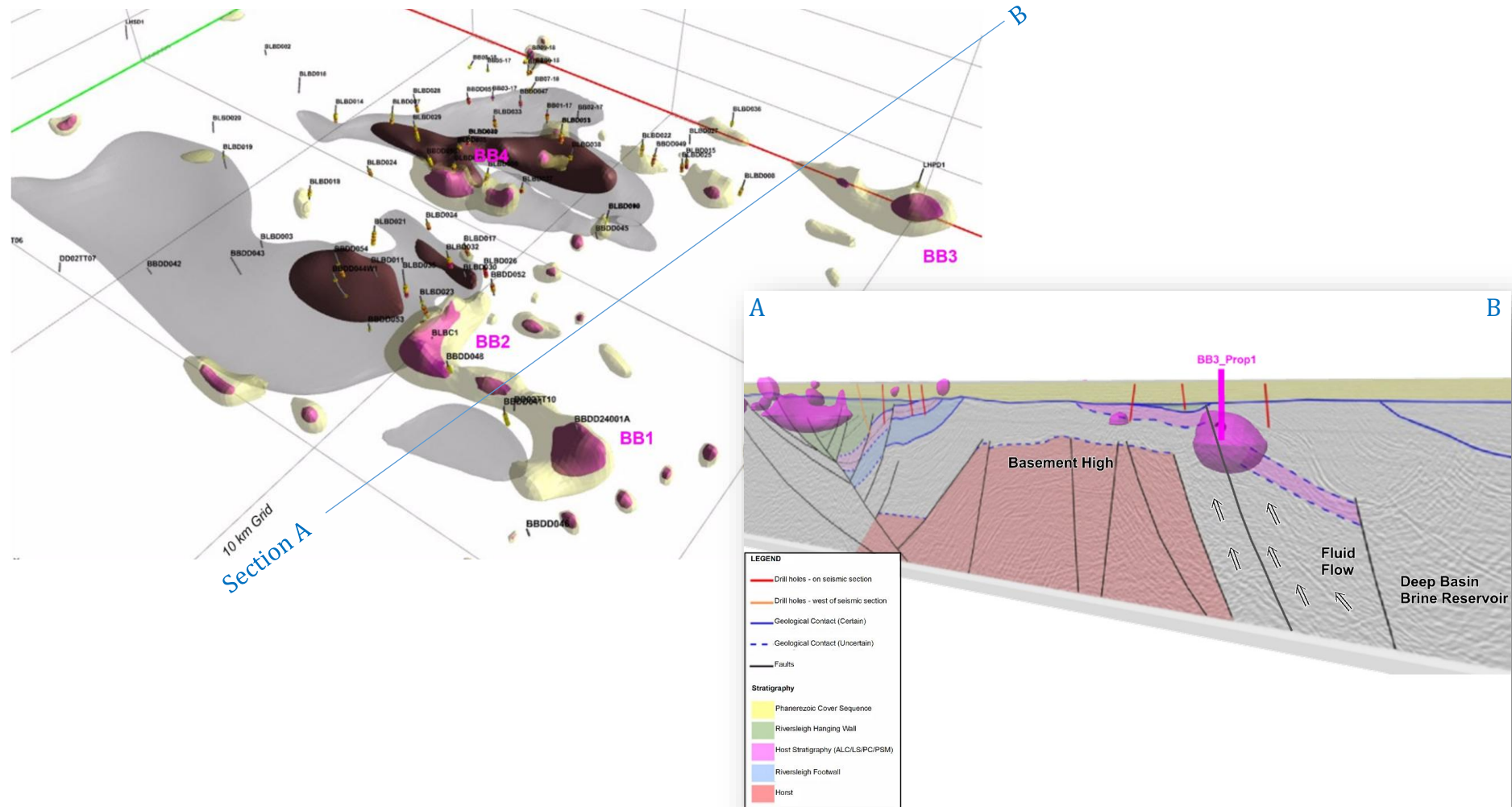
[Figure 11] Lawn Hill Project, Bluebush Prospect: Top left is an oblique 3D view facing northwest showing historic drilling, high gravity shells (pink-yellow) and high-magnetic shells (brown-grey) from 3D modelling and the previously untested, high-priority, geophysical targets labelled BB1, BB2, BB3 and BB4, and Red Metal’s recent drill hole BBDD24001A on target BB1 (refer Red Metal ASX announcement dated 17 March 2025). Bottom left is a section view down the anticlinal axis showing interpreted seismic section (Teck line BB_SL01) with high density gravity inversion shells (pink). Note the location of the BB3 high-gravity target along the faulted margin to a regional basement high (or anticline) along which metal-enriched, deeper basin brines may have been focused. Potential for the discovery of dense, stratabound or breccia style copper-silver, silver-lead-zinc, and/or iron sulphide mineralisation associated with weakly magnetic pyrrhotite or magnetite is speculated.
