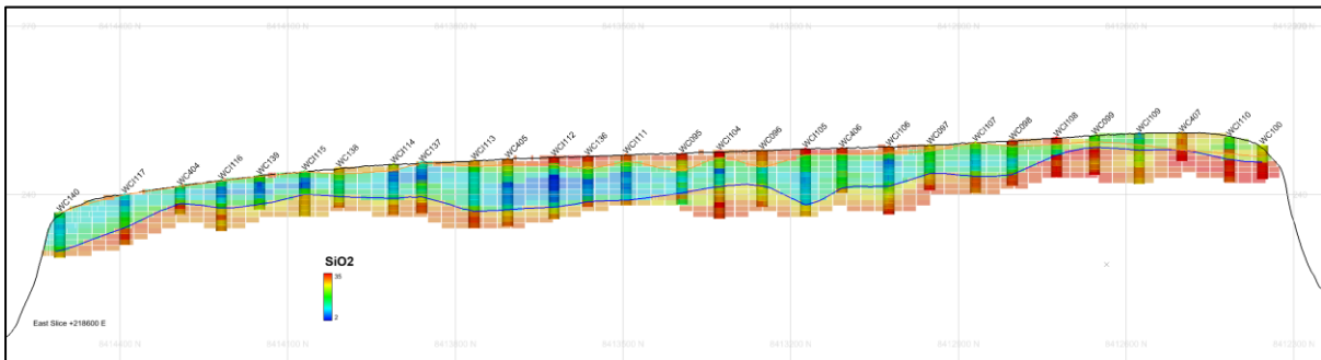
Figure 6: Example section (E 218,600) plot comparing sample and model SiO 2 grades - Plateau C
