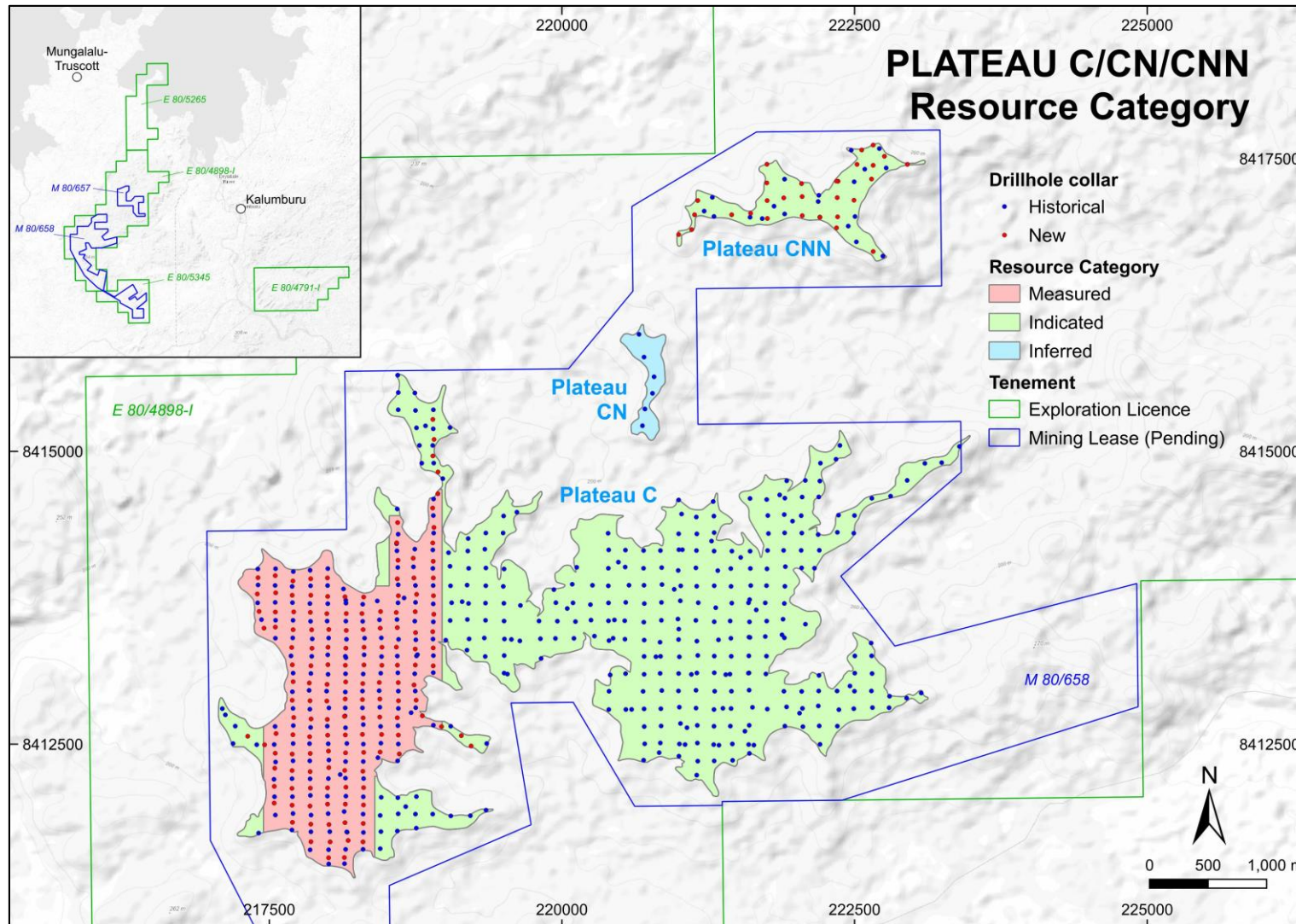
Figure 10: Wudagu C (including CN and CNN) Resource Classification
