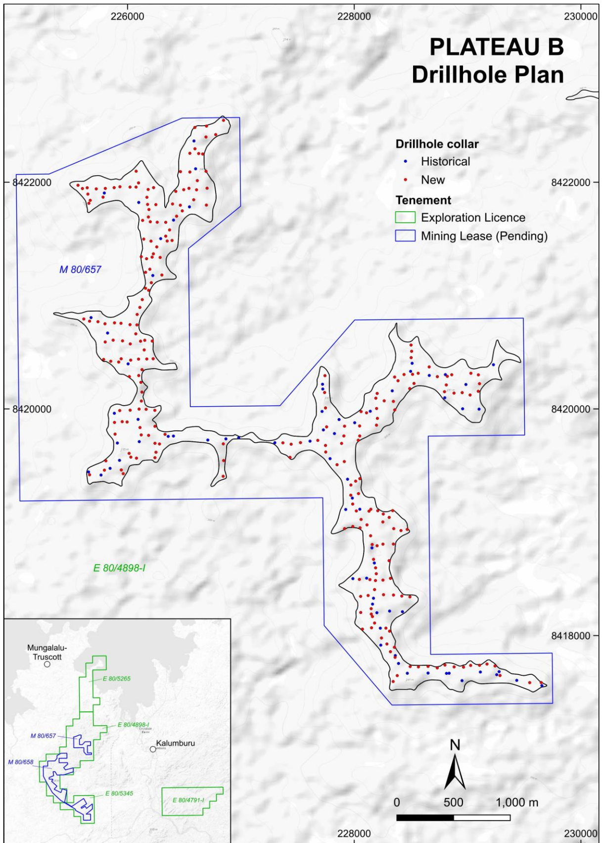
Figure 2: Wudagu B Drillhole Plan
