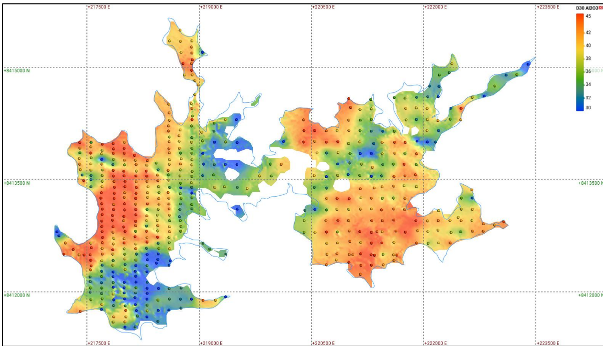
Figure 7: Example plan plot (Plateau C) - Domain 30 Al 2 O 3
