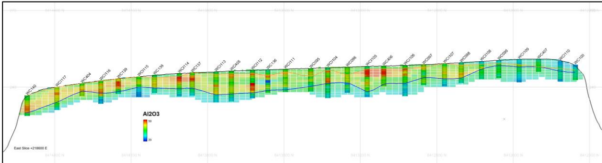
Figure 5: Example section (E 218,600) plot comparing sample and model Al 2 O 3 grades - Plateau C
