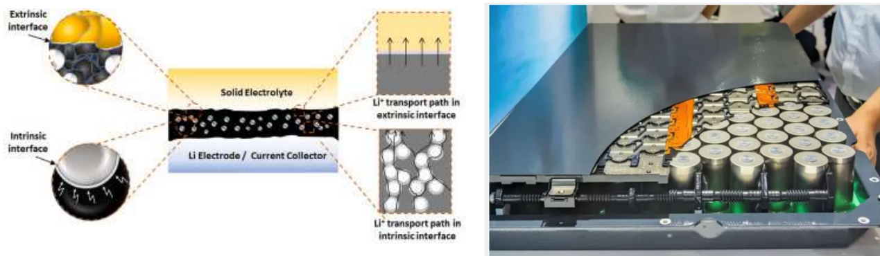
Samsung SDI solid state technology uses silver at the anode as Ag-C to prevent dendrite formation
