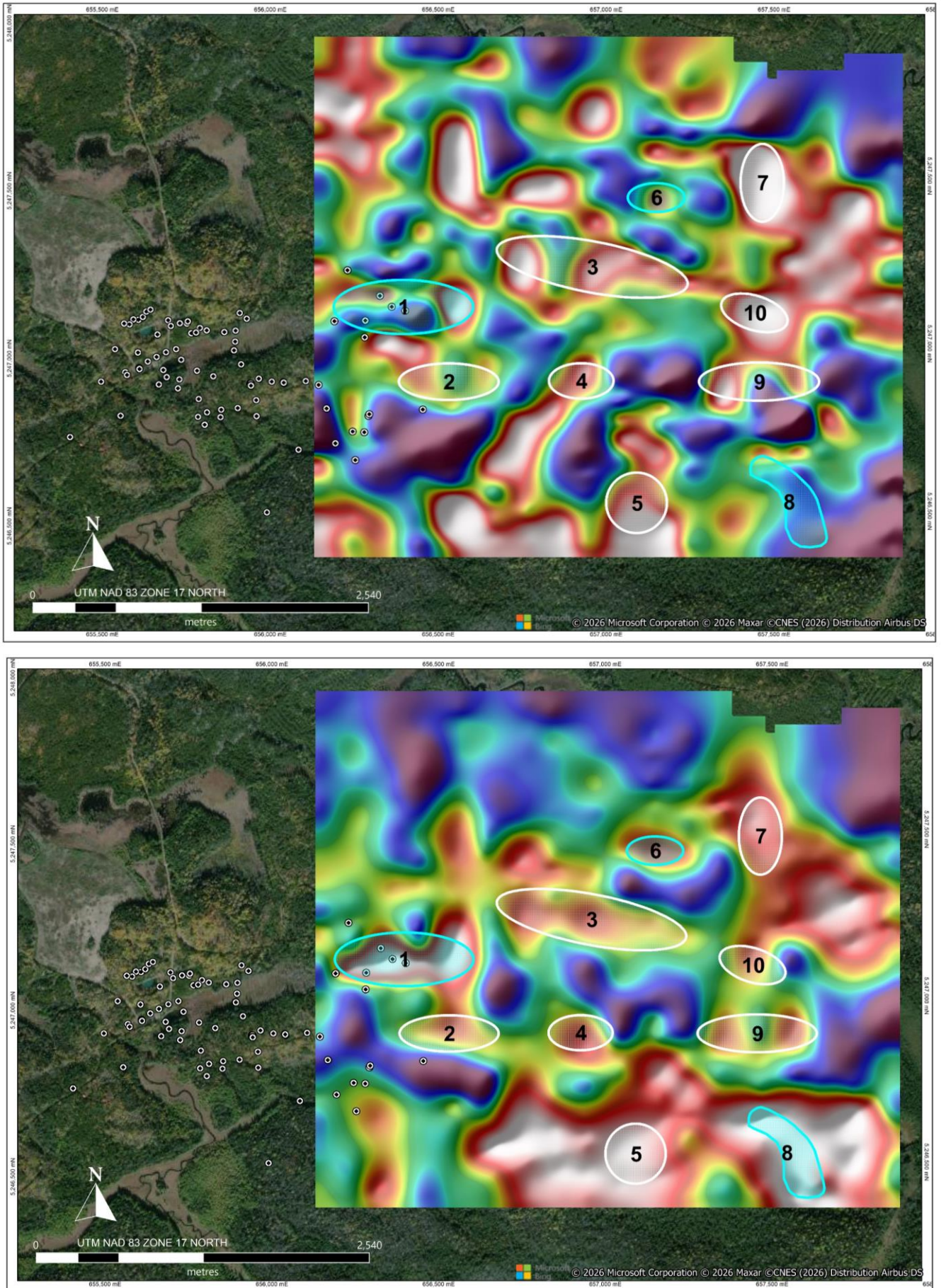
Figure 7: IP survey results showing 70m depth slice resistivity (upper) and chargeability (lower).
