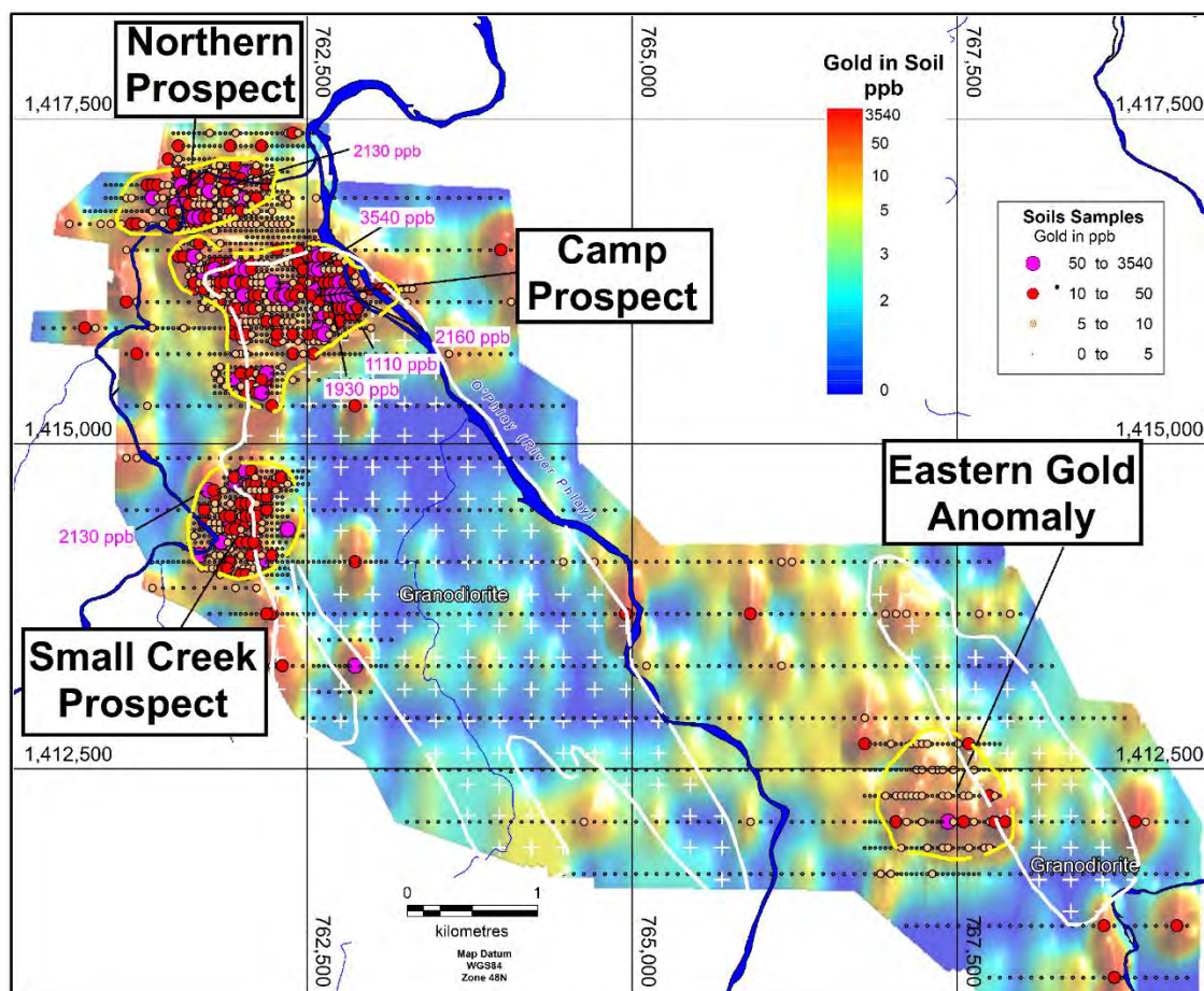
Figure 14. Soil sample locations and gold results at O'Phlay Gold Project over the imaged gold-in-soil assay data (inverse distance method).
