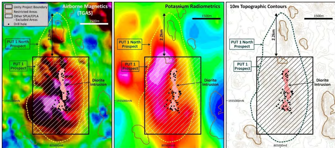
Figure 18. Potential extension to the PUT 1 Copper-Gold Deposit into Unity Metals' adjacent PUT 1 North area shown on Total Gradient-Analytical Signal (TGAS) magnetics, potassium (K) radiometrics and topographic contours.
