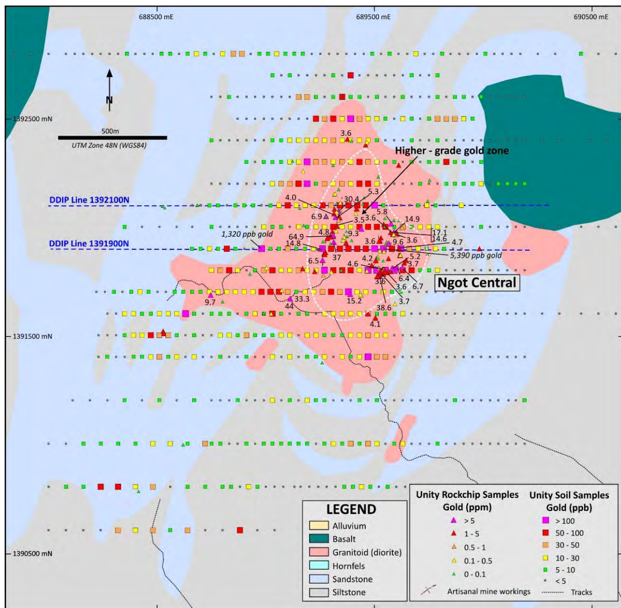
Figure 6. Ngot Central Prospect. Soil and rock chip gold results on a geological interpretation.
