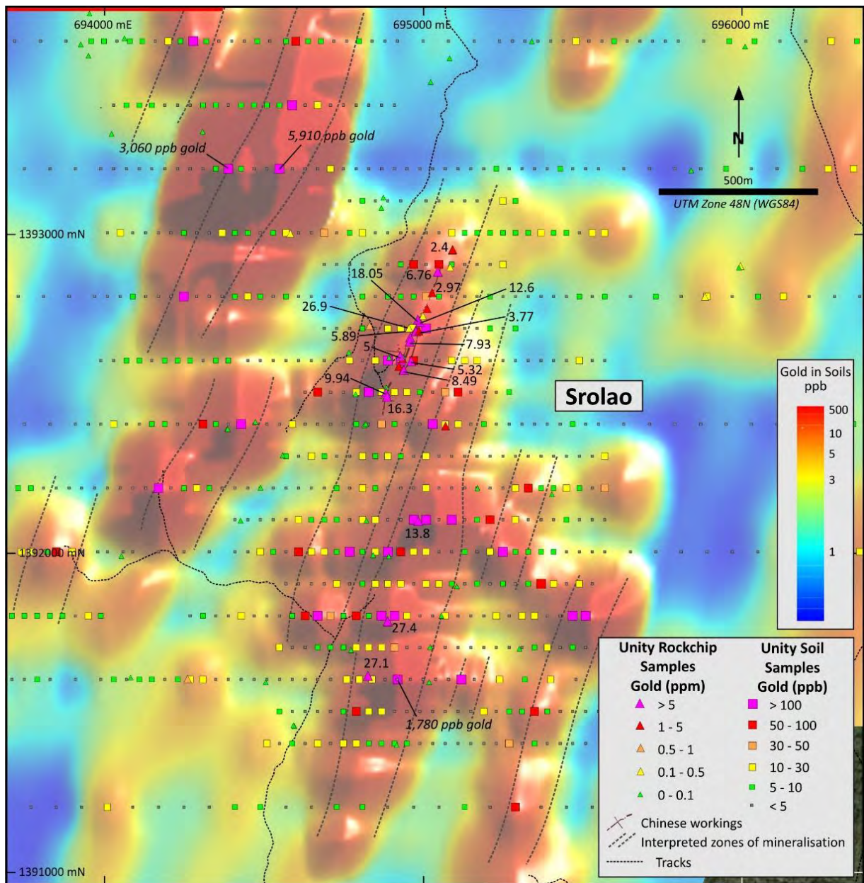
Figure 11. Srolao Gold Prospect. Soil and rock chip sample results on gridded gold-in-soil image.
