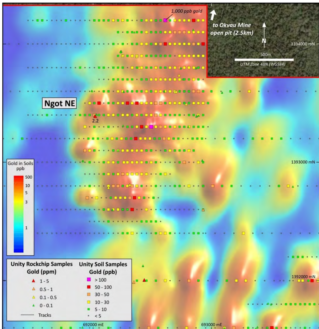
Figure 10. Ngot NE Prospect. Soil and rock chip sample results on gridded gold-in-soil image.
