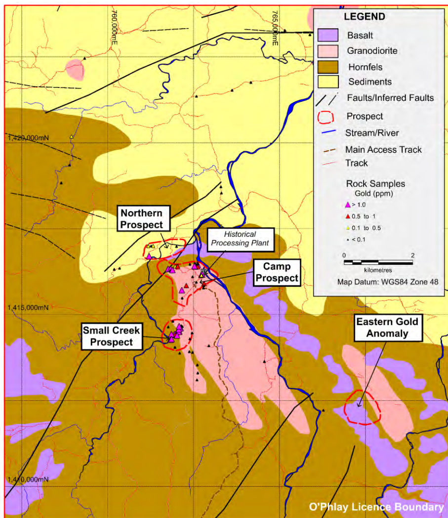
Figure 13. O'Phlay Licence. Rock chip sample gold results on interpreted geology.
