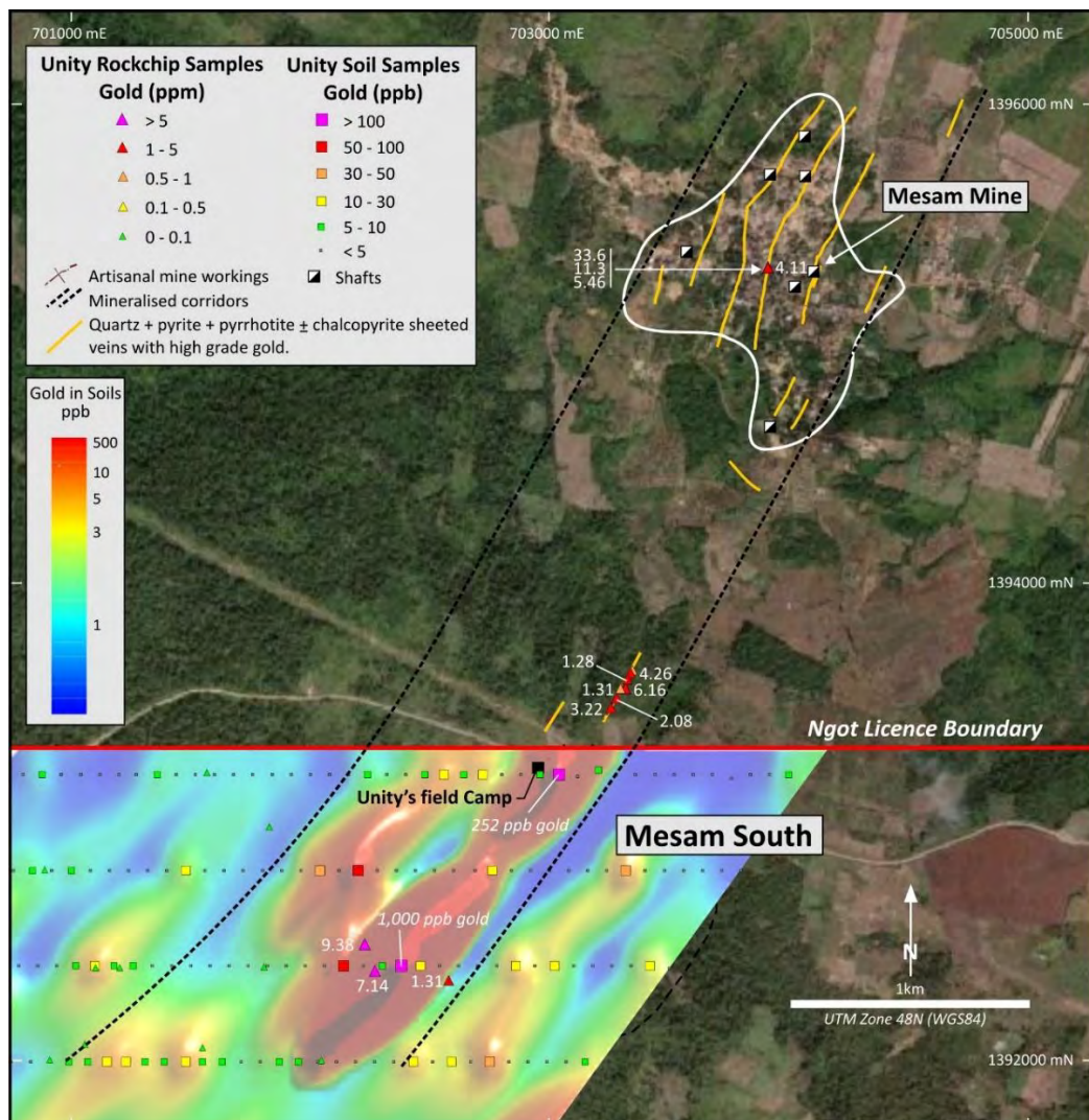
Figure 12. Mesam South Prospect. Soil and rock chip sample results on gridded gold-in-soil image.
