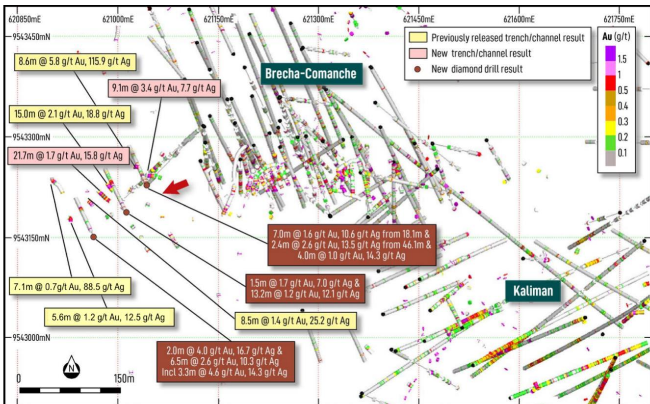
Figure 2. Plan view displaying the Brecha-Comanche and Kaliman targets, drill traces coloured by Au g/t, trench/ channel and drill significant intercepts. Note extensive porphyry hosted mineralisation defined at Kaliman which remains open.
