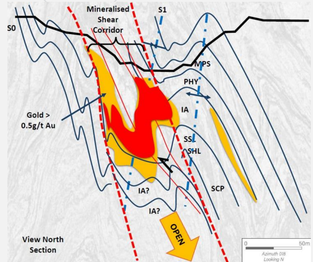
Schematic Structural Geology cross section looking north for the southern portion of the London Victoria Pit; demonstrating a parasitic fold on the east dipping limb of a larger anticlinal fold (preliminary interpretation pending further structural studies) Red > 1.0g/t Au, Yellow = 0.5 - 1.0g/t Au
