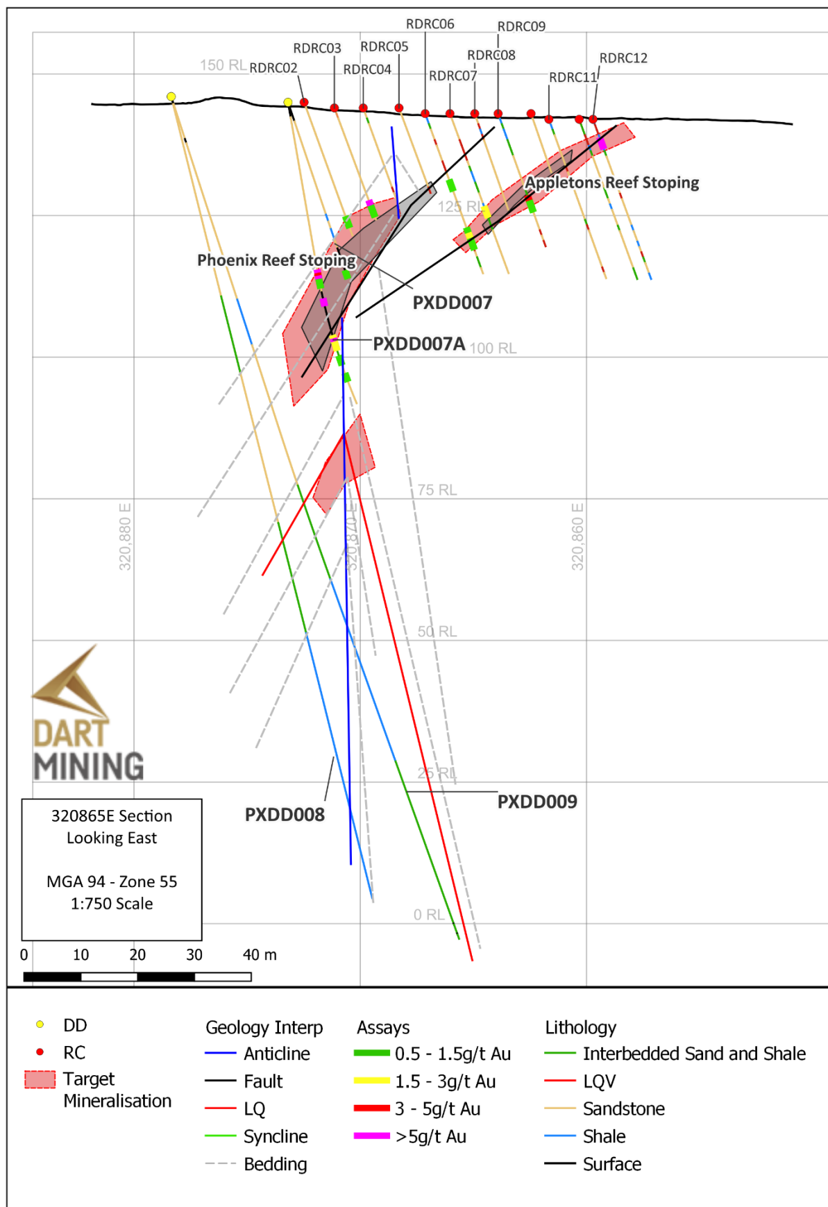
Figure 3: 320865E section showing PXDD007, PXDD007A, PXDD008 & PXDD009 with geological interpretation highlighting fold closure offset and prospective zones of mineralisation.
