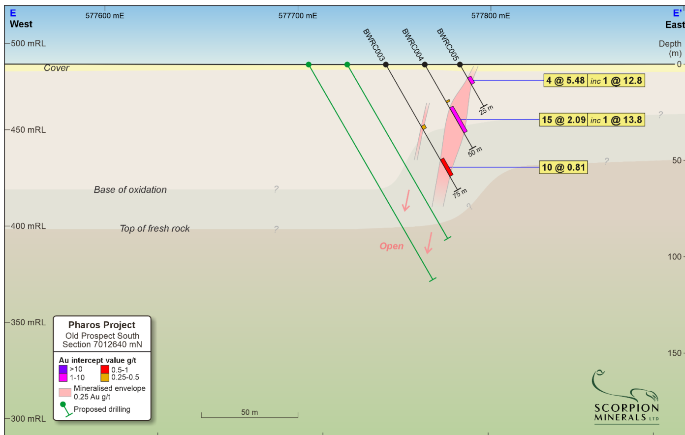
Figure 9: Old Prospect South Section E – E'
