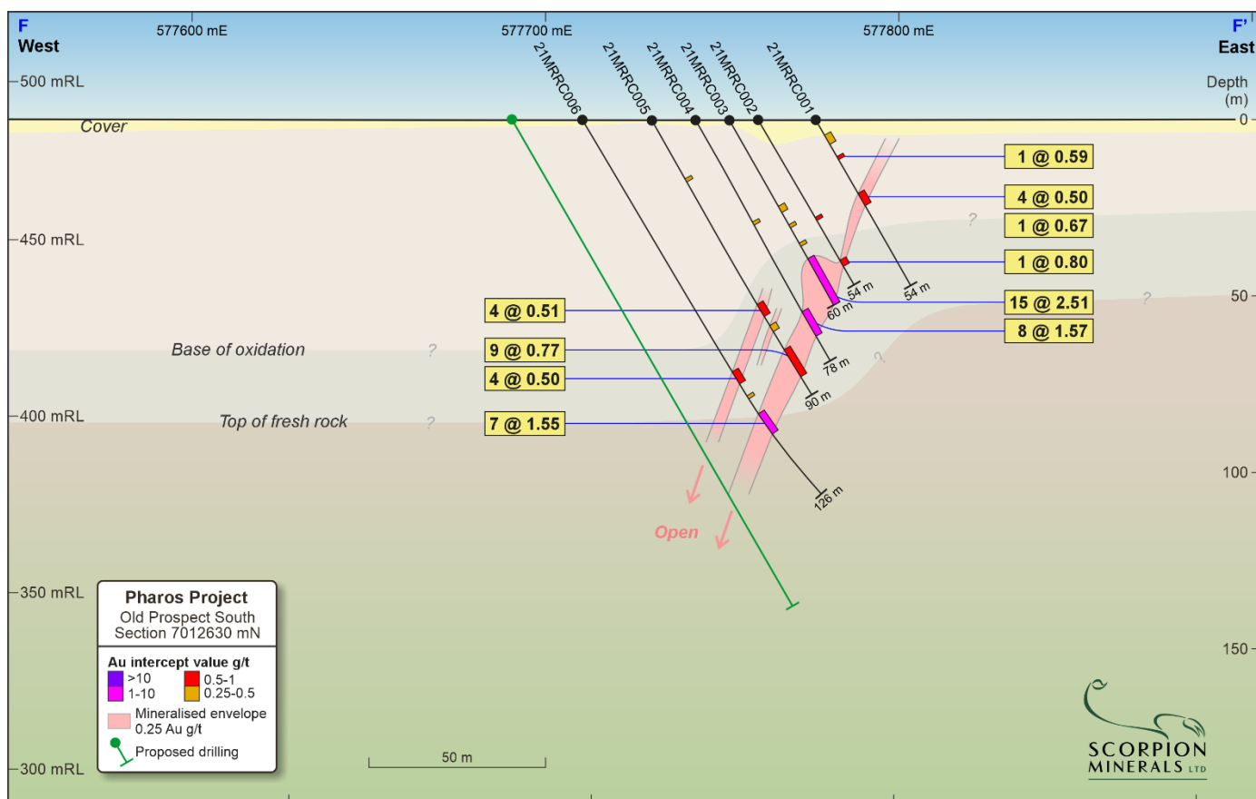
Figure 10: Old Prospect South Section F – F'
