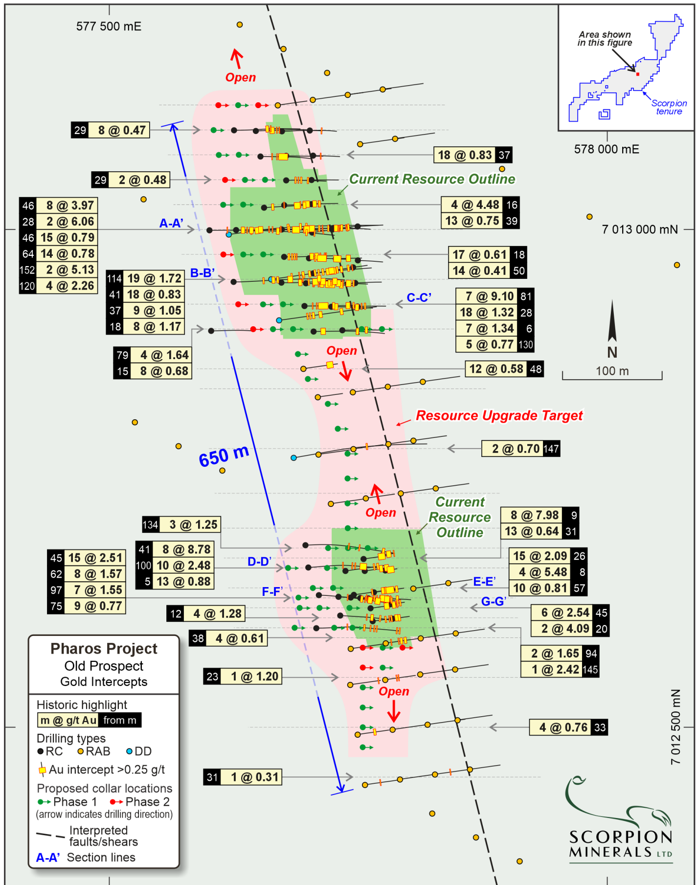
Figure 4: Old Prospect significant intercepts plan
