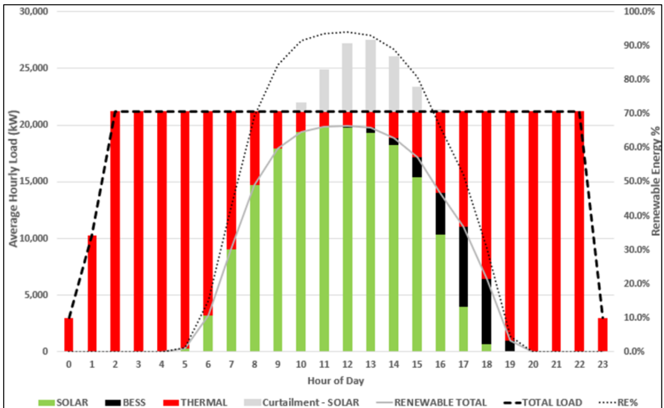
Figure 17 – Power Balance
