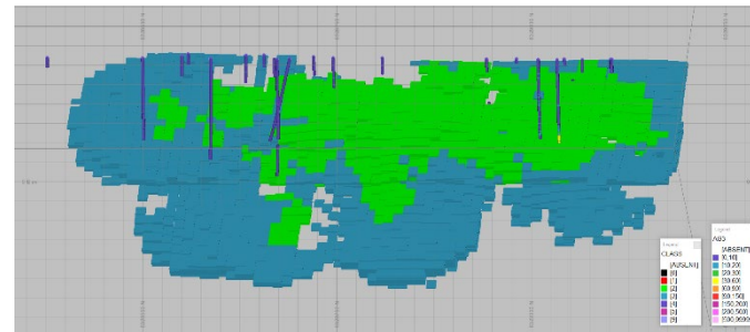
Figure 10: Long section (above) Drill holes with pXRF intervals (blue cylinders) and MRE coloured by Green – Indicated; Blue – Inferred, and looking up dip of mineralisation from below (below). None of the pXRF intervals are inside the MRE
