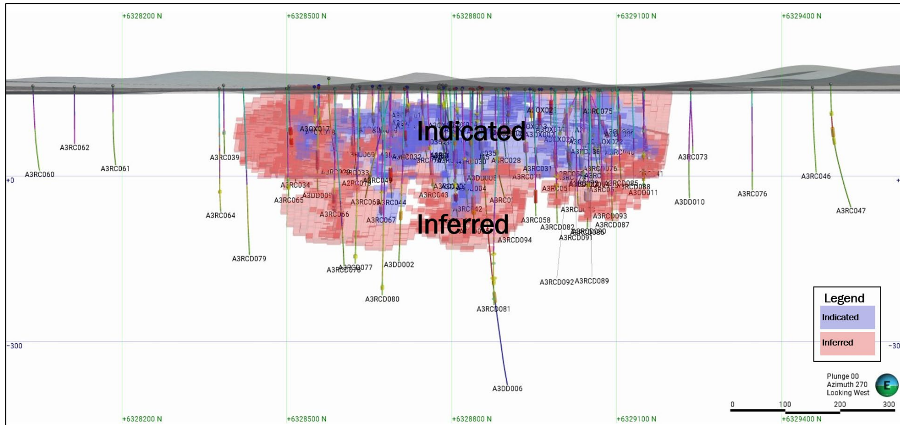
Figure 2: Long section drill holes locations with the block model coloured by resource classification showing distribution of Indicated (blue) to Inferred (pink).
