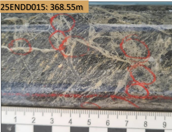
Photo 3. Visible gold (circled red) in hole 25ENDD015 at 368.55m down hole in pyrite-quartz+/-silver sulphosalts-arsenian pyrite-iron carbonate veins within moderately phyllic altered granite host rock. Scale bar units are centimetres.
