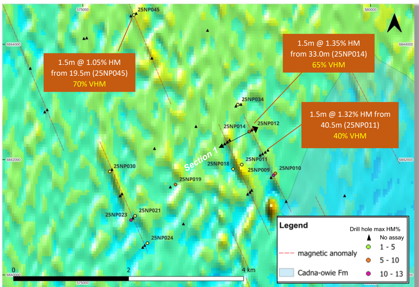
Figure 5. Max HM% results in Nilpinna Priority 1 area (TMI RTP background)
