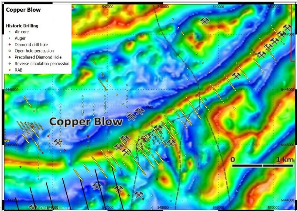
Figure 4 Copper Blow magnetics with historic drilling.
