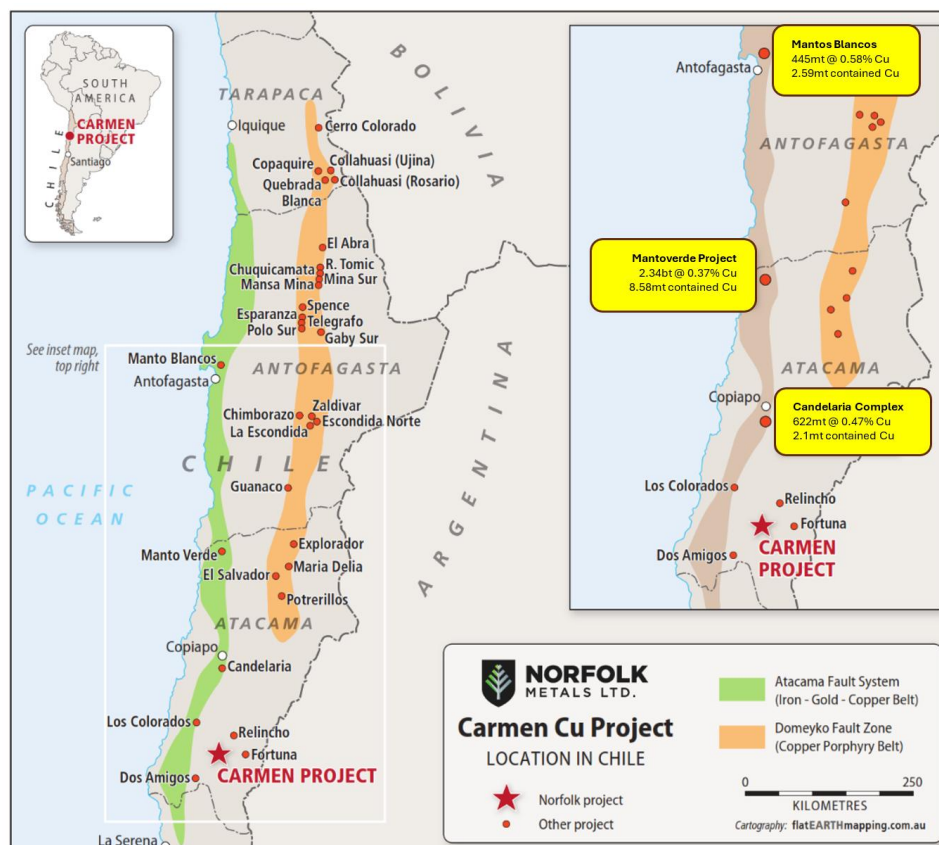
Figure 3: Carmen Cu Project Location in Huasco Province of Atacama Region in northern Chile (See Annexure A for resource references in Figure 1)
