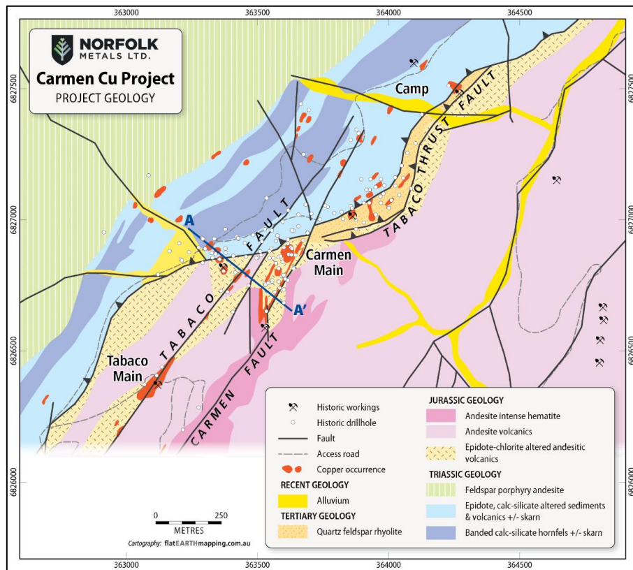
Figure 6: Carmen Cu Project Local Geology
