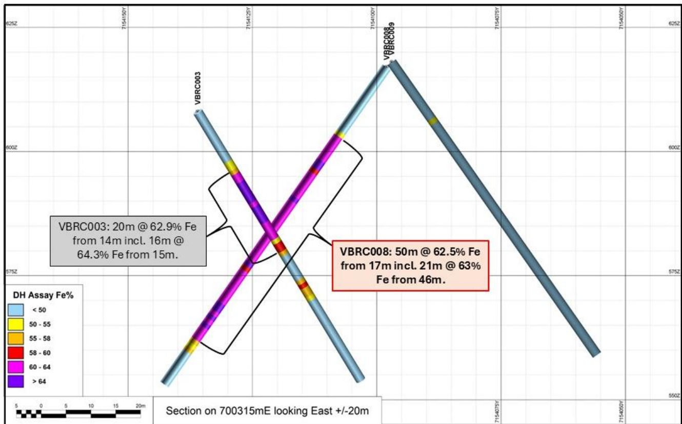
Figure 3: Section 700315mE looking east (new intercept in red) 1
