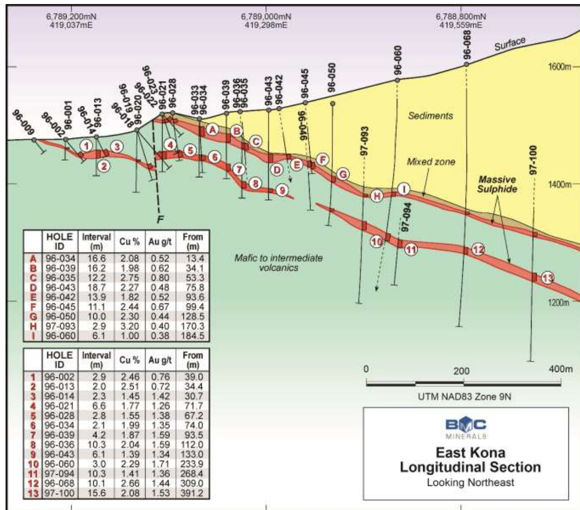
Figure 7-12: Longitudinal section of the East Kona Zone showing significant intersections. View is to northeast; letters A to I reference upper lens intersections, and numbers 1 to 13 reference lower lens drill intersections of massive sulphide, with corresponding analytical results tabulated.
