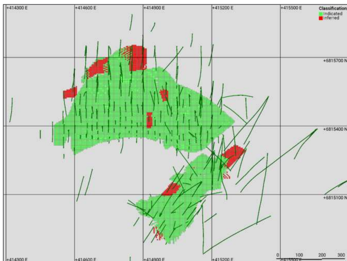
Figure 7-8: ABM Deposit Mineral Resource classification in plan view (red = Inferred, green = Indicated).
