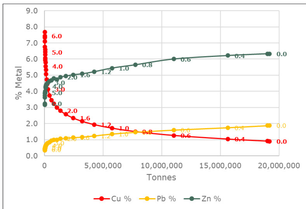
Figure 7-9: ABM Deposit global grade-tonnage curves for Cu%, Pb%, and Zn%. Source: Cube
