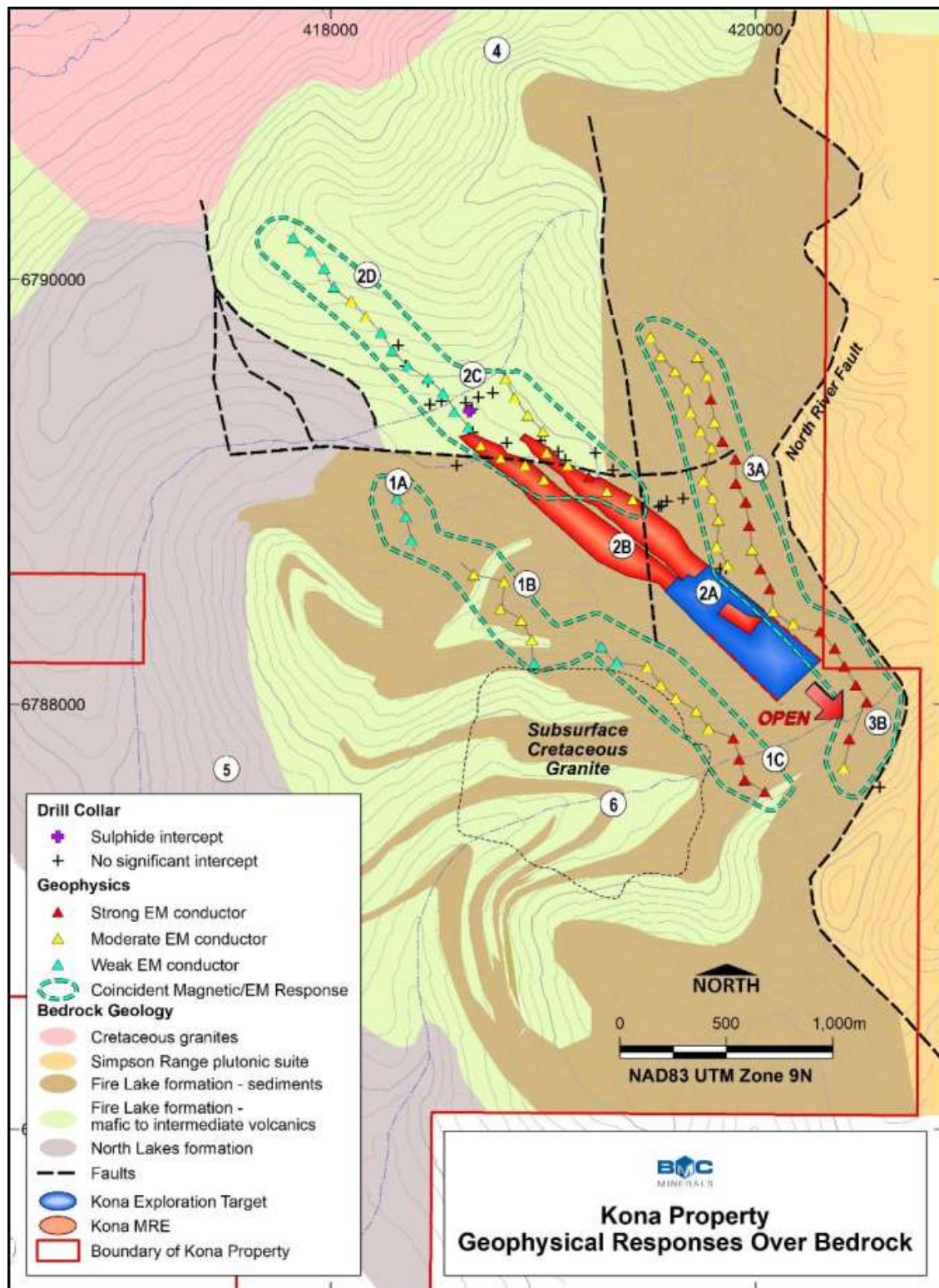
Figure 16-16: Exploration targets of the Kona Property; (Interpreted bedrock geology with mineralisation outline and conductive electromagnetic response trends from VTEM™ both projected to surface)
