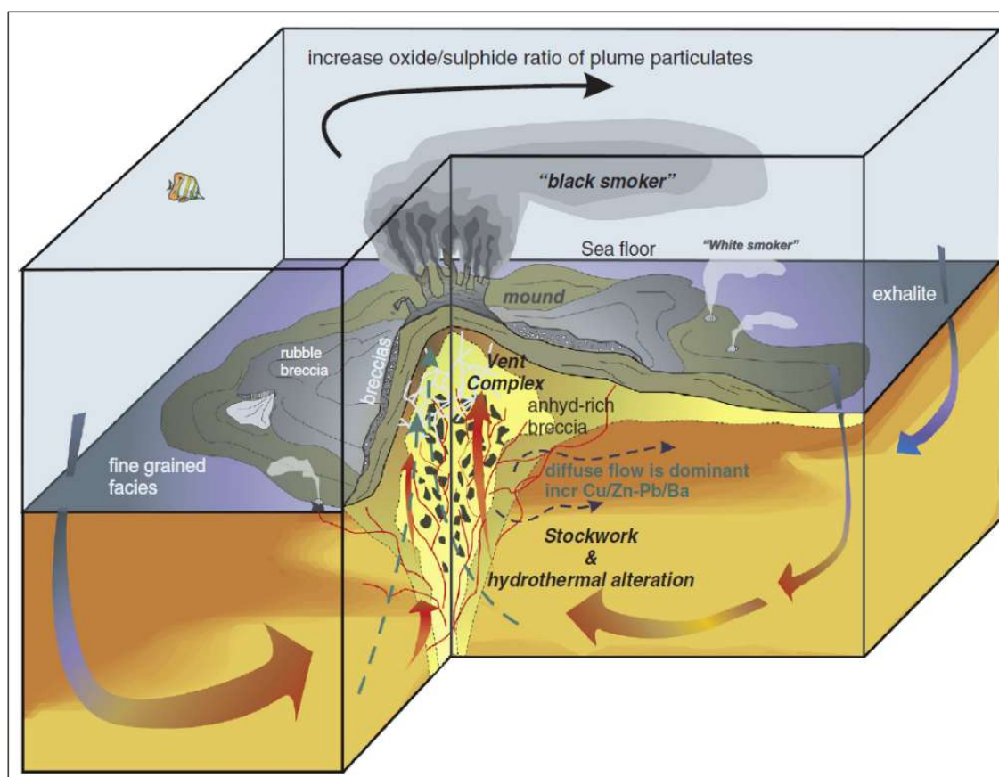
Figure 4-1: Schematic diagram of a "classic" VHMS deposit, with concordant semi-massive to massive sulfide lens underlain by a discordant stockwork vein system and pipe of alteration. Source: from Tornos et al. (2015) 8
