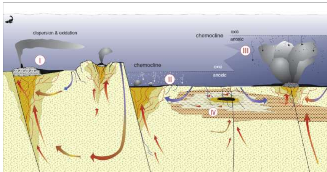
Figure 4-2: Schematic diagram showing the main features of the different styles of VHMS mineralisation. (I) Mounds and black smoker chimneys in oxic environments; (II) brine pools; (III) mound and stratiform sulfides in regional anoxic environments; (IV) sub-seafloor replacement. Source: Tornos et al. (2015) 9
