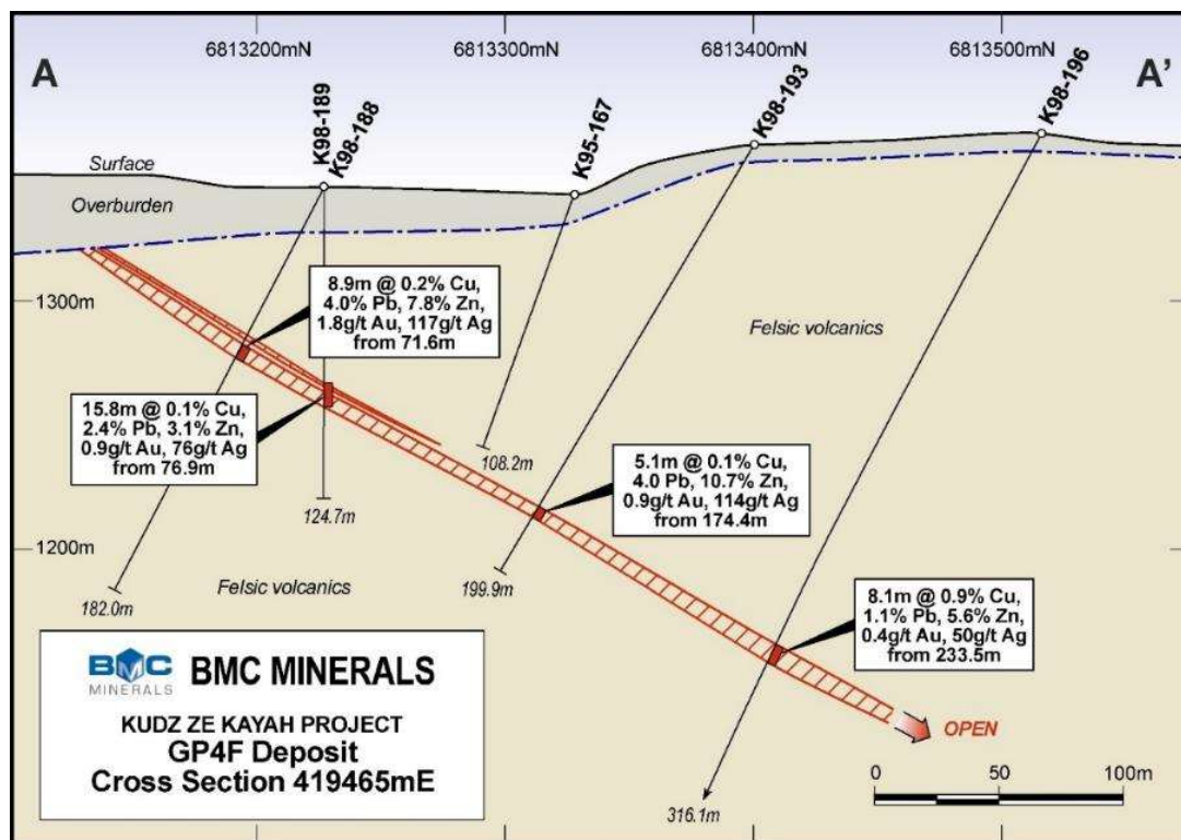
Figure 16-13: Schematic cross-section looking west through the GP4F Zone (419,465 mE) (source: BMC)
