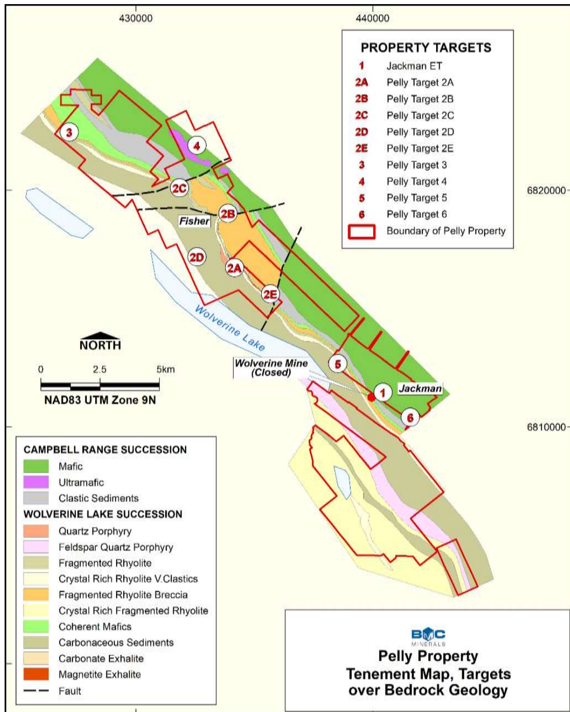
Figure 16-17: Location of prospective targets on the Pelly Property. Source: BMC
