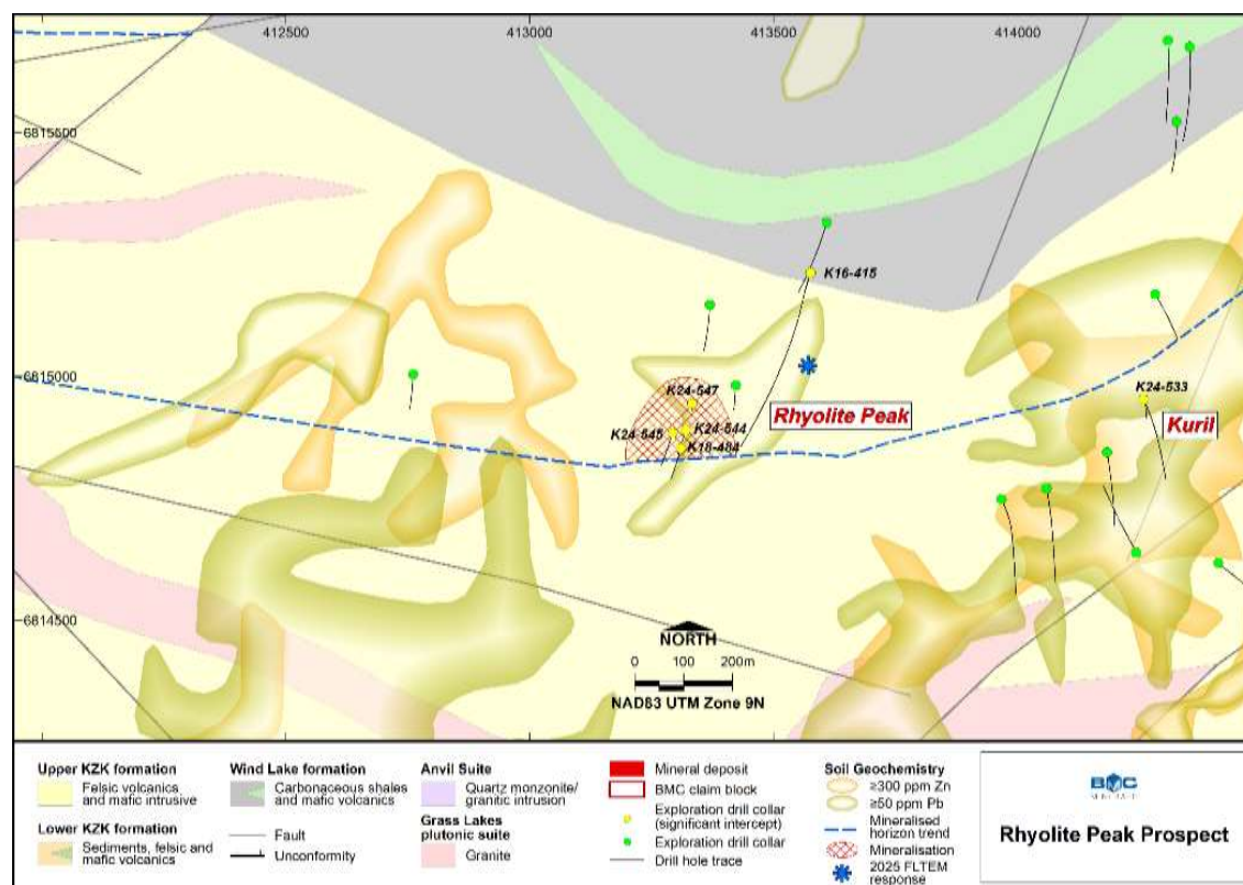
Figure 16-12: Map of the Rhyolite Peak Prospect and exploration drillholes with material intercepts. Source: BMC
