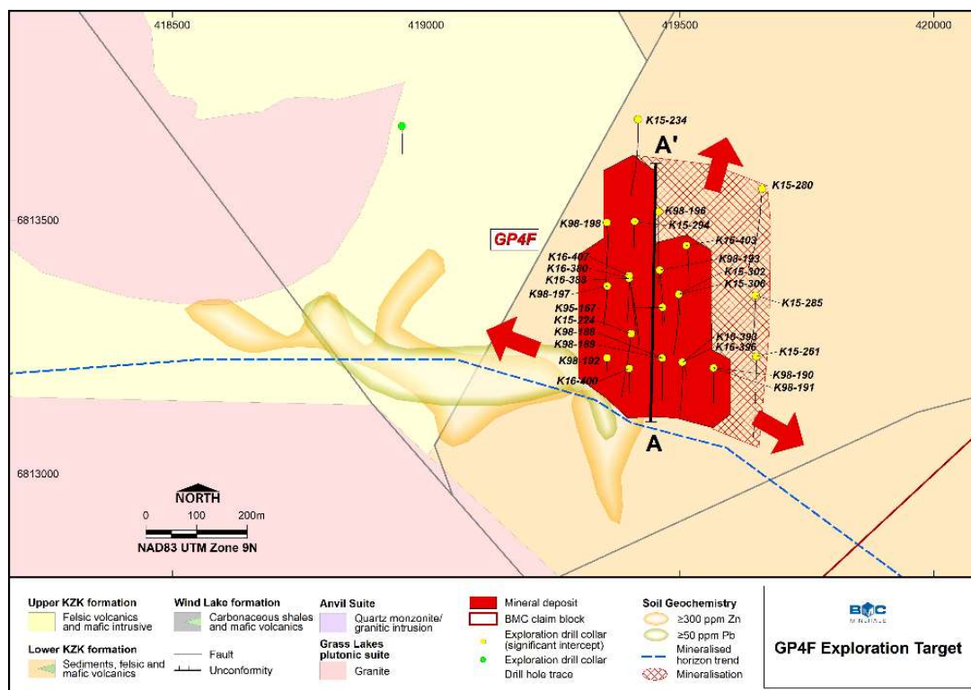
Figure 16-14: Map of the GP4F Prospect and exploration drillholes with material intercepts (source: BMC) (see Appendix E for results).
