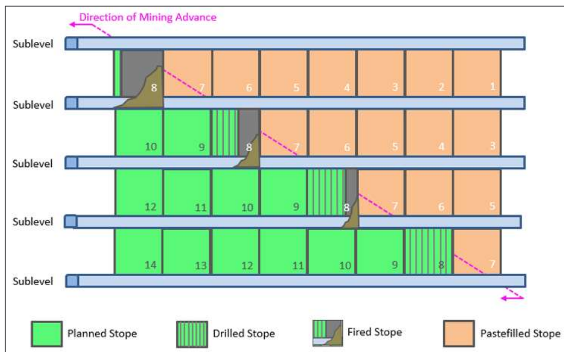
Figure 9-8: Stopping Sequence Schematic. Source: BMC
