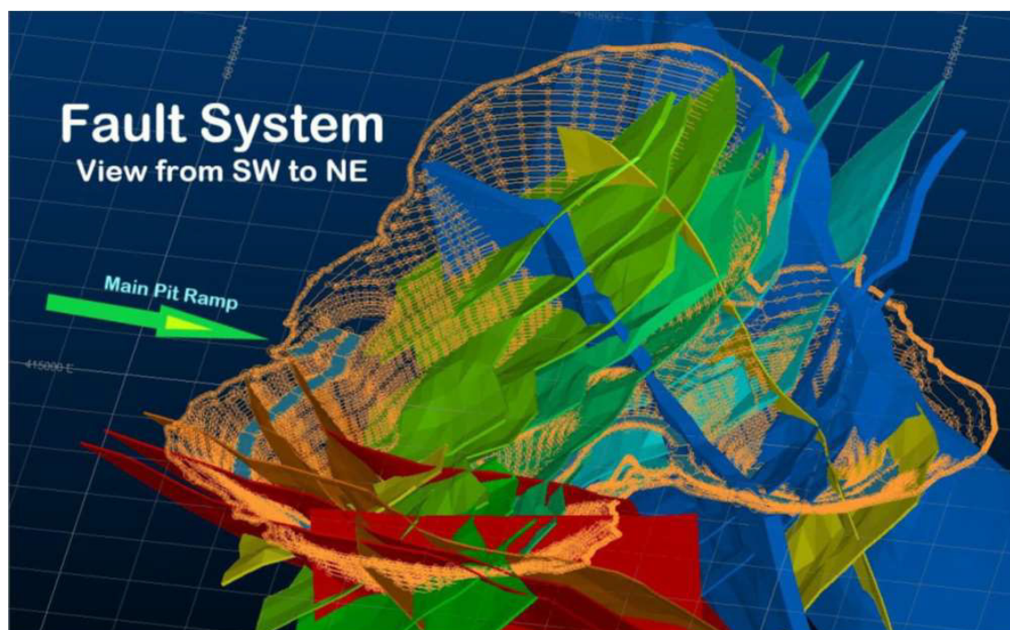
Figure 9-4: Isometric View of the Open Pit Design and Interpreted Faults Source: BMC
