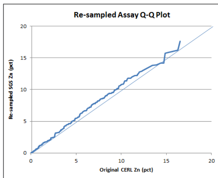
Figure 7-3: Q-Q plot for historical and 2015 data for Zn. Source: CSA Global
