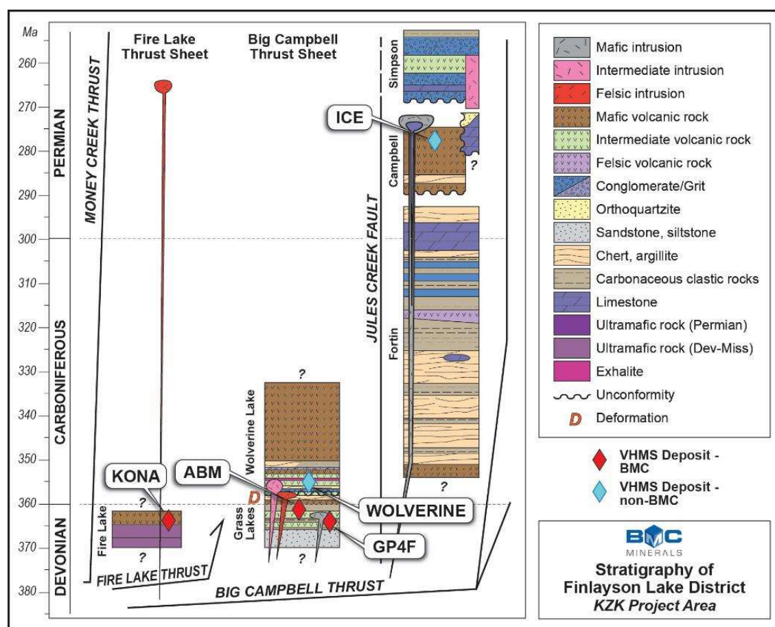
Figure 5-3: Stratigraphy of the Finlayson Lake District, showing location of VHMS deposits Source: BMC
