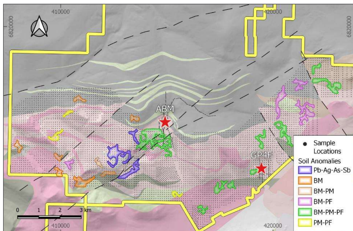
Figure 16-8: Soil geochemistry samples from the Kudz Ze Kayah Property and discrete multi-point anomalies Soil anomalies are divided into several associations: Base metal (BM: Cu, Pb and Zn), precious metals (PM; Au and Ag), and pathfinder elements (PF; As, Bi, Sb, Sn, Tl and W).
