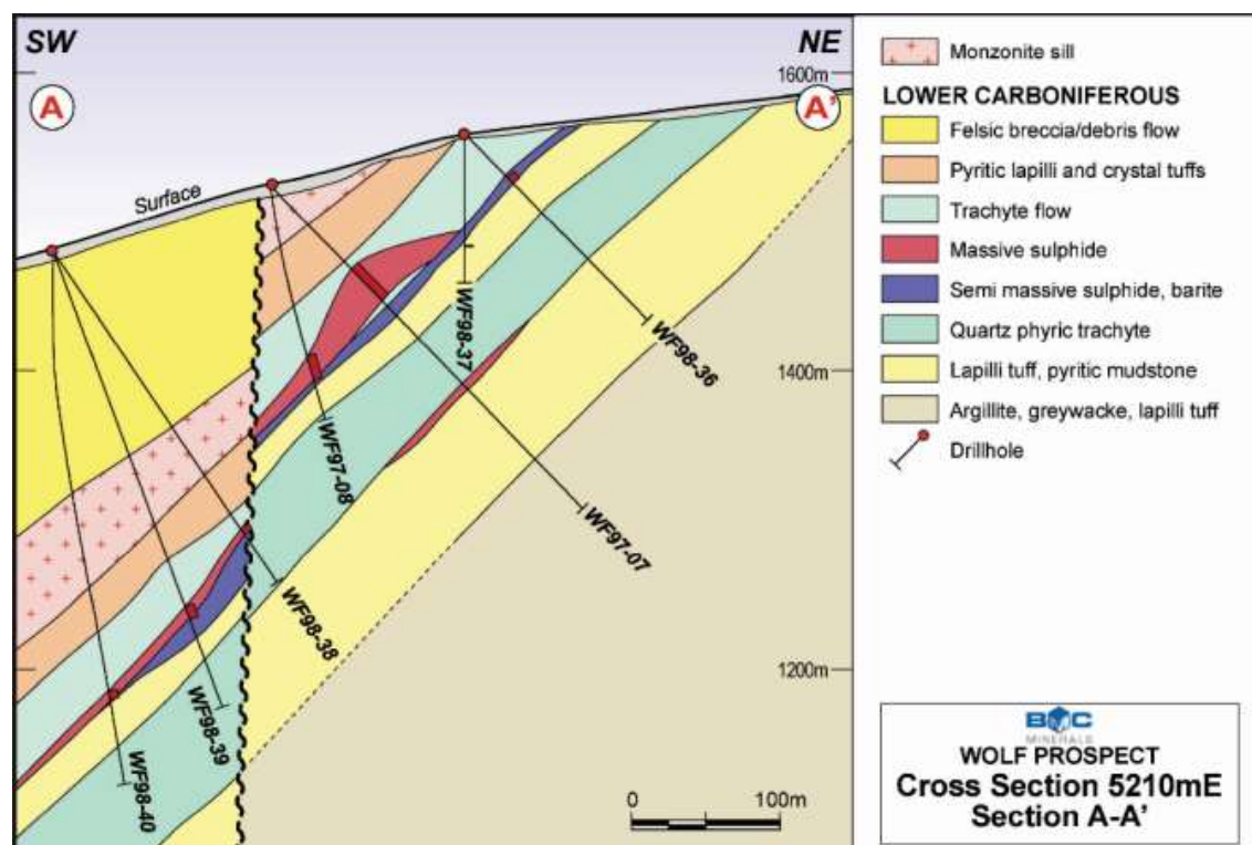
Figure 16-20: Cross-section A-A' (refer Figure 16-21) through the Wolf Deposit. Source: BMC
