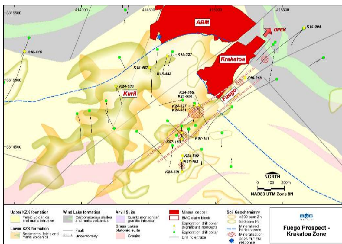
Figure 16-11: Map of the Fuego and Kuril prospects and exploration drillholes with material intercepts.
