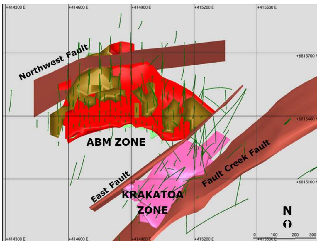
Figure 7-5: Plan view of the ABM and Krakatoa Zone mineralisation wireframes and drill hole traces
