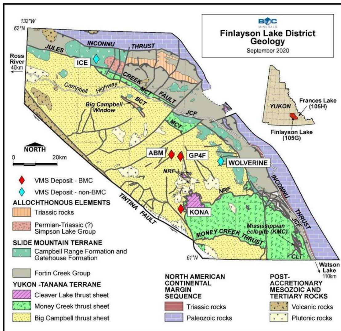
Figure 5-2: Geological map of the Finlayson Lake District Source: BMC
