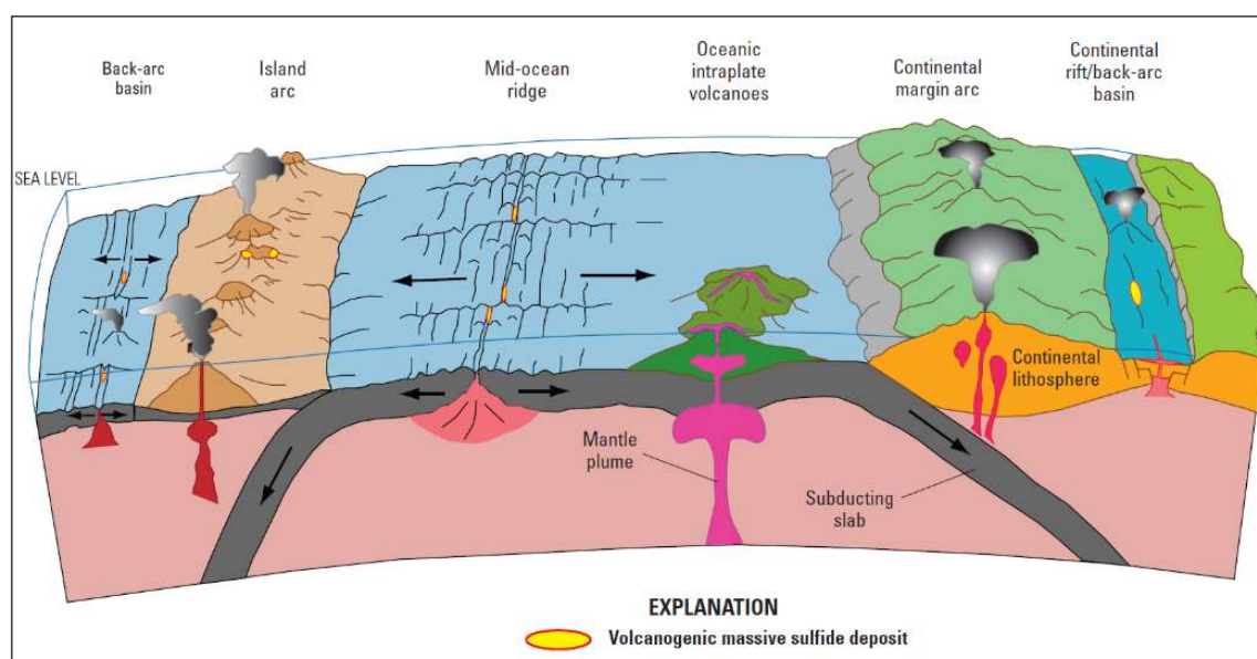
Figure 4-3: Schematic diagram showing volcanogenic massive sulfide deposits in divergent (mid-ocean ridge and back-arc basin) and convergent (subduction related island arc and continental margin arc) plate tectonic settings. Source: Shanks and Thurston (2012) 10
