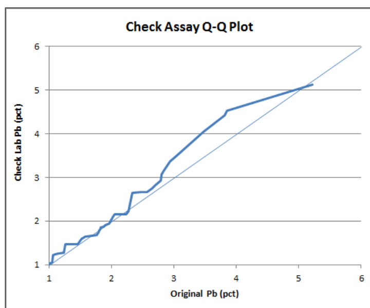
Figure 7-1: Q-Q plot using each data pair as a quantile and showing different distributions for Pb data from ALS check data and original SGS data
