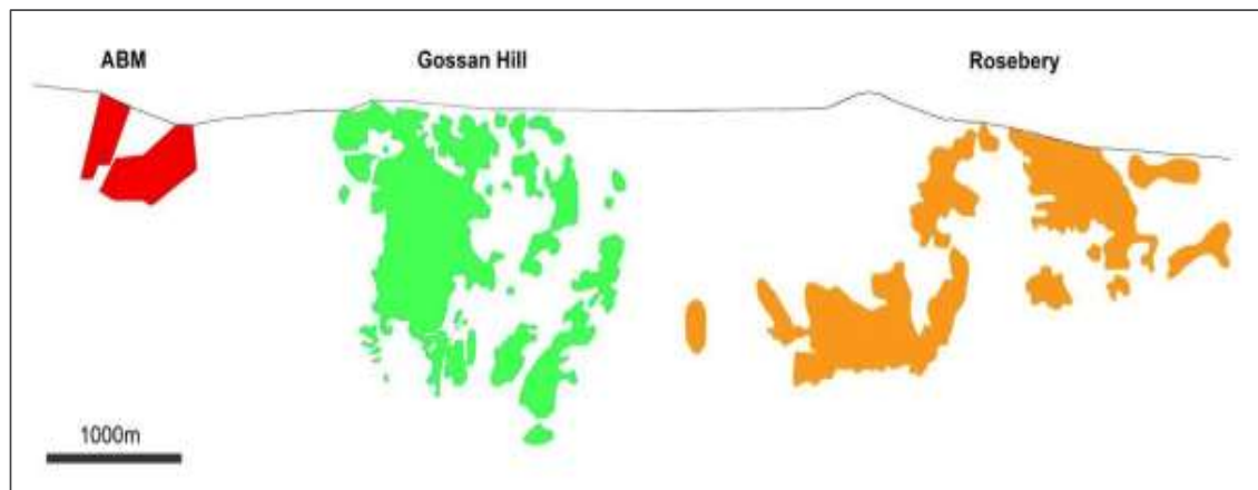
Figure 16-23: Schematic long section projections of the ABM Deposit outline in comparison to schematic projections of the multi-lens Gossan Hill and Rosebery VHMS deposit outlines projected to a common vertical plane and scale. Note ABM Deposit is shallowly dipping and has only been drilled to around 200 m vertical depth so far. Source: BMC and company annual reports 16
