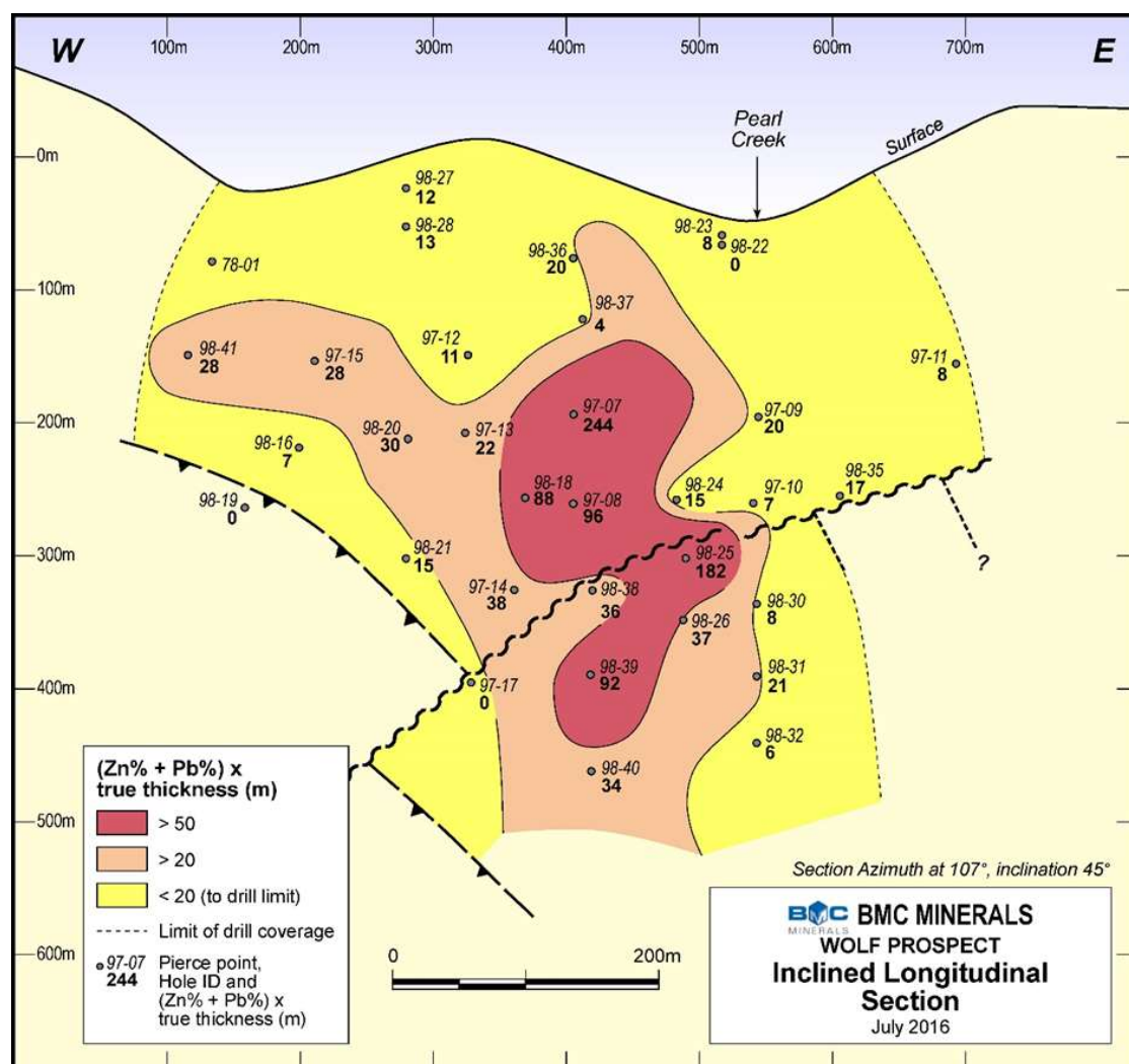
Figure 16-22: Inclined longitudinal section showing drill pierce points and high-grade "keel" to the Wolf Deposit Source: BMC
