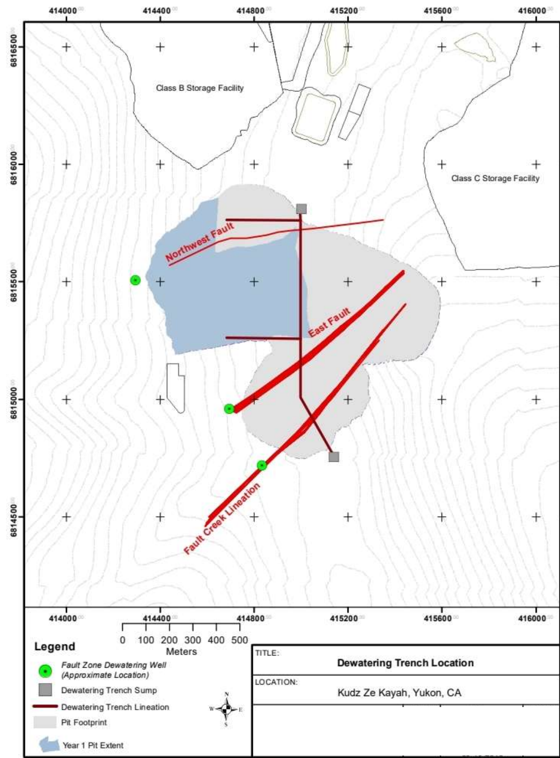
Figure 8-2: Proposed dewatering trench locations Source: BMC
