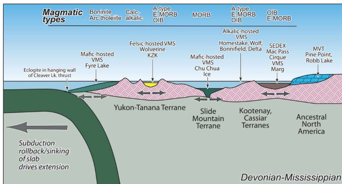
Figure 5-4: Interpreted Tectonic Setting of the Mineral Deposits Source: Nelson and Colpron (2007) 12
