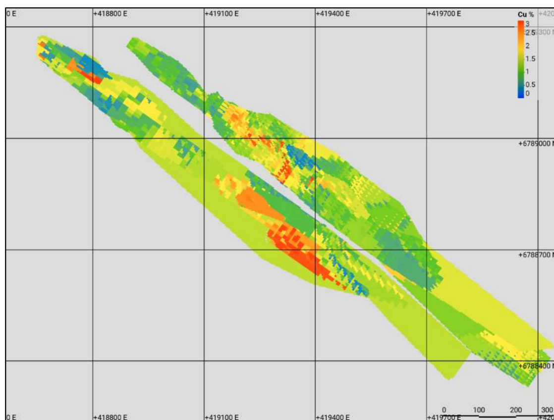
Figure 7-14: Kona block model showing Cu grades (%) (plan view) no cut-off grade applied. Source: Cube
