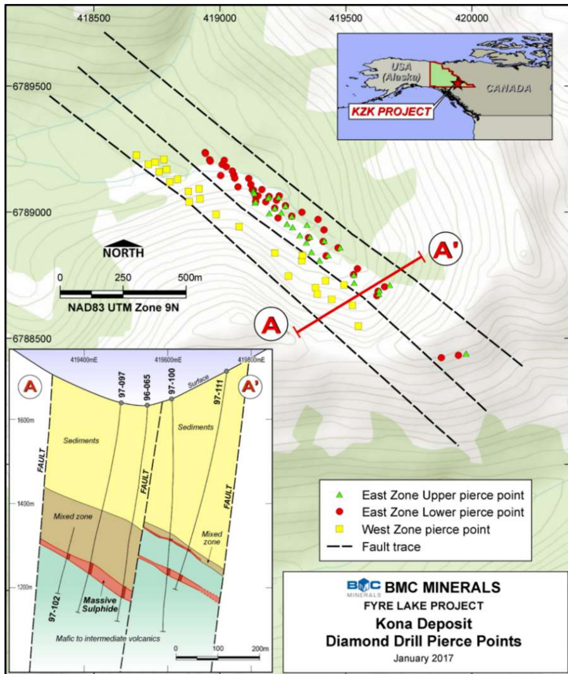
Figure 7-11: Plan and Cross-Section View of the Kona Deposit Source: BMC
