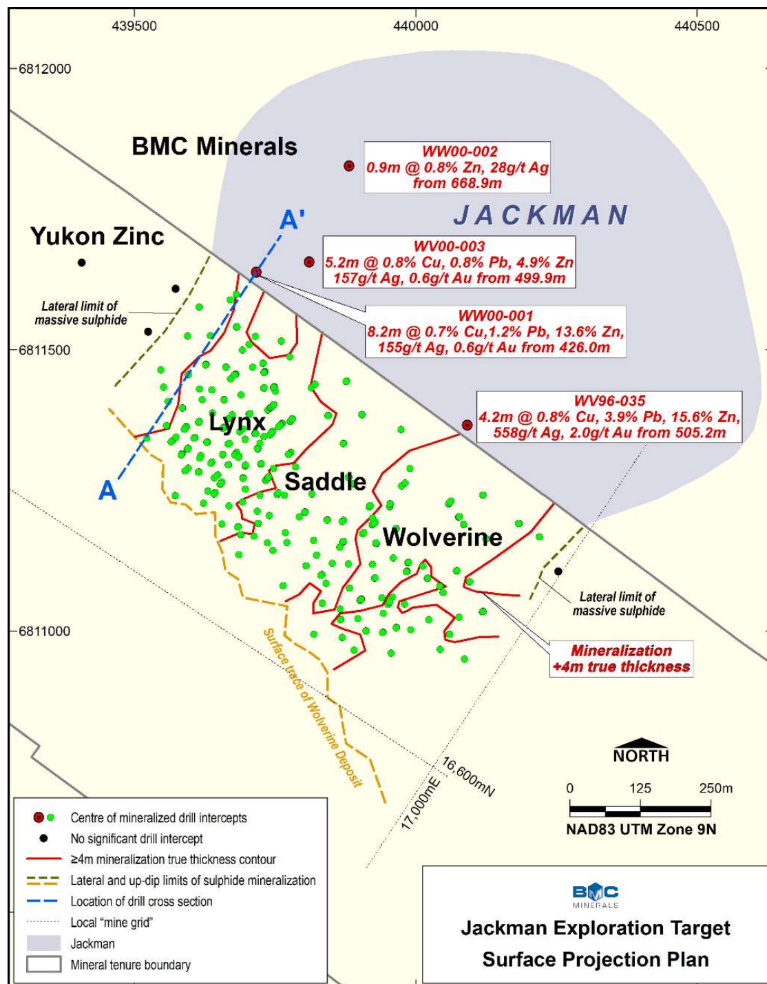
Figure 16-18: Plan view of the Jackman exploration target. Source: BMC
