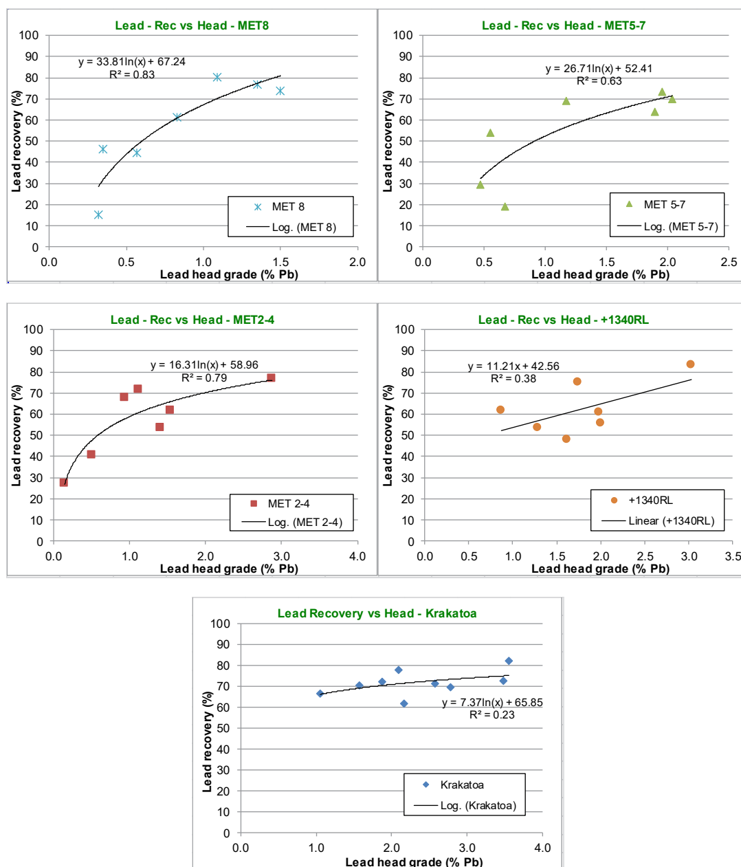
Figure 10-2: Lead head grade vs recovery
