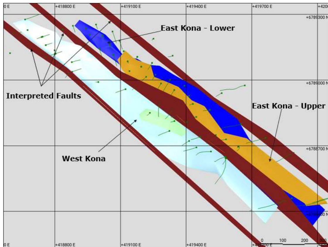
Figure 7-13: Plan view of Kona Mineralisation Wireframes and Interpreted Faults.
