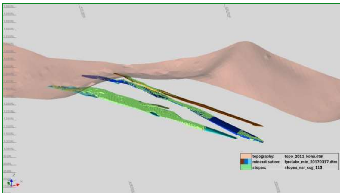
Figure 7-15: Oblique view of the interpreted Kona mineralisation - View Looking NE – Slope Outlines (pale green) over Mineralised Lodes generated for C$113/t cut-off. Source: Cube
