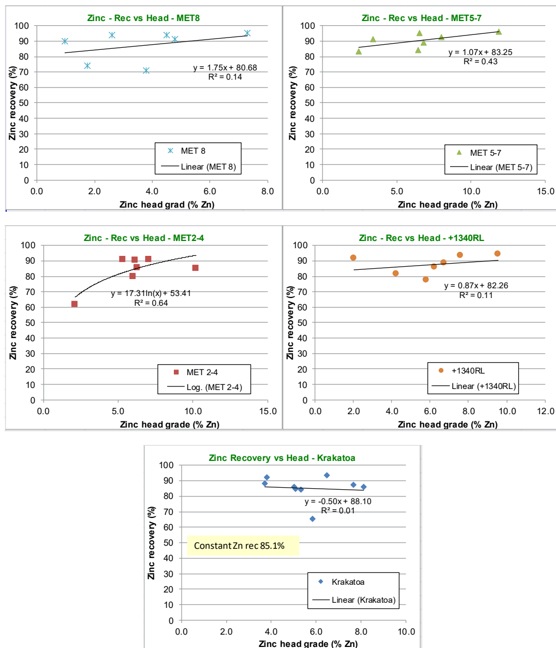
Figure 10-3: Zinc head grade vs recovery source: 2025 Technical Report
