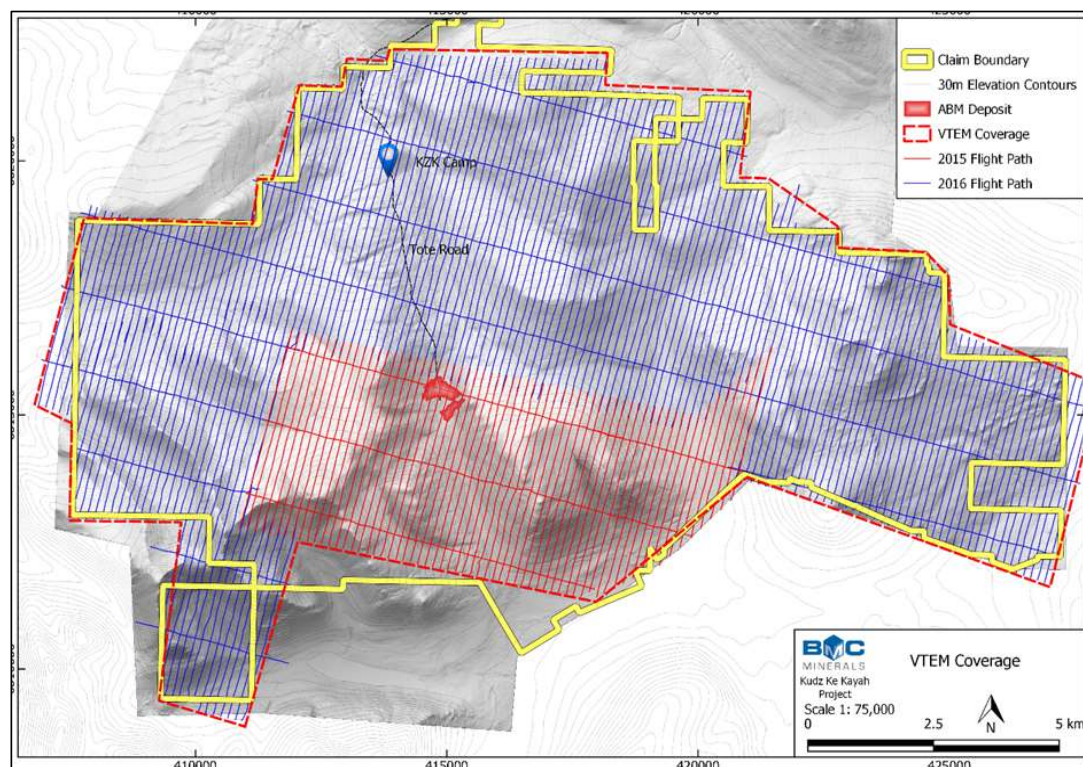
Figure 16-2: VTEM™ coverage Source: BMC
