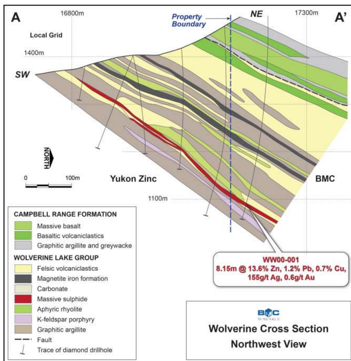
Figure 16-19: Cross Section A-A' through the Wolverine Deposit and the Jackman exploration target Source: BMC
