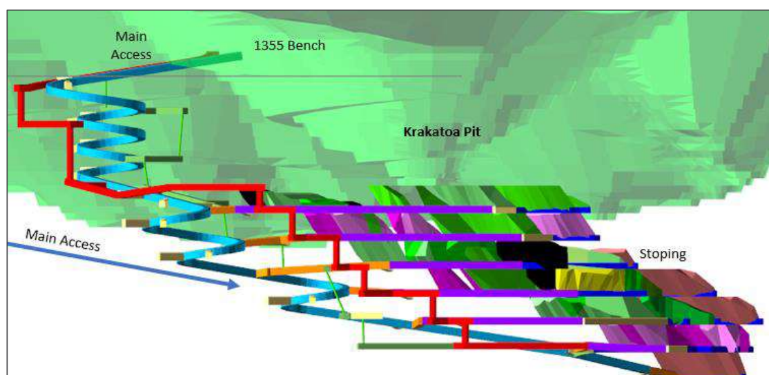
Figure 9-6: Diagrammatic isometric long section of the Krakatoa underground mine, looking west. Source: BMC
