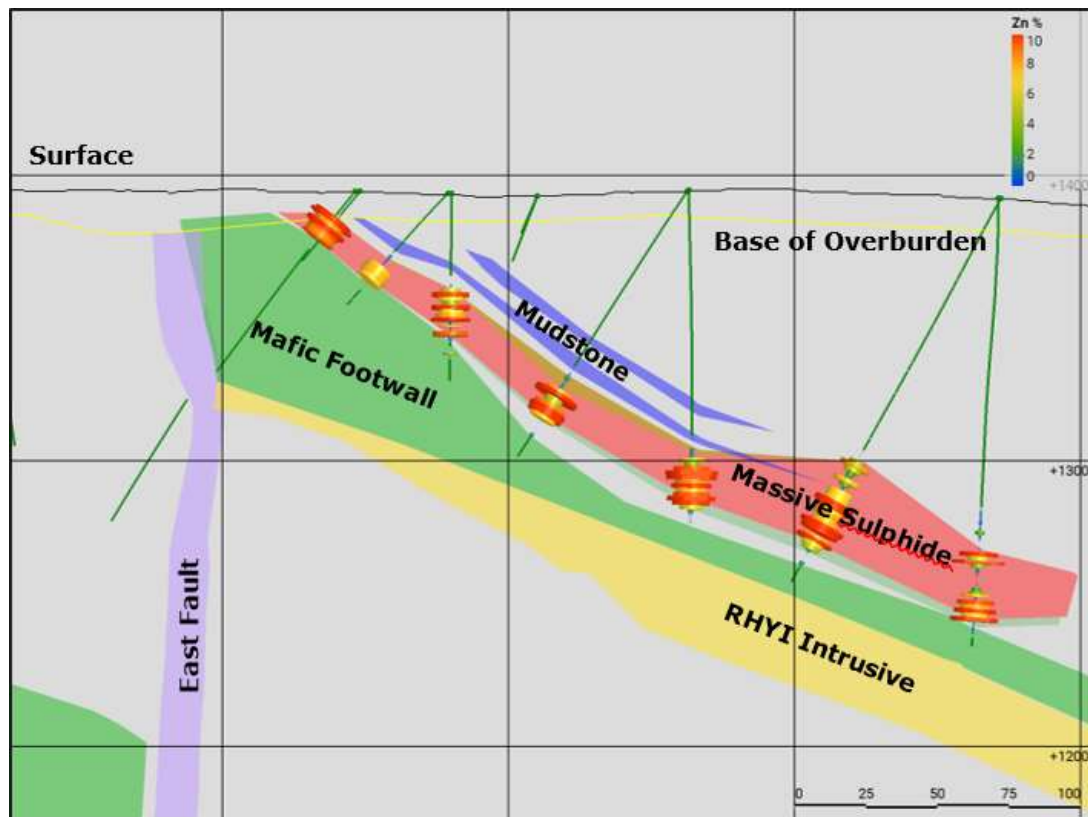
Figure 7-4: ABM geology interpretation (Section 415,100 mE looking west)
