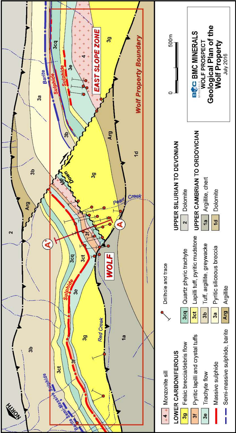
Figure 16-21: Geological plan of the Wolf Property. Source: BMC
