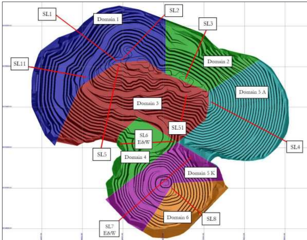
Figure 9-2: Geotechnical slope zones for ABM and Krakatoa pits Source: BMC
