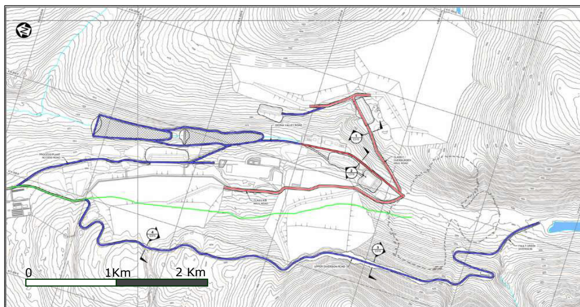
Figure 12-2: Proposed site road network; Green indicates road upgrade, blue indicates new light vehicle road, red indicates mine haul road.
