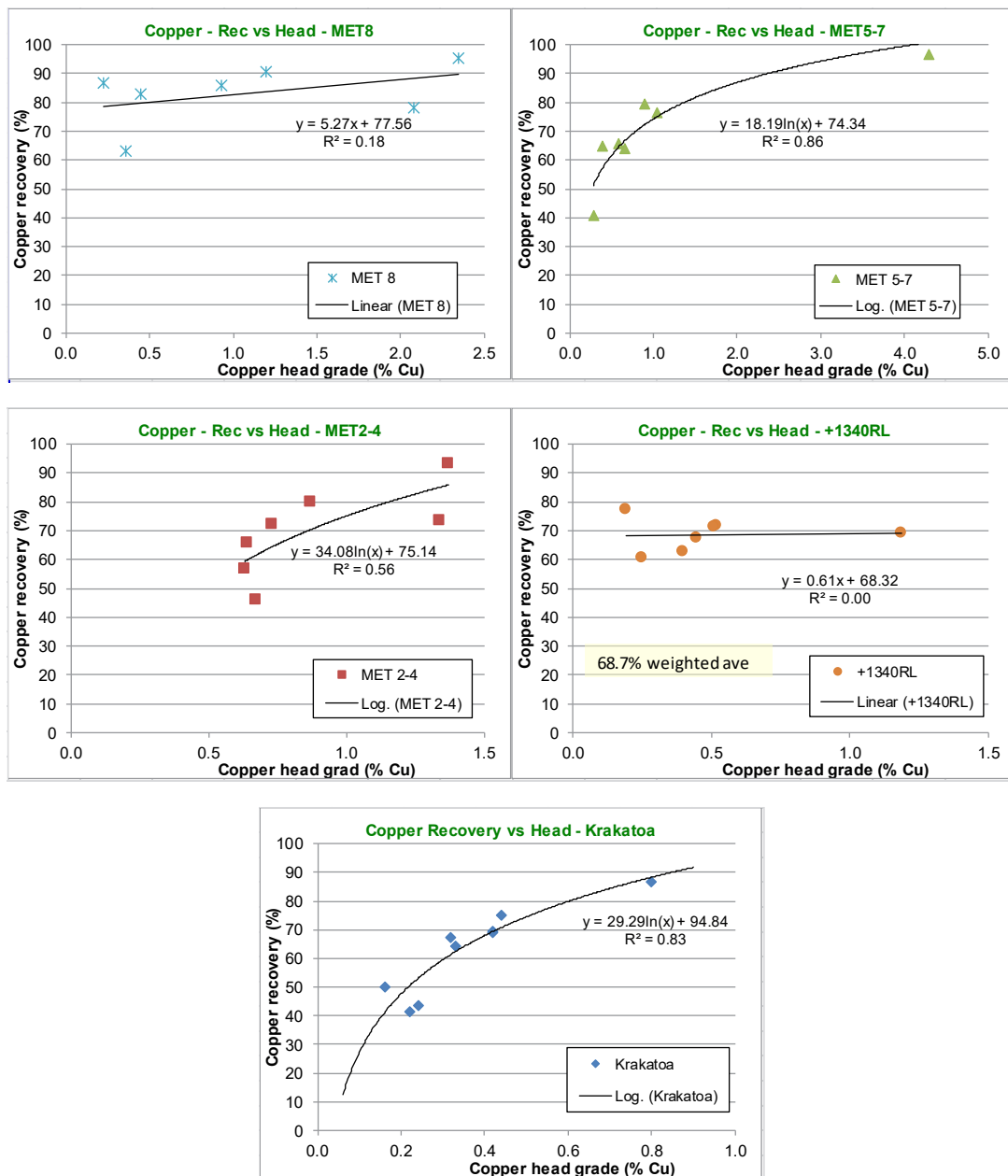
Figure 10-1: Copper head grade vs recovery (source: 2025 Technical Report)
