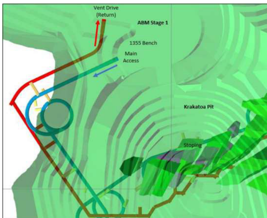
Figure 9-7: Krakatoa – Diagrammatic sketch of main access and ventilation ramp (plan view).
