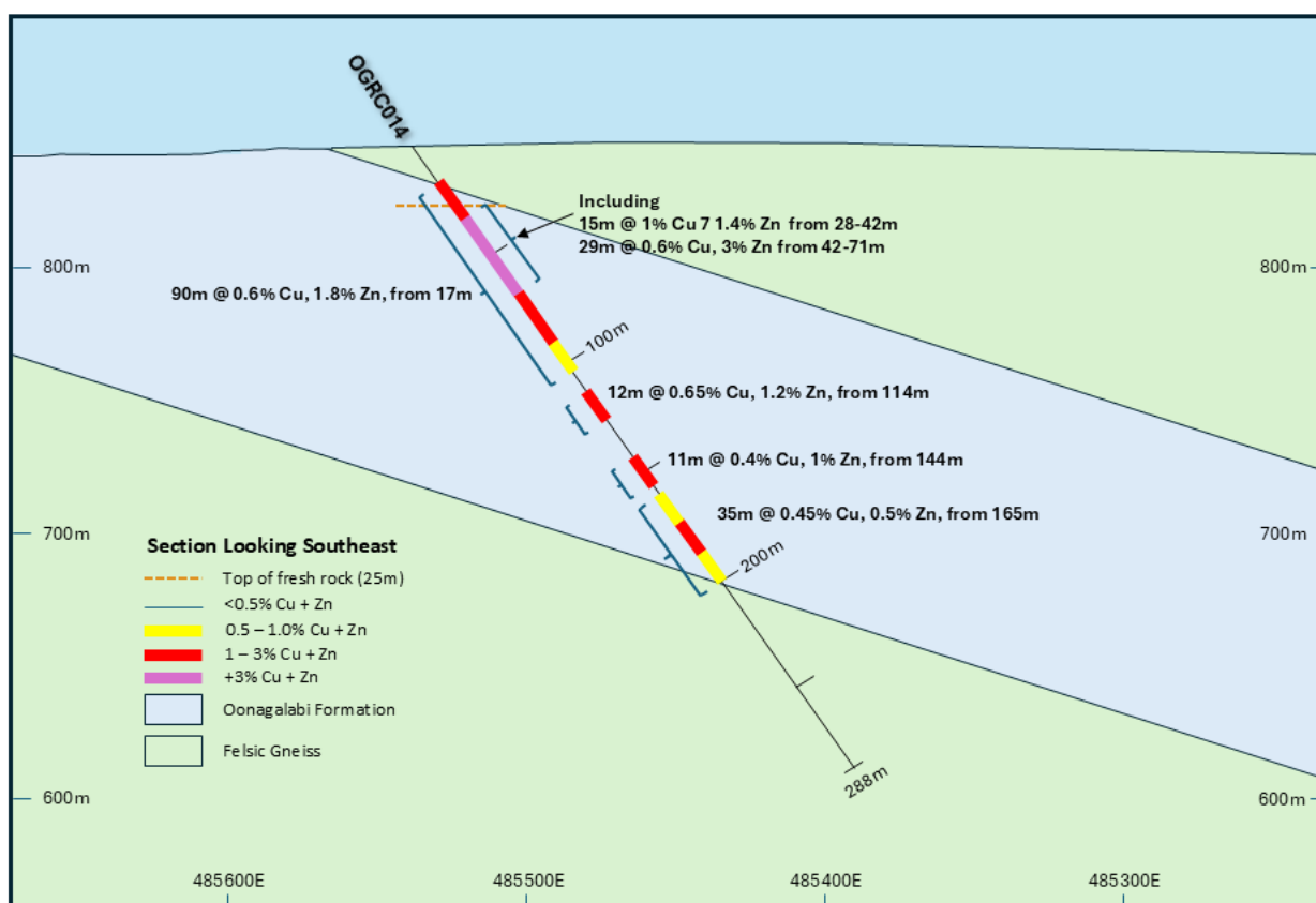
Figure 1 – Simple view of geology with cross section of OGRC014.
