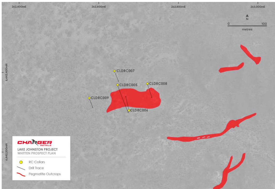
Figure 2. Plan of the Whitten LCT pegmatite and the recent RC drill holes areas within the Lake Johnston Lithium Project.
